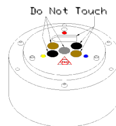
Detector Module "puck" Figure 2-4
