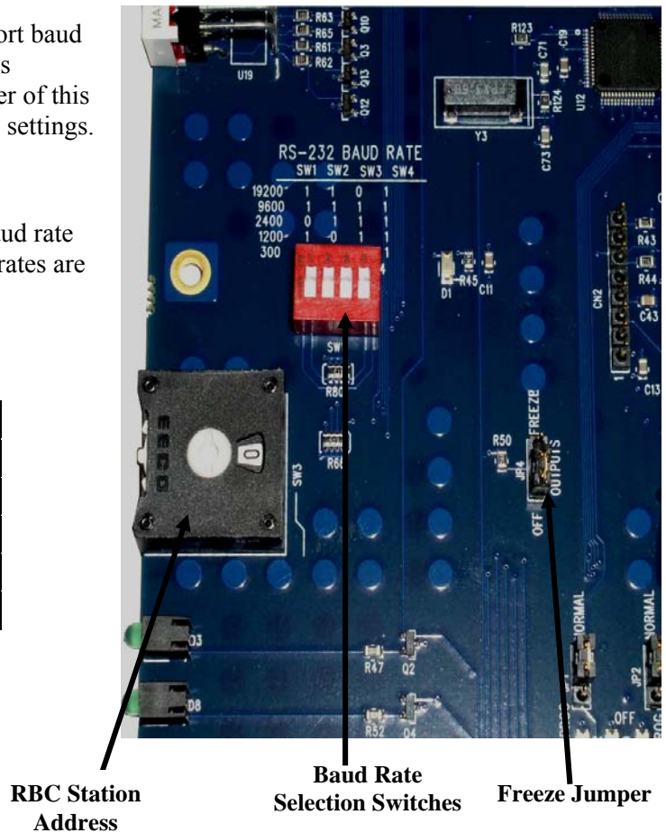
Figure 2. Switch Locations
