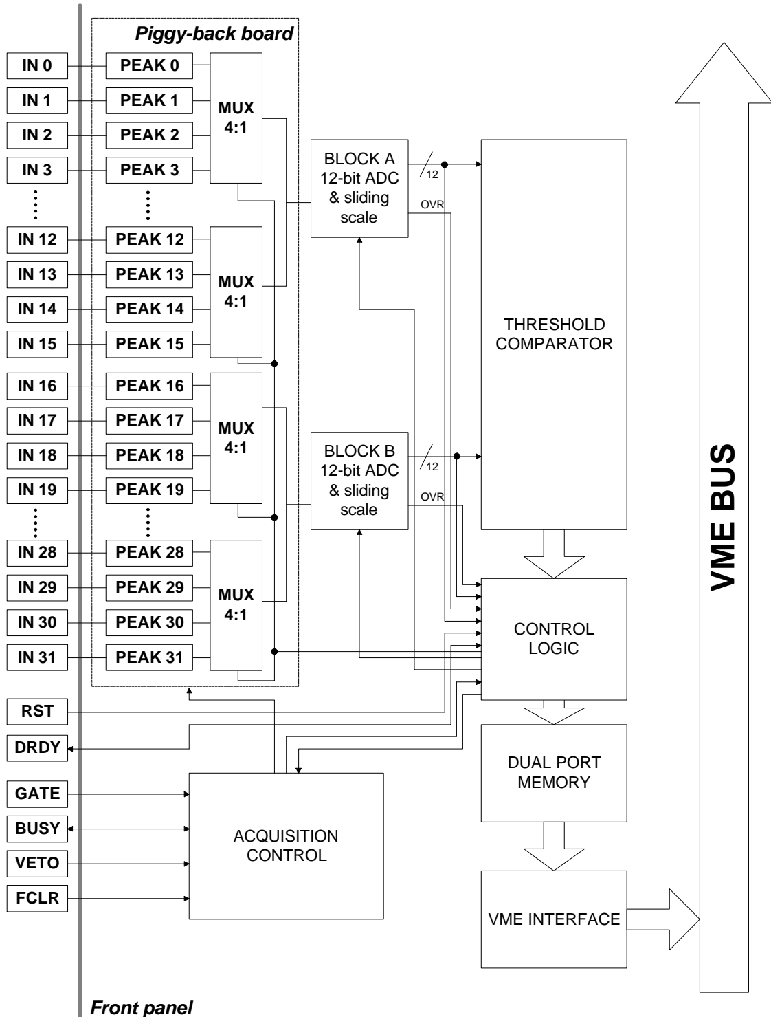
Fig. 1.1: Model V785 Block Diagram
