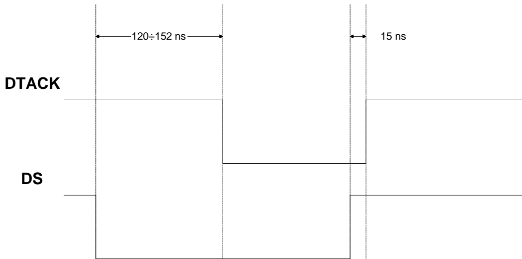
Fig.A.3: VME cycle timing in MBLT/CBLT64 mode
