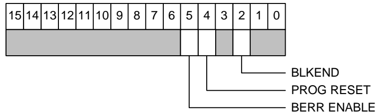
Fig. 4.17: Control Register 1
