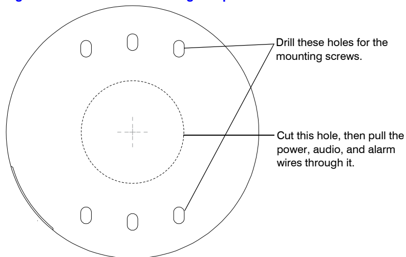
Figure 2-2 Surface Mounting Template
