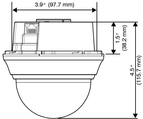
Figure C-3 HD3MDIH/X Camera Side View Dimensions with Adapter Plate
