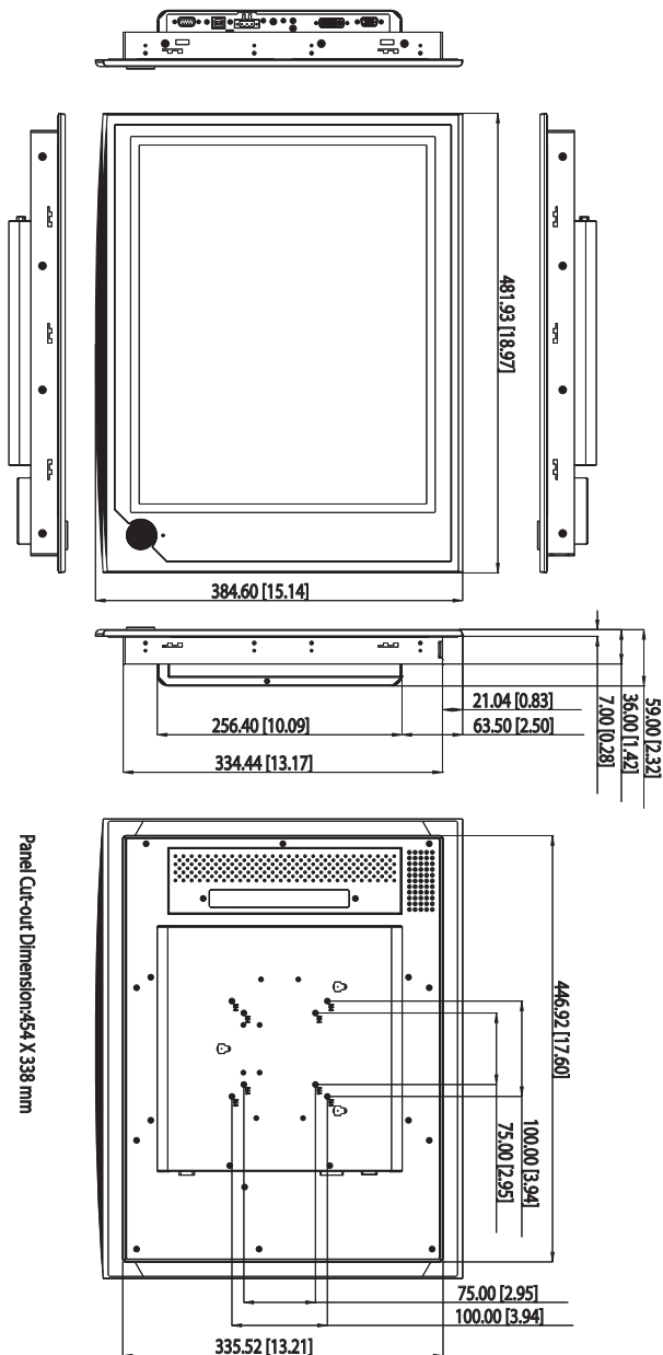
Figure 1.1: FPM-5191G Dimensions
