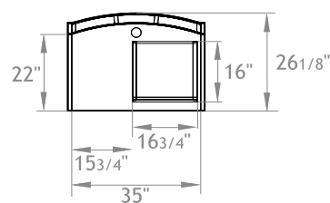
Overhead view of lectern
