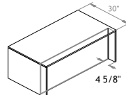
30" depth: 4-5/8" standard recess
