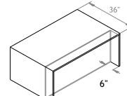
36" depth: 6" standard recess
