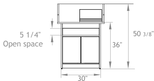
Front view of lectern
