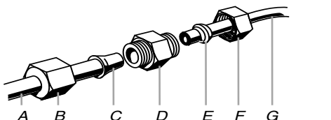
A. Refrigerator water tubing B. Nut (provided) C. Bulb D. Coupling (purchased) E. Ferrule (purchased) F. Nut (purchased) G. Household water line
