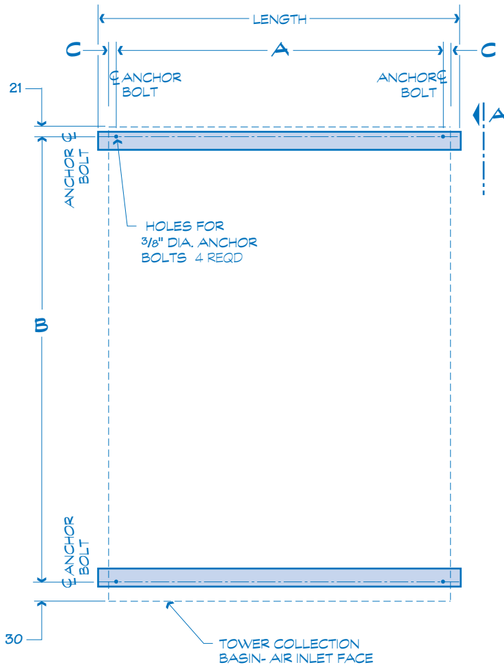
SUPPORTING STEEL SINGLE CELL
