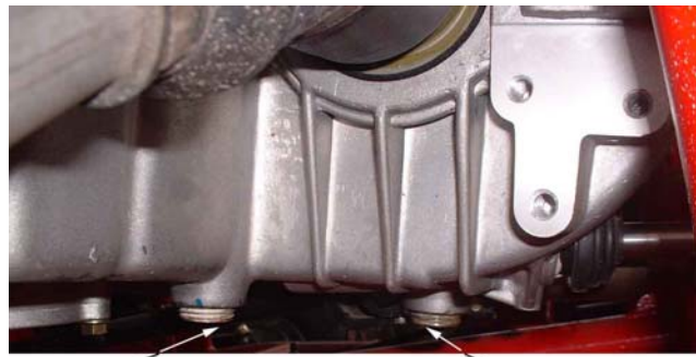
outlet of iron dust oil transmission outlet
