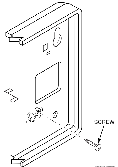
Figure 2: Tamper Protection
