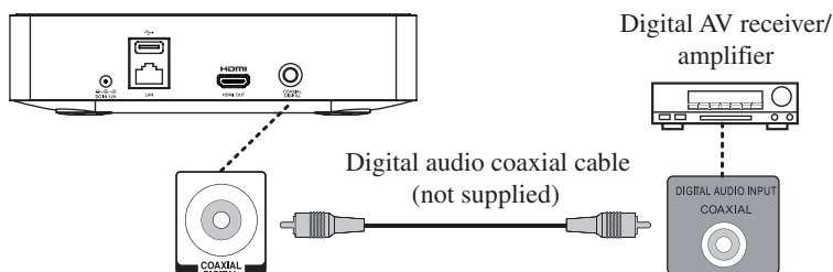
(Sample Illustration) Connecting to a digital AV receiver/amplifier
