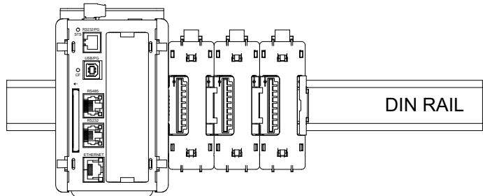
Figure 4 - Installation Complete
