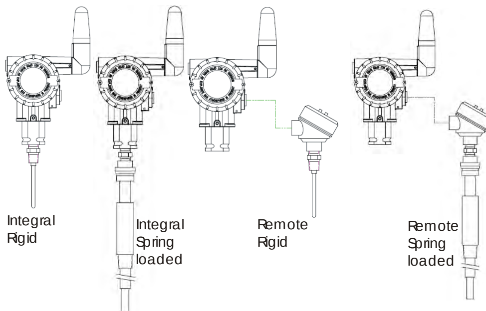
Figure 3-4 Temperature probes
