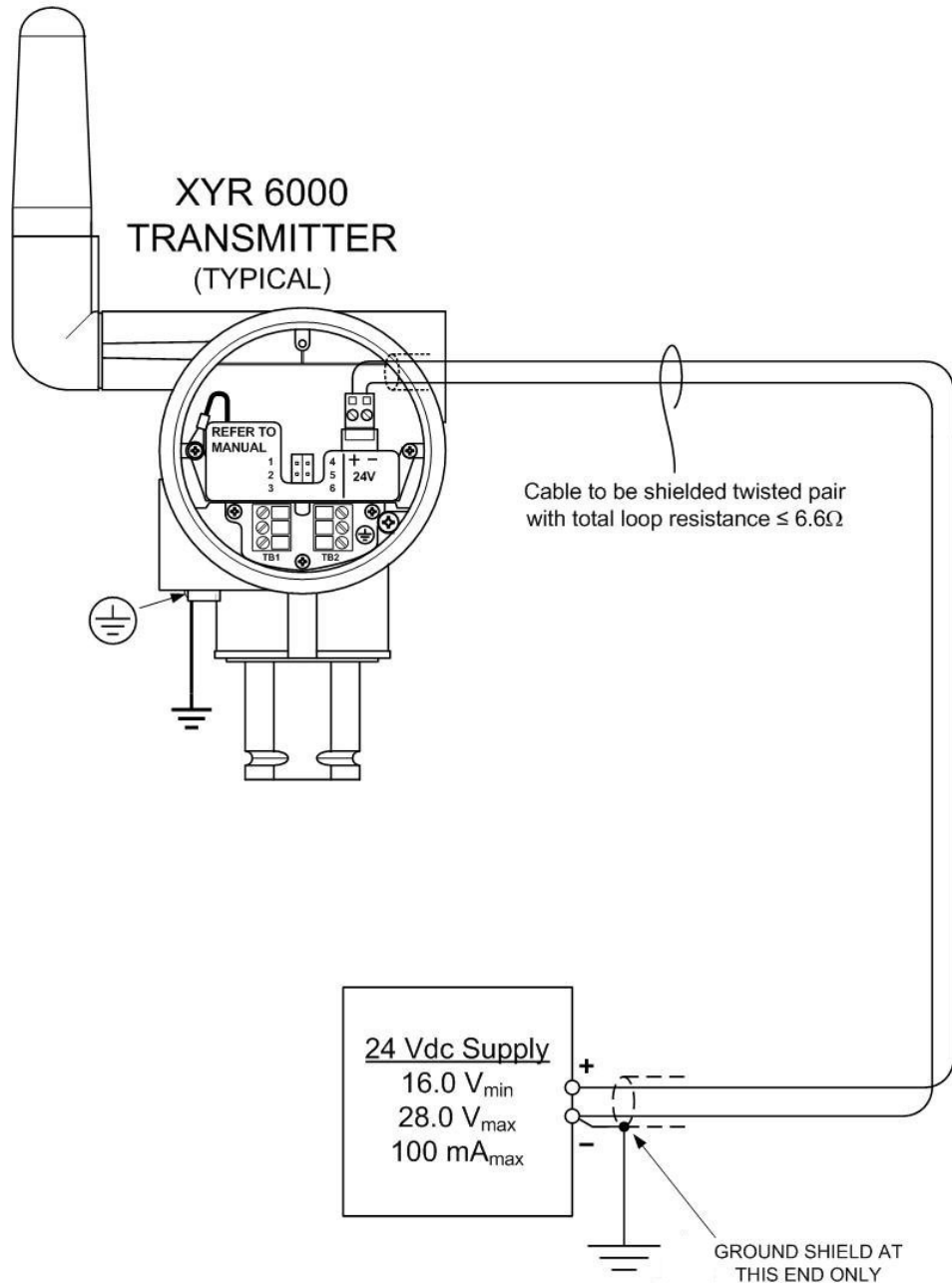
Figure 5-5 Power Supply 24 Vdc Option (DC) System Diagram
