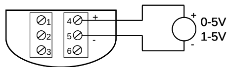
Figure 3-6 Voltage input wiring
