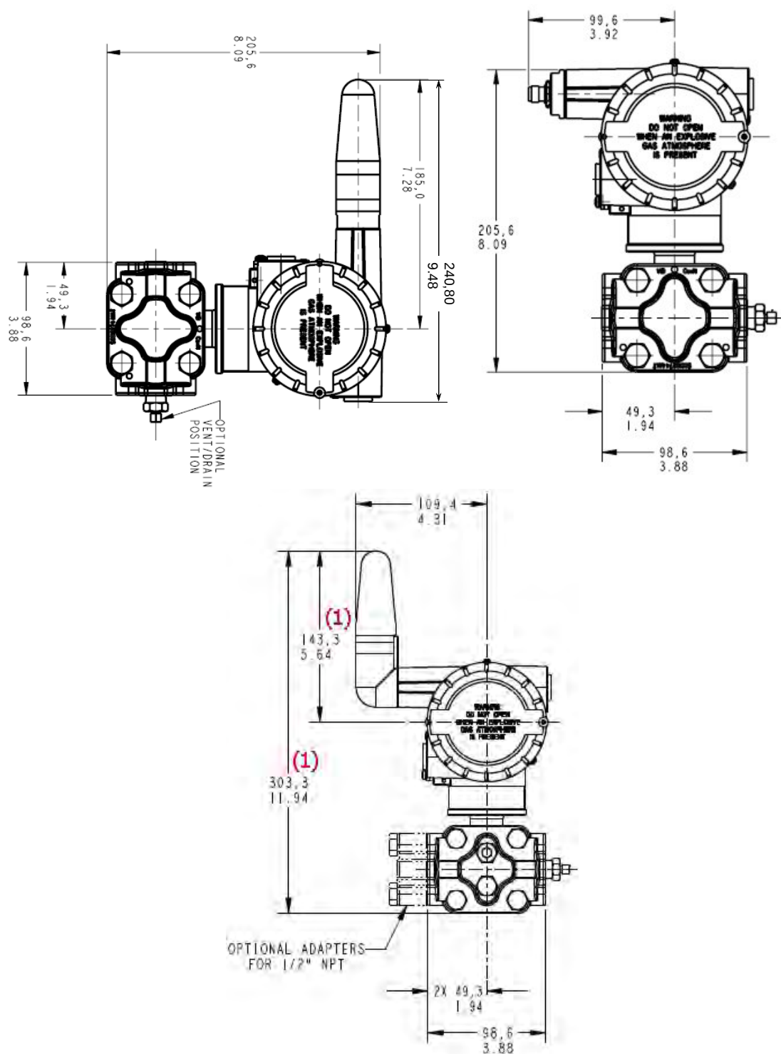
Figure 2-4 DP/DHGP Pressure antenna dimensions
