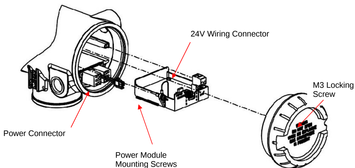
Figure 5-3 Power Option 24V
