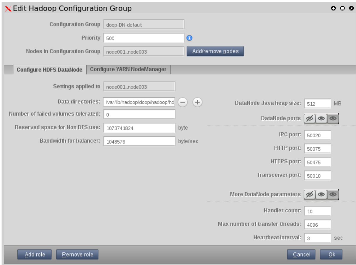
Figure 3.11: Hadoop Configuration Groups Tab, After Opening DataNode Configuration Group: DataNode Role Configuration
