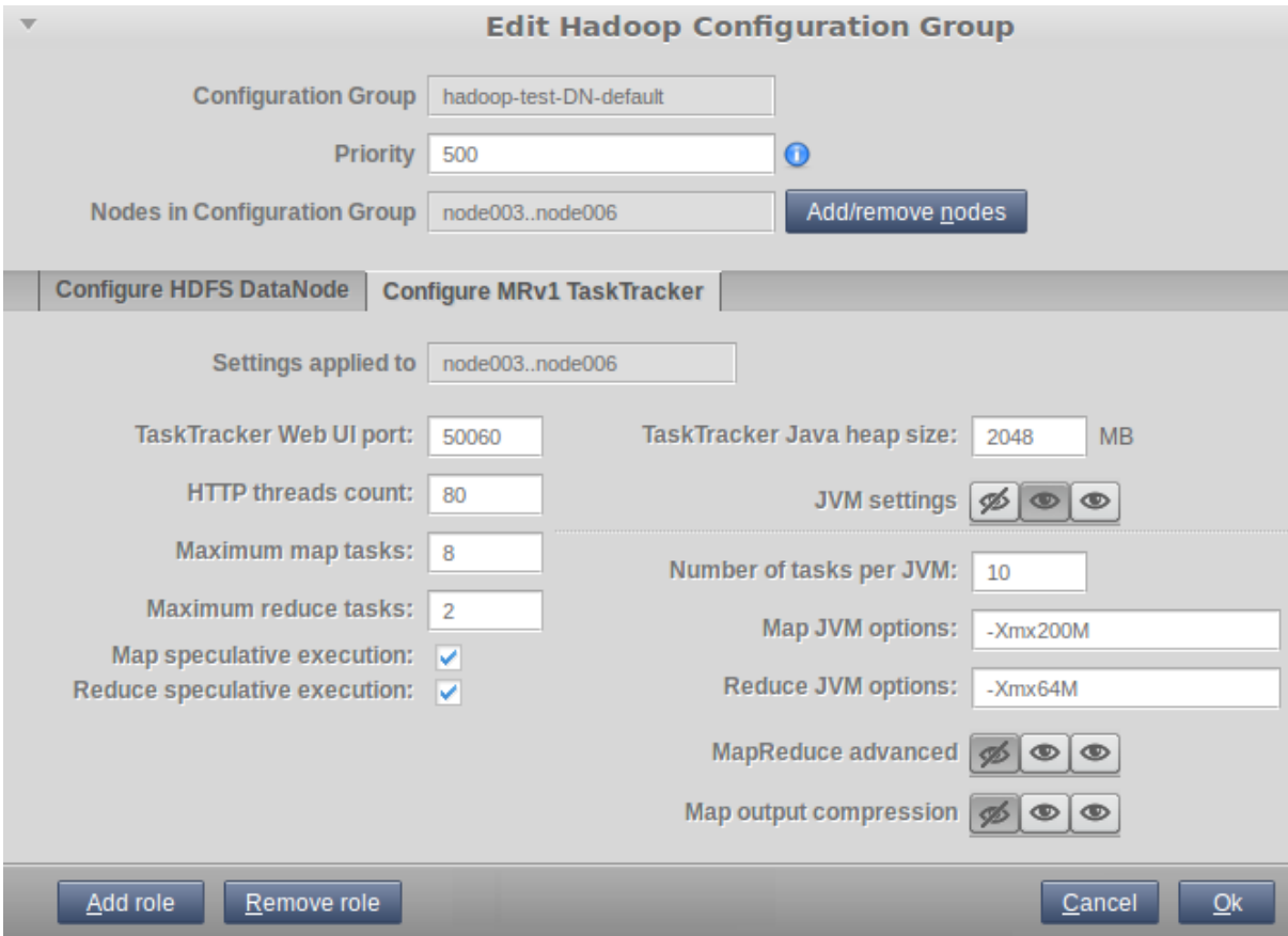
Figure A.2: Hadoop Configuration Group Prior To Cloning
