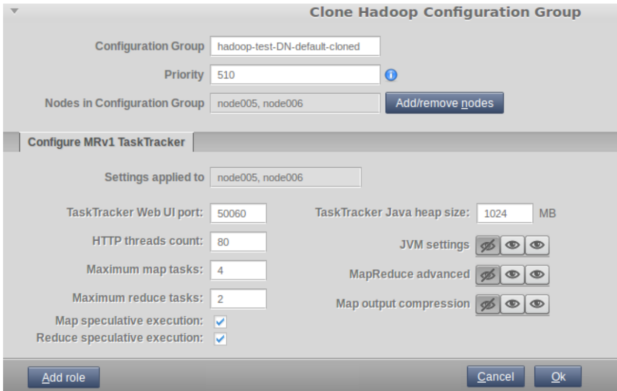
Figure A.3: Example Of Cloned Hadoop Configuration Group
