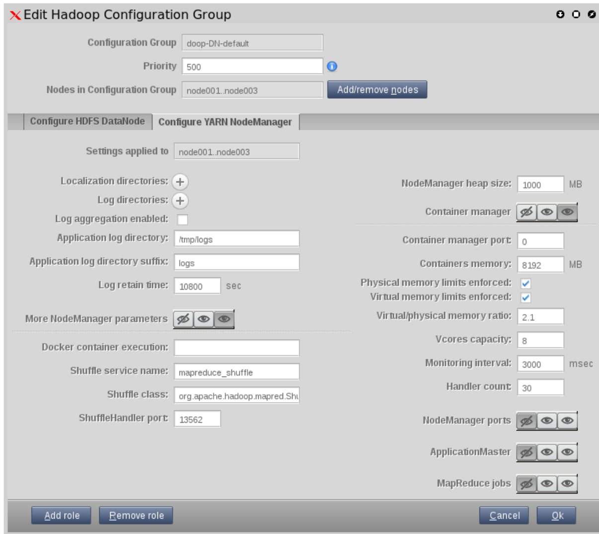
Figure 3.12: Hadoop Configuration Groups Tab, After Opening DataNode Configuration Group: YARN NodeManager Role Configuration
