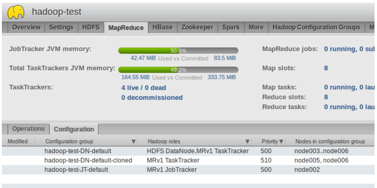
Figure A.4: Hadoop Configuration Groups for MapReduce after example configuration
