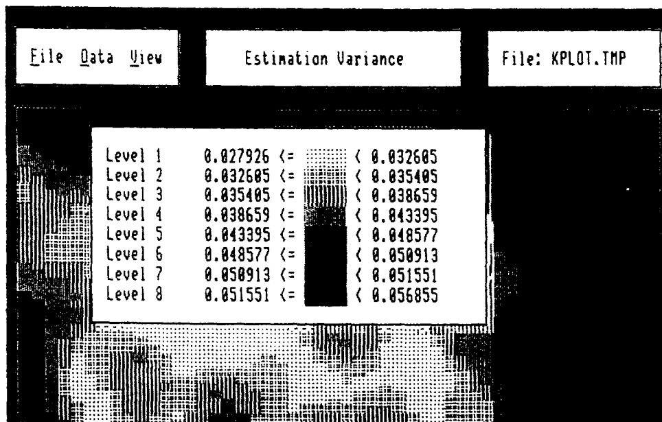
Figure 3.1.5. Contour diagram using the Ordinary [Col]Kriging and Block Contour Diagram programs. In A and B, respectively, the estimated value for the decay rate and the estimation variances are illustrated.
