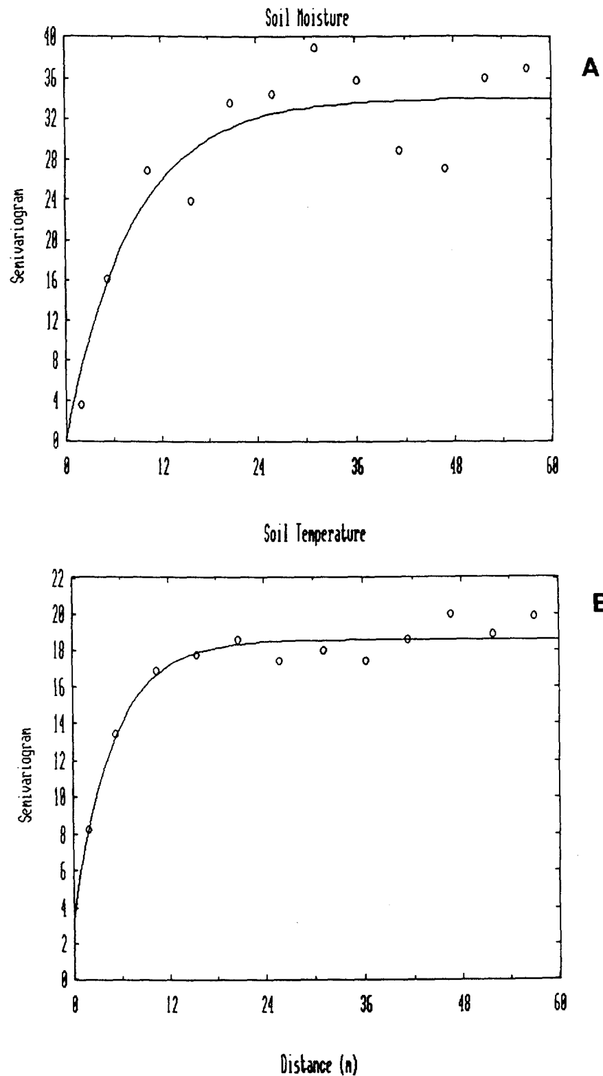
Figure 3.3.1. The semivariogram function for the surface moisture content (in A) and the surface soil temperature (in B) using the Variogram Calculation (Sample) program and the data see, C912.DAT.
