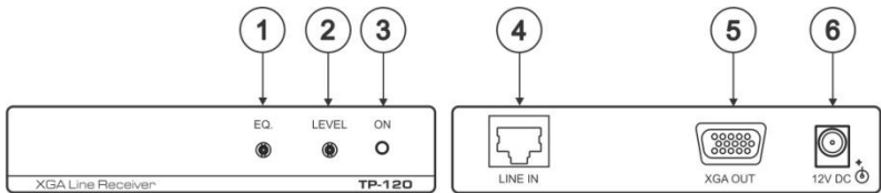
Figure 7: TP-120 XGA Line Receiver
