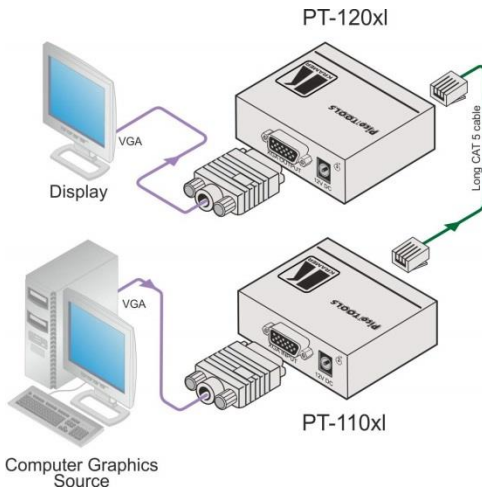
Figure 6: Connecting the PT-110xl to a PT-120xl
