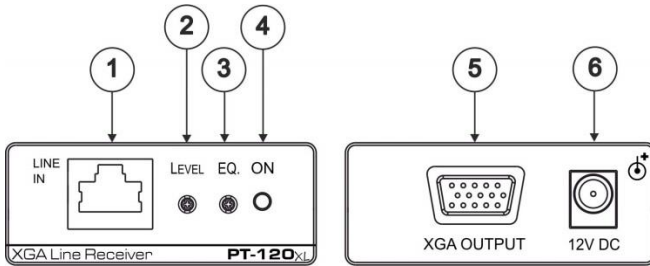
Figure 5: PT-120xl XGA Line Receiver
