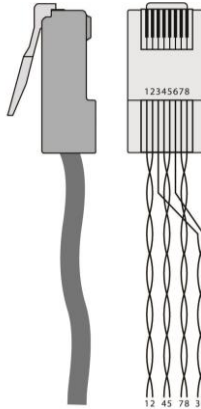
Figure 8: CAT 5 PINOUT
