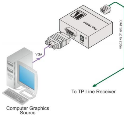
Figure 2: Connecting the PT-110xl UXGA Line Transmitter
