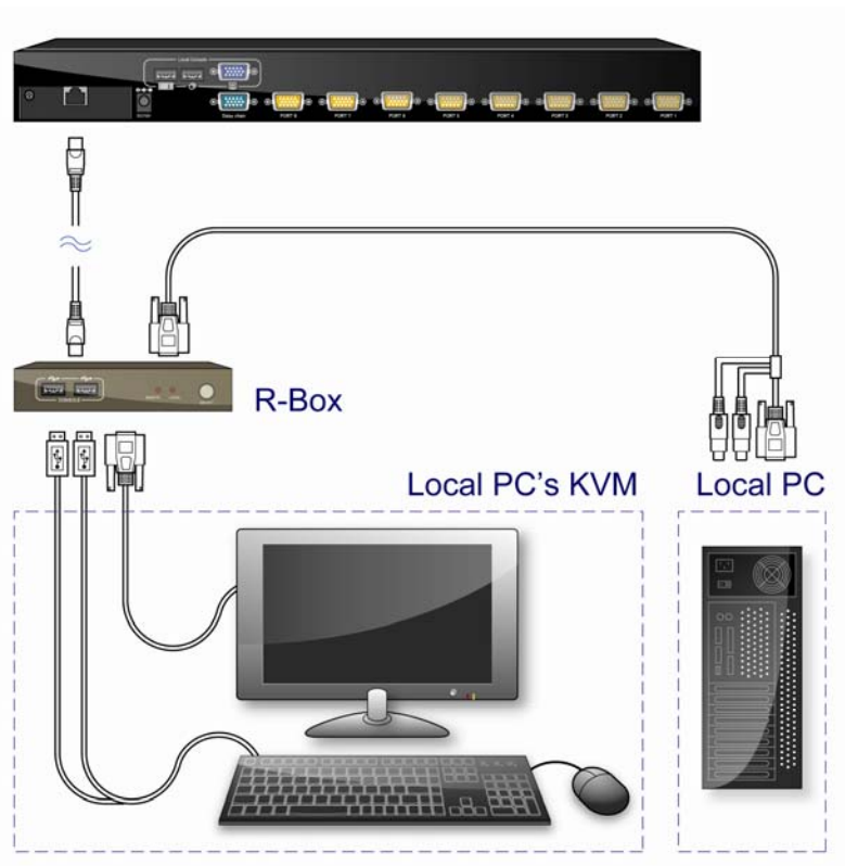
Figure 2-7. CAT5 Module Installation
