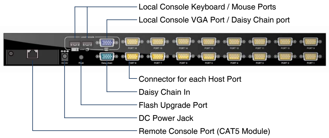
Figure 1-7. Rear Panel
