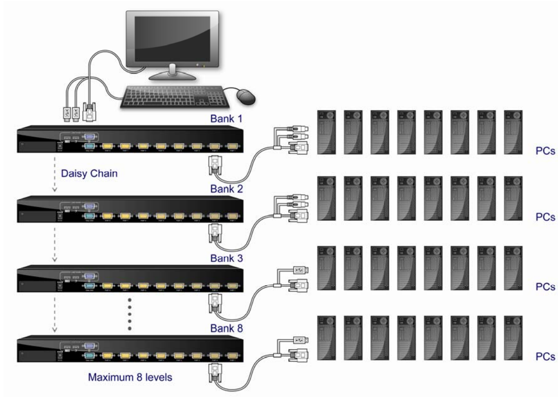
Figure 2-8. Daisy Chain Connection
