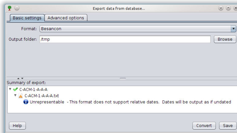
Figure 7.1: Screen showing a series that has been exported to Besançon format. In the summary of the export at the bottom of the screen you can see the warning to the user that this format does not have the ability to represent relative dates properly.
