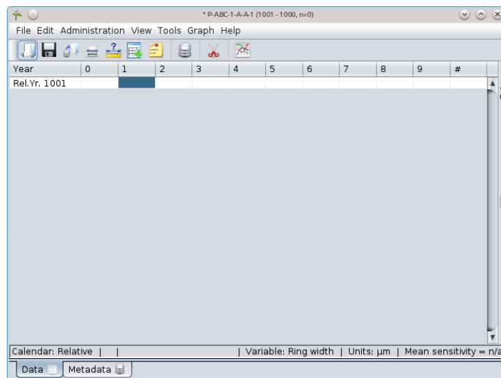
Figure 2.1: An empty data window ready to receive measurements. Note the status bar at the bottom includes buttons for changing the measurement variable, display units and cumulative statistics. The data table stores ring width values in decadal rows following the standard convention which derives from data entry via punch-cards. Undated sequences begin in the relative year 1001 for the same reason.
