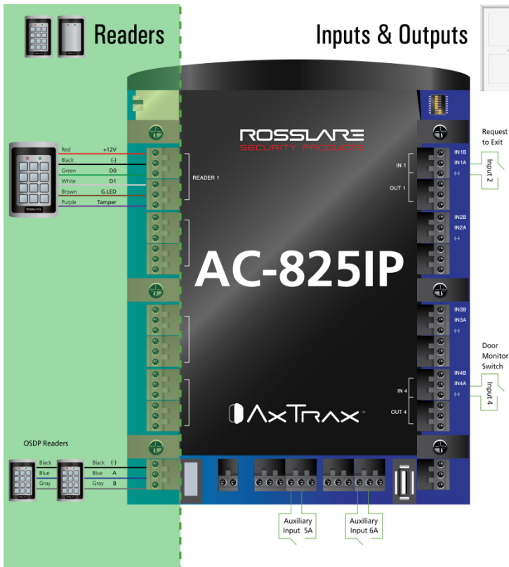
Figure 2: Input Wiring – Supervised Inputs
