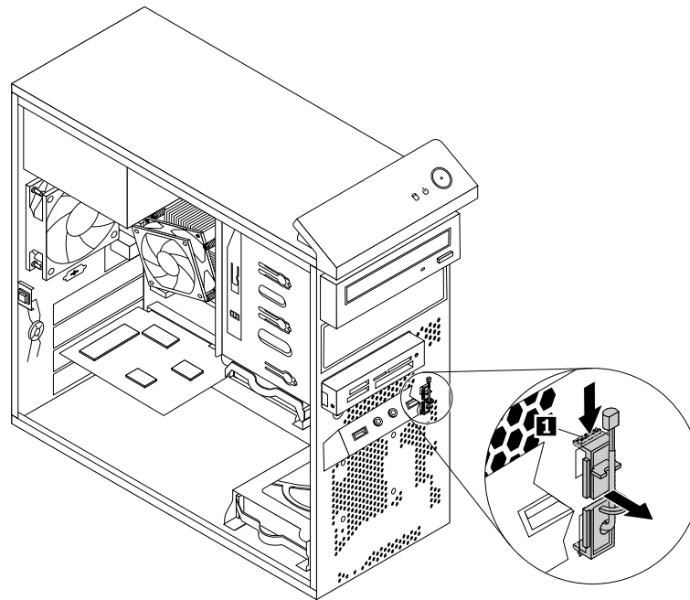
Figure 61. Removing the thermal sensor
