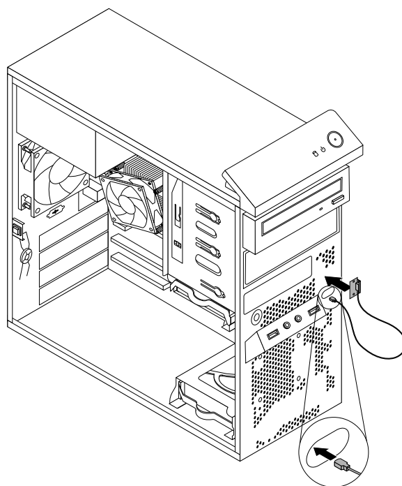
Figure 77. Installing the front WiFi antenna
