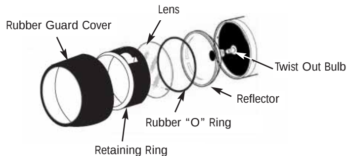
Figure 2. Lens Assembly
