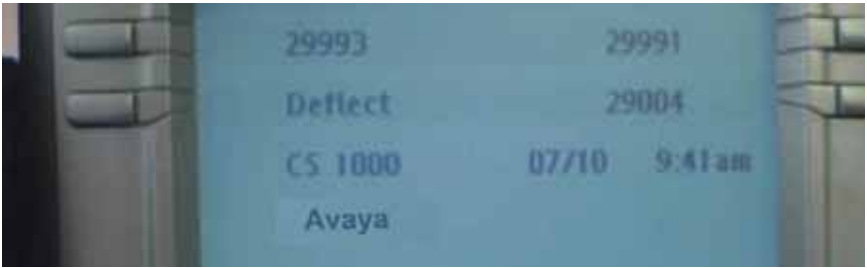
Figure 7: Call deflect
