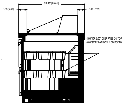
UCD4460N-12M RIGHT SIDE VIEW
