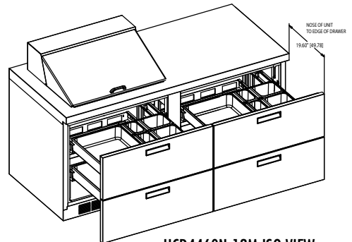
UCD4460N-12M ISO VIEW
