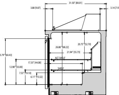
UC4460N-24M RIGHT SIDE VIEW
