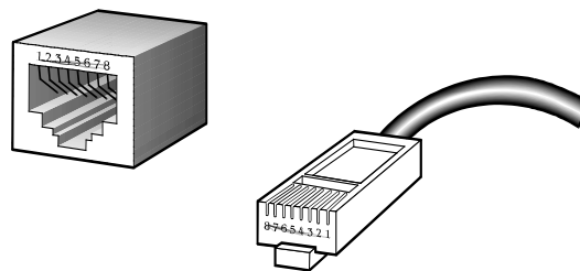
The standard RJ-45 receptacle/connector
