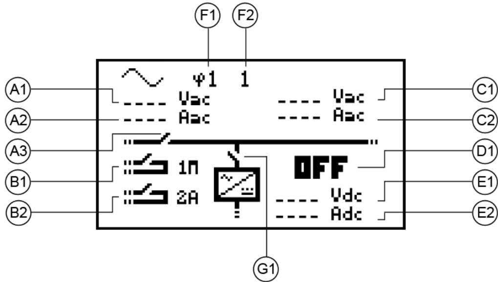
Fig. 4 - The RCC-03, main display
