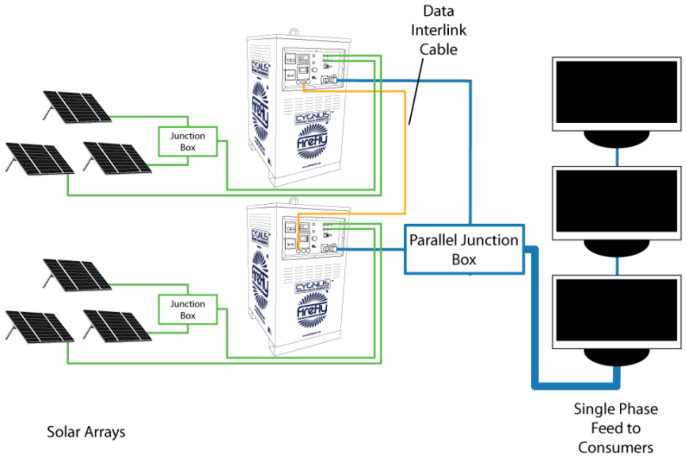
Fig. 9 - Example Showing the use of Two Units to Provide a Higher Output
