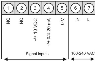
Type M3-7VR5A.0001.S70BD supply of 100-240 VAC
