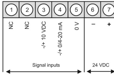
Type M3-7VR5A.0001.770BD supply of 24 VDC
