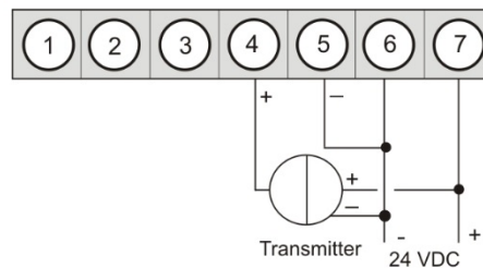
M3 in combination with a 3-wire-sensor 0/4-20 mA
