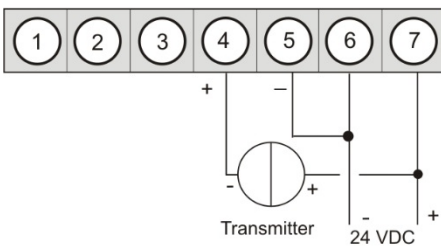
M3 in combination with a 3-wire-sensor 0-10 V
