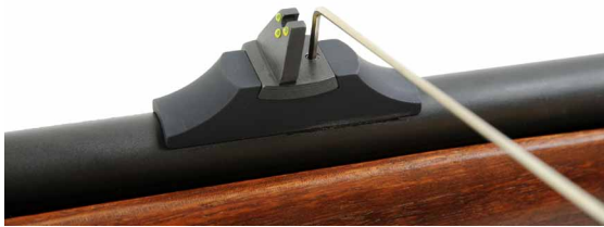
Fig. 29 Rear sight windage
