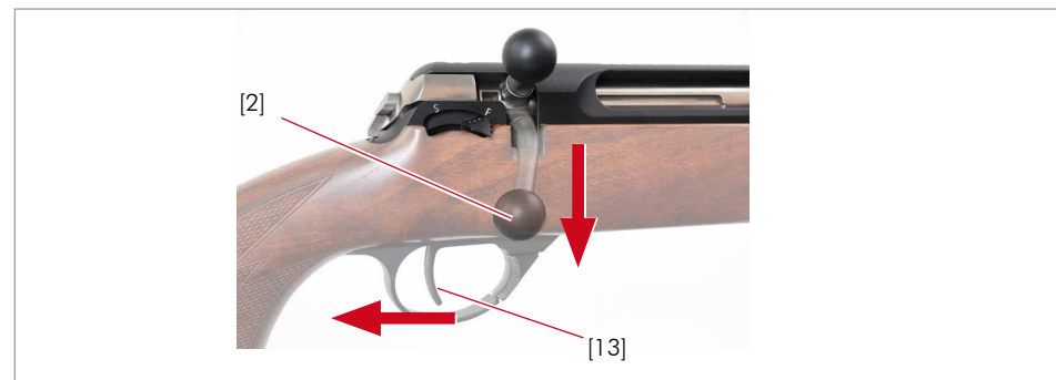
Fig.14 Pivoting the bolt handle downwards
