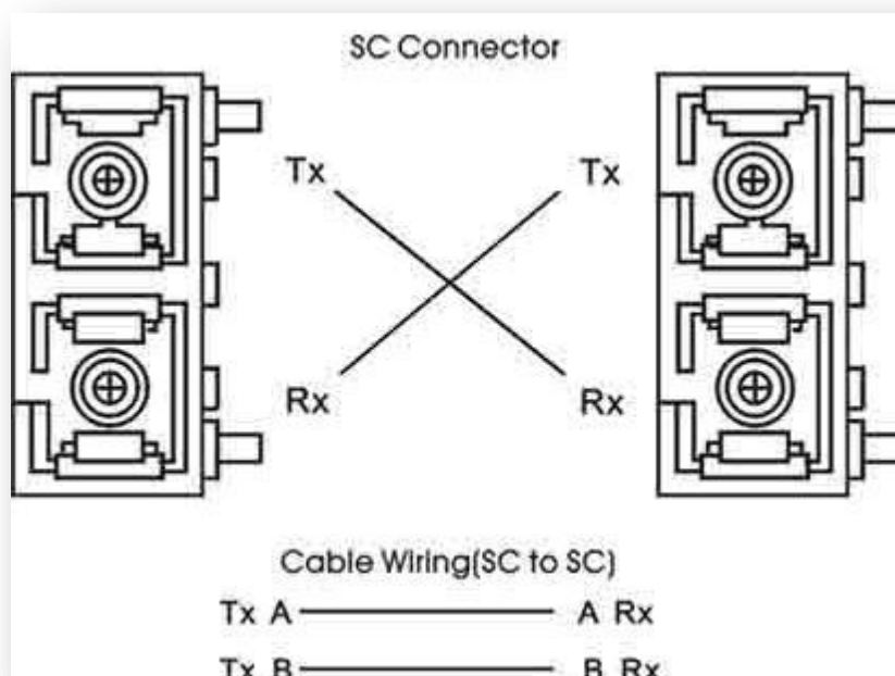
Figure 2.6 – Fiber Port Cabling
