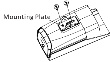
Figure 2-6 Screw the Mounting Plate
