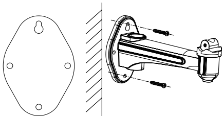
Figure 2-5 Drill Template & Install Mount
