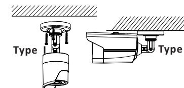
Figure 2-2 Fix the Camera to the Ceiling
