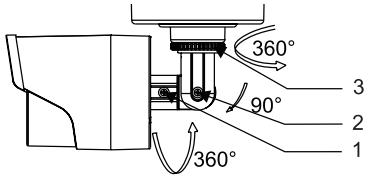
Figure 2-3 3-axis Adjustment
