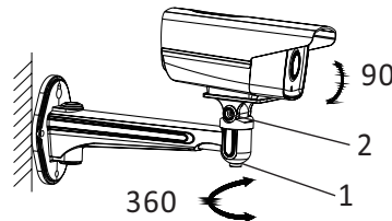
Figure 2-8 Angle Adjustment
