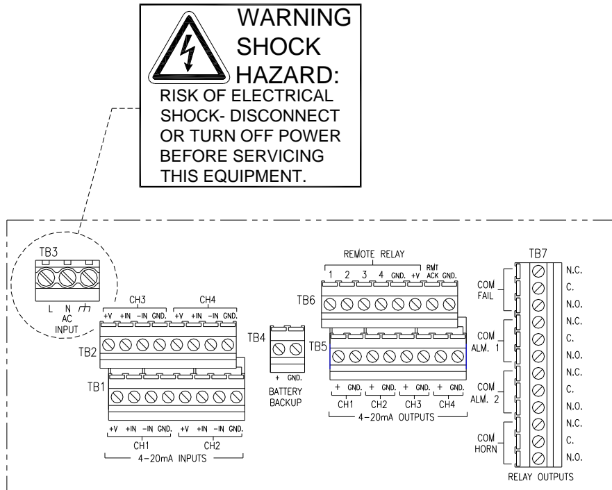
Figure 4 - Terminal Strip Layout
