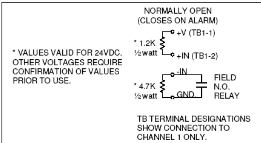
Figure 8 - Wiring of Normally Open Field Contact into Model 7400
