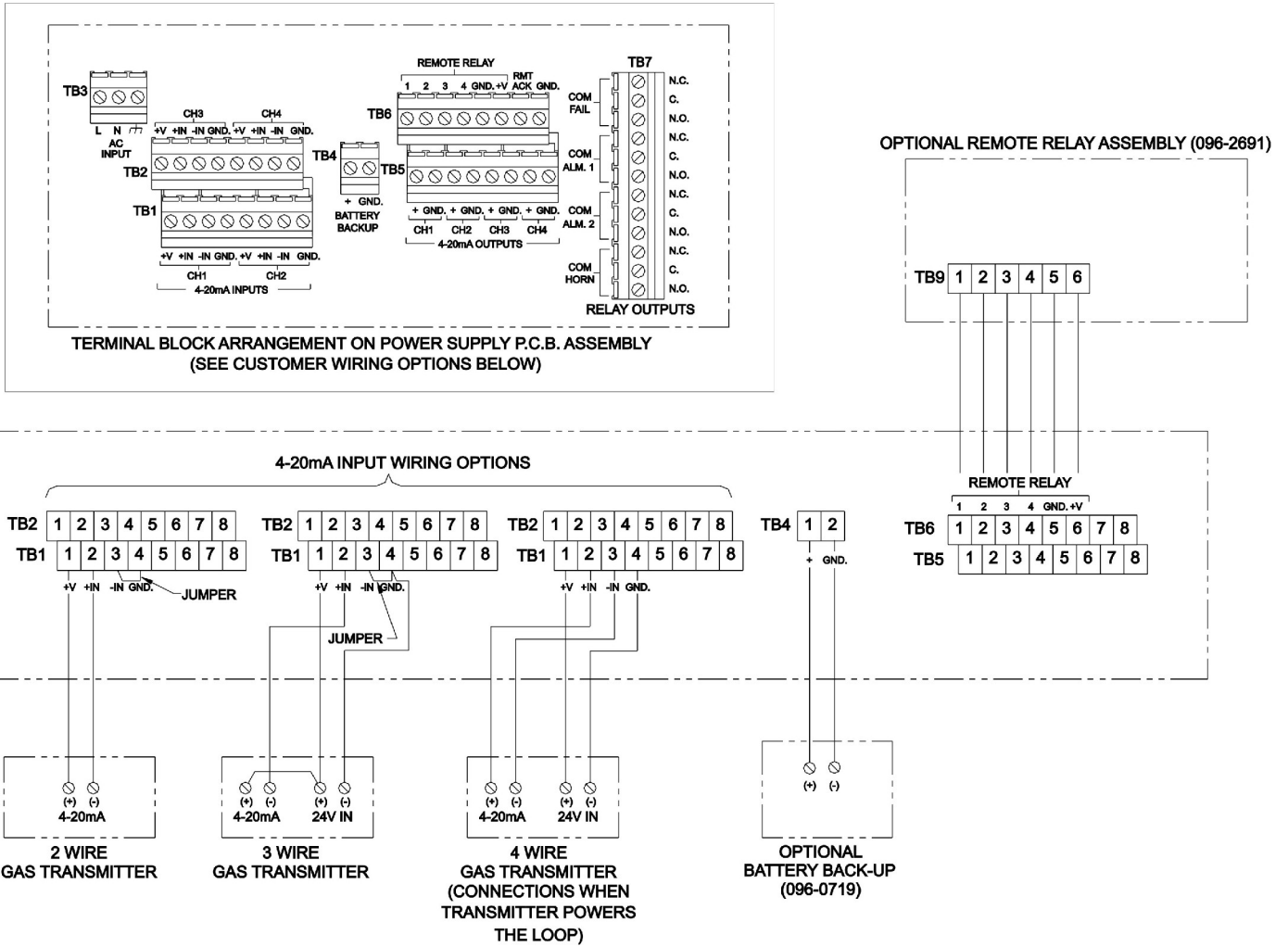
Figure 7 – Transmitter Wiring to Model 7400
