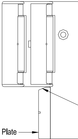
Figure 2A (Enclosure Side View)
