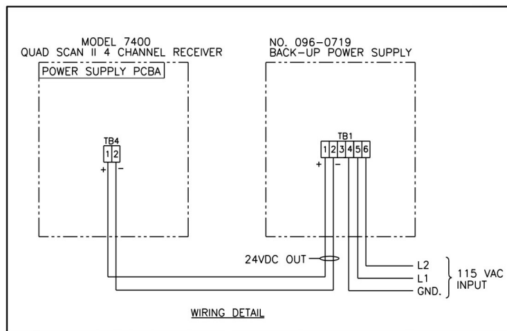
Figure 9 - Battery Backup (P/N 096-0719) Outline & Interconnection Wiring
