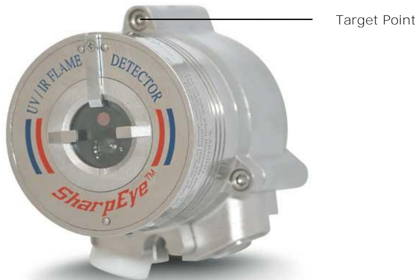
Figure 16: 40/40L, LB, L4, L4B UV/IR Detector Target Point
