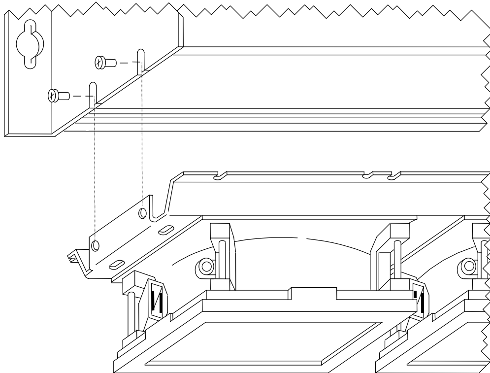
Mounting Details for Fan Assembly (AC Type Shown)
