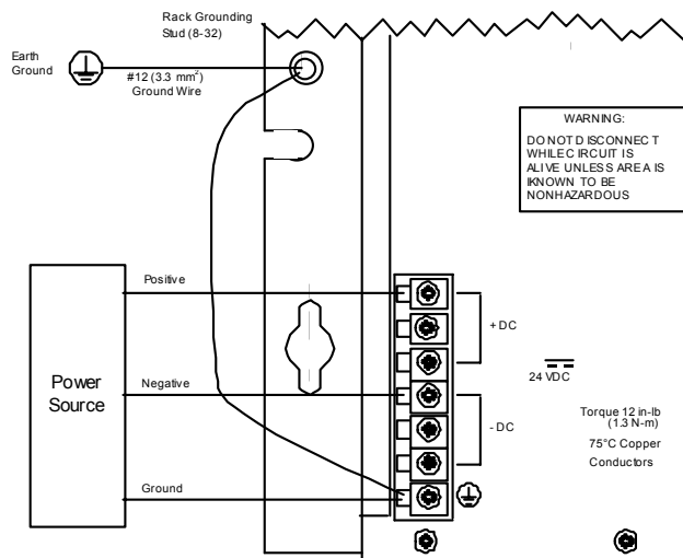
Terminal Board Connections for IC698PSD300
