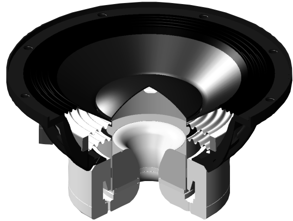
Figure 3. The TAD Reference One's Bass Drivers.
