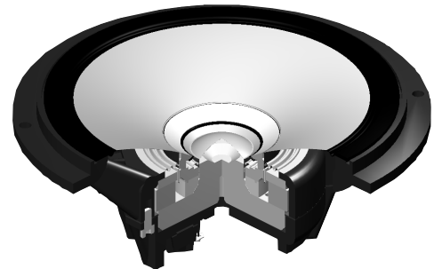
Figure 2. The TAD Reference One’s Coherent Source Transducer
