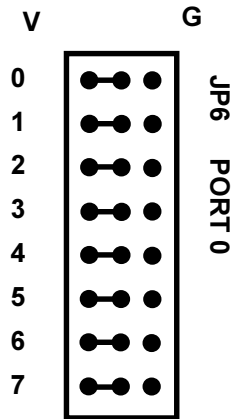
Fig. 1-9 — Port 0 Pull-up/Pull-down Resistor Connections, JP6
