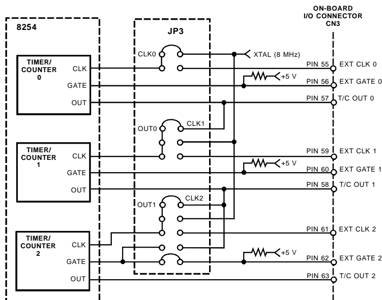
Fig. 1-5 — 8254 Circuit Diagram
