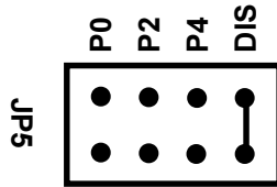
Fig. 1-6a: Strobe Disabled (Factory Setting)
