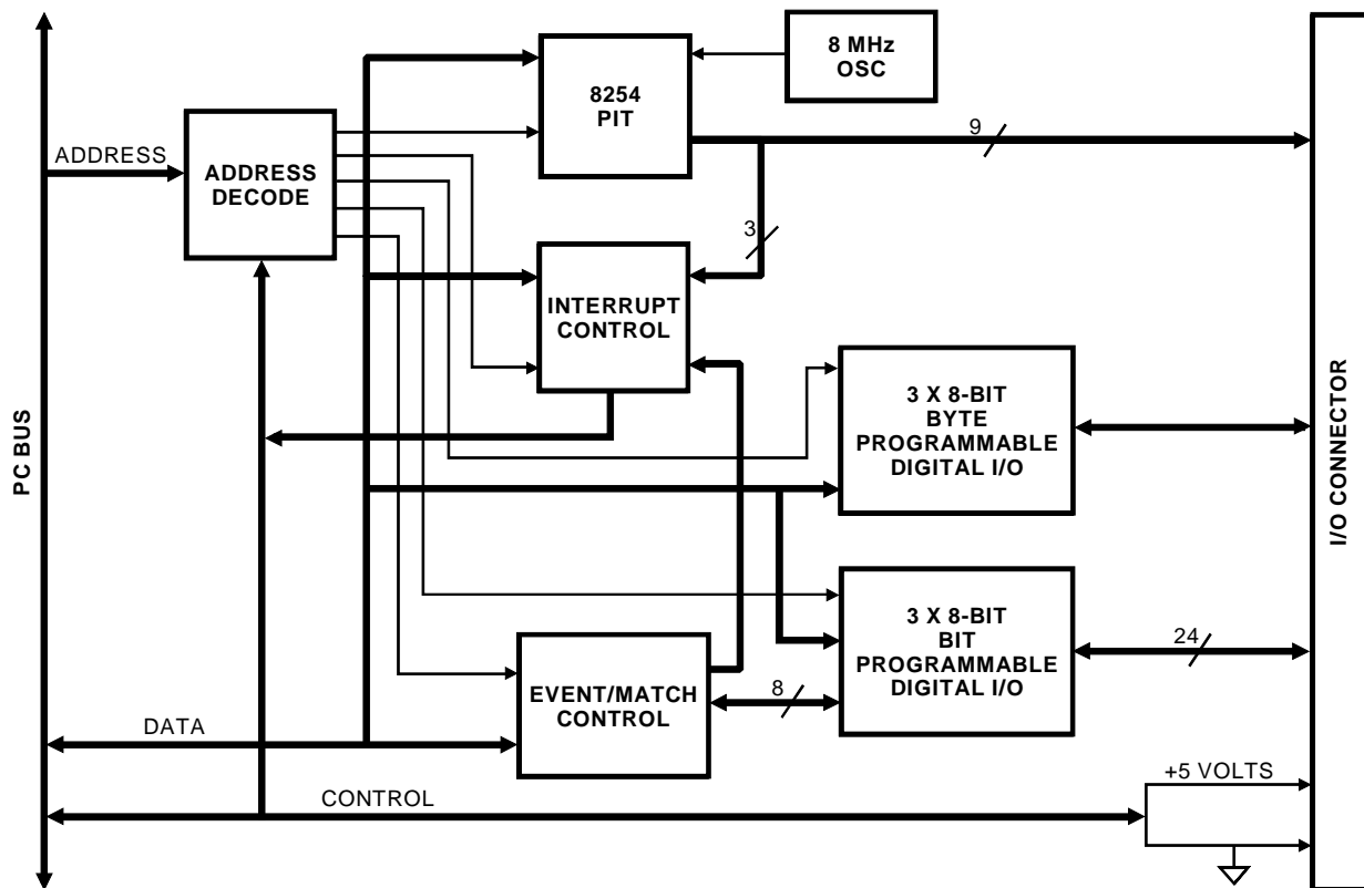
Fig. 3-1 — DM6910 Block Diagram
