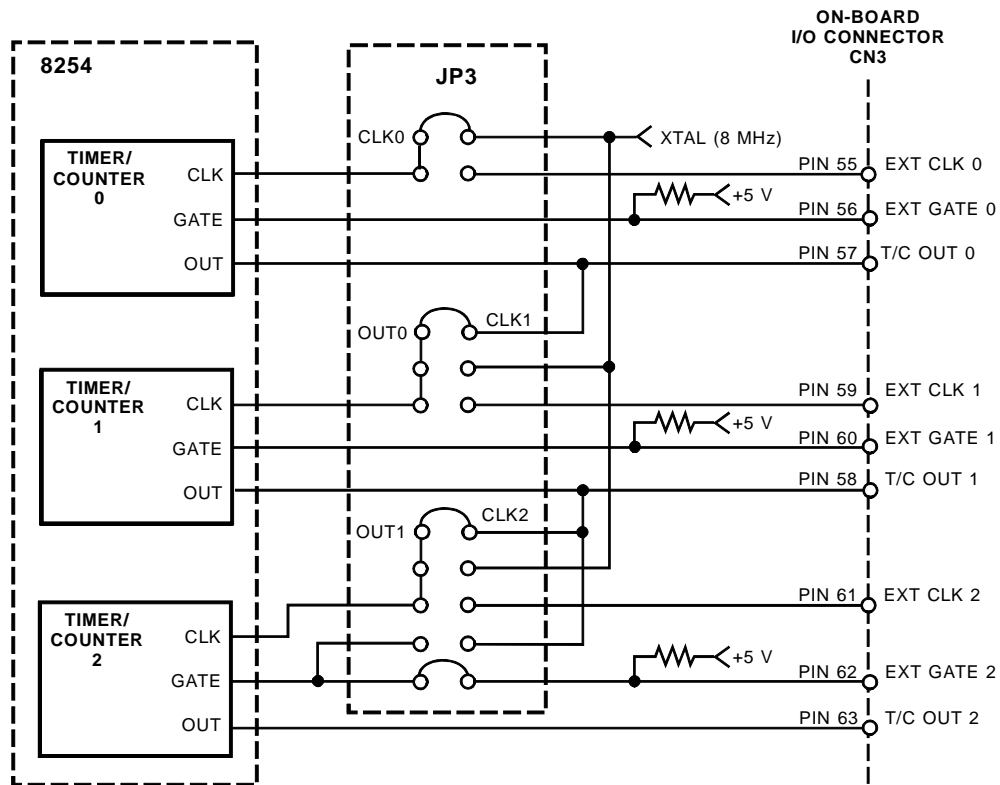
Fig. 3-2 — Timer/Counter Circuit Block Diagram
