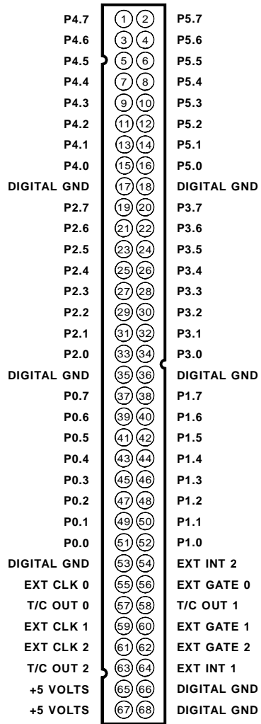
Fig. 2-1 — CN3 I/O Connector Pin Assignment
