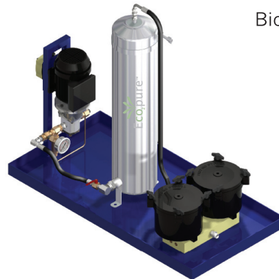
Biodiesel Wash & Polish Station includes suction & return hoses
