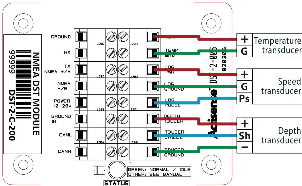
Figure 2 – Transducer connections
