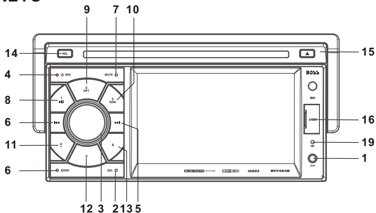
Control Panel
