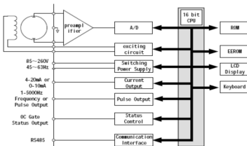
Fig. 1 Schematic of converter circuit
