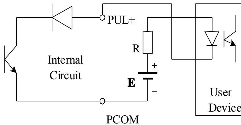
Fig. 14(e) Connection with photo-coupler (e.g. PLC)
