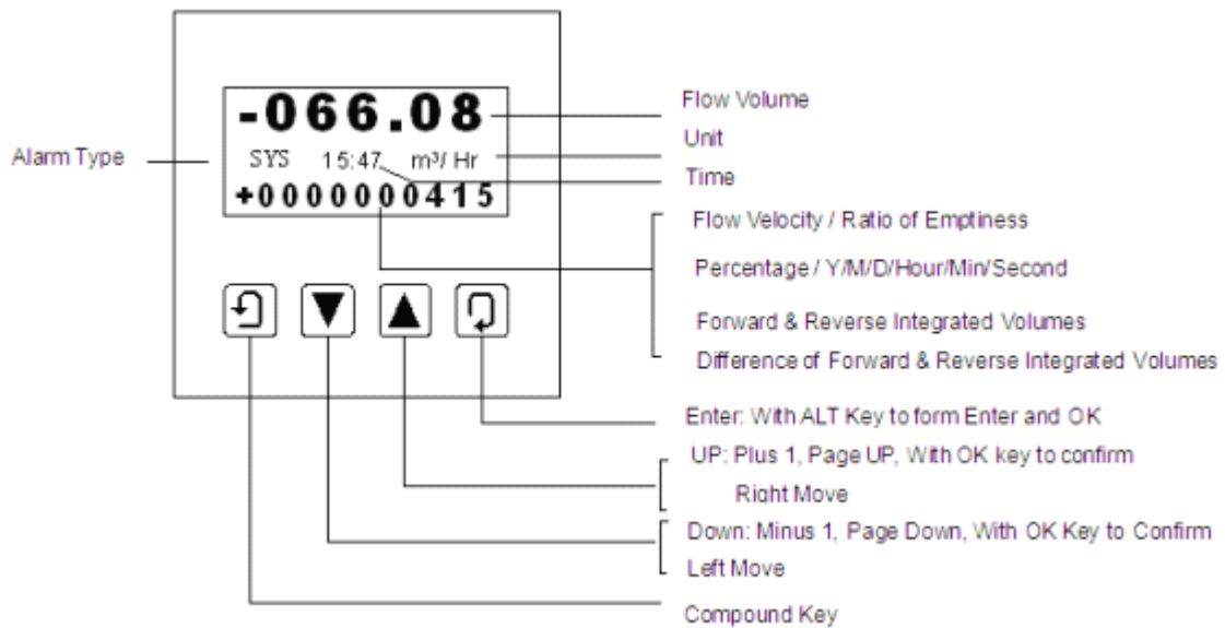
Fig.5(a) Remote-type key and display
