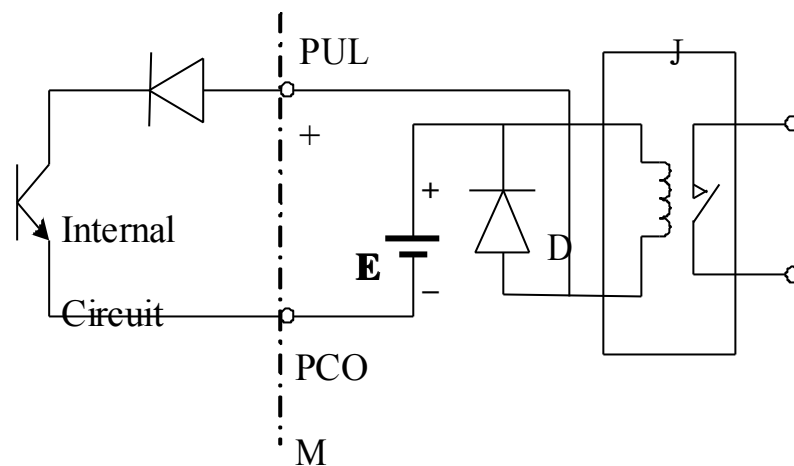
Fig.14 (f) Connection with relay (e.g. PLC)
