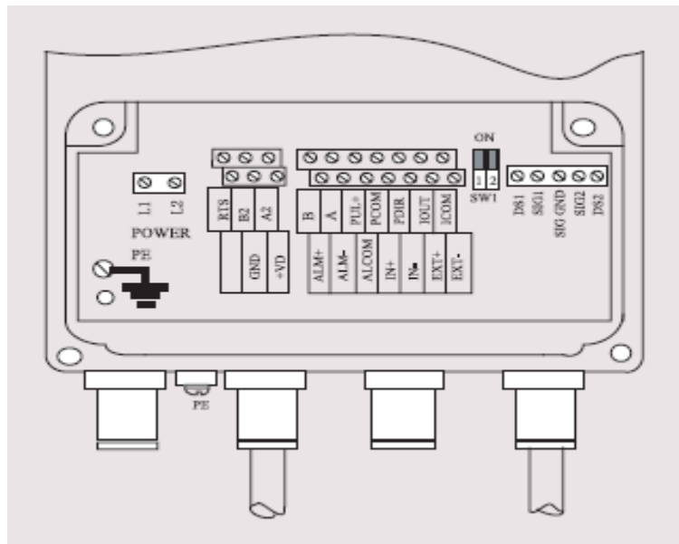
Fig. 8 Remote Type: Terminals and Marks
