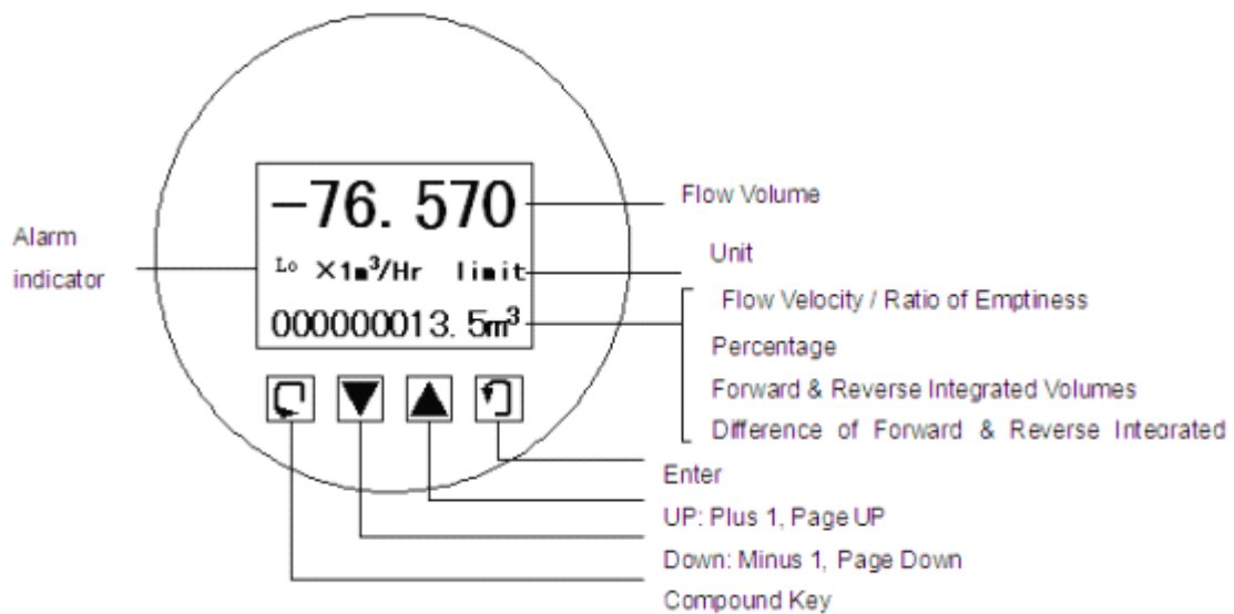
Fig.5(b) Compact-type key and display
