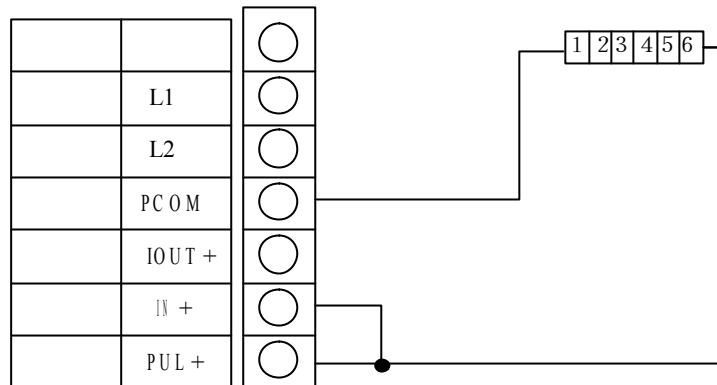
Fig. 14(c) Example of electrical counter connection
