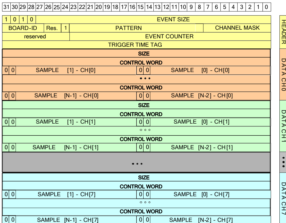
Fig. 3.9: Event Organization
