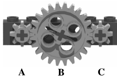
Figure 2-13. Idler Gear
