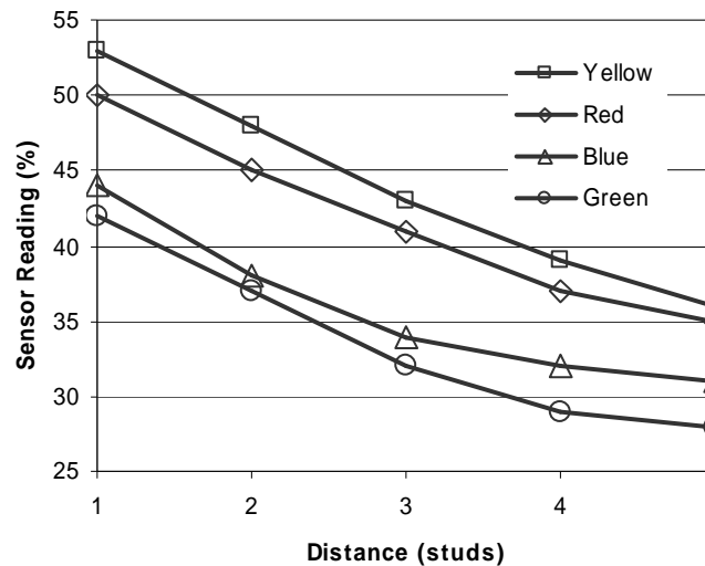
Figure 4-22. Color Experiment Sensor Readings
