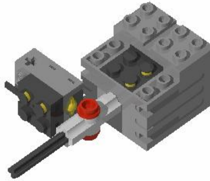
Figure 4-16. A Touch Rotation Sensor
