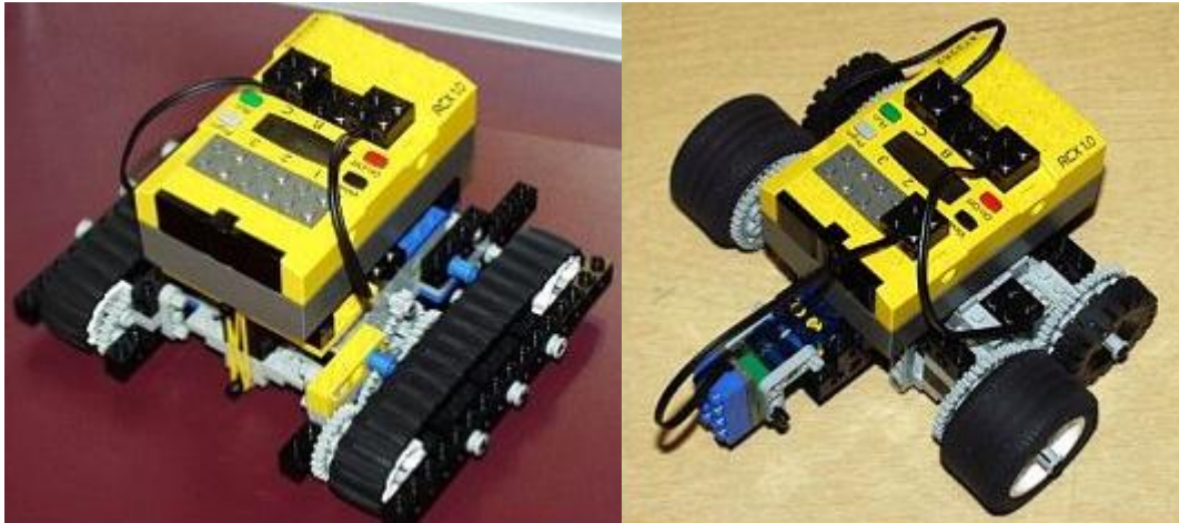
Figure 5-11. A Pair of Differential Skid Robots
