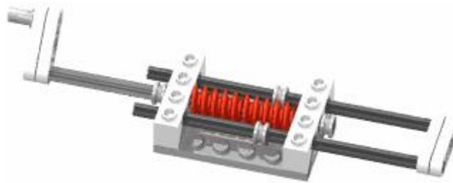
Figure 2-20. LEGO Lead Screw
