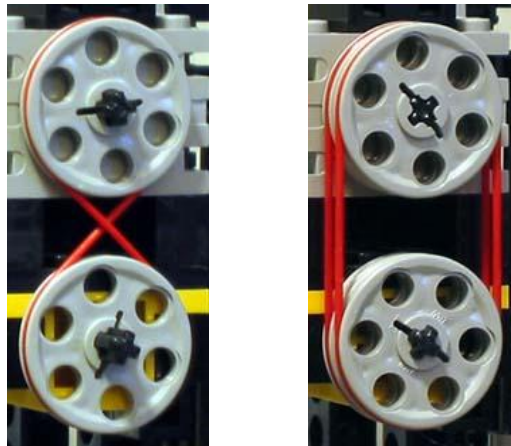
Figure 2-30. Two ways to Increase Torque Capacity
