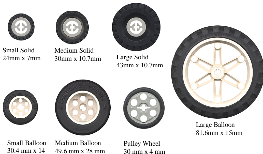
Figure 3-1. Lego Wheels and Tires
