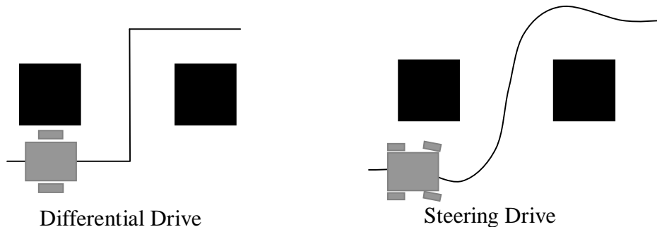
Figure 5-13. Path Planning is Harder for Non-Holonomic Robots
