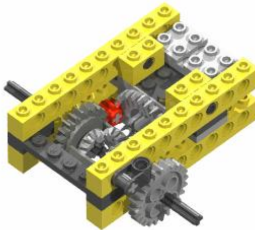
Figure 2-26. Ratchet Splitter
