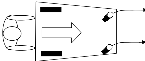
Figure 5-4. Casters Generate Steering Forces While Aligning
