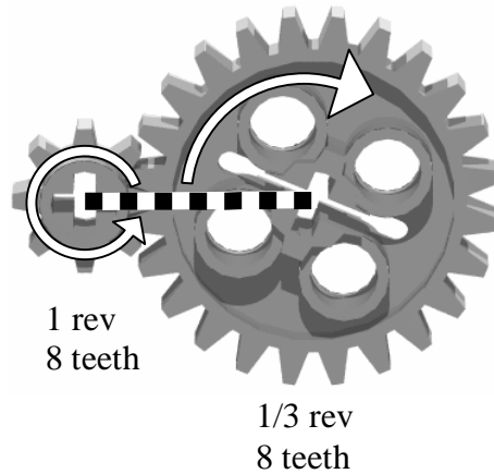
Figure 2-8. 3:1 Gear Ratio
