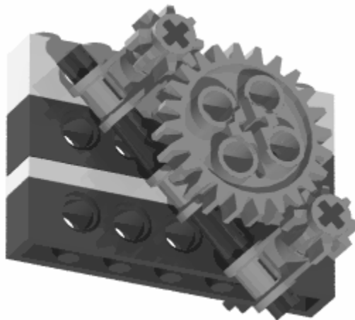
Figure 2-7. Circumventing Diagonal Gear Spacing Restrictions
