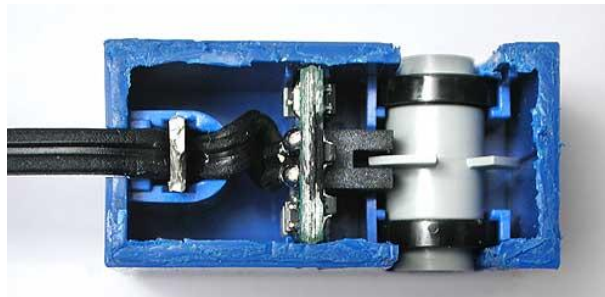
Figure 4-27. Rotation Sensor Internals. DON'T DO THIS!!!
