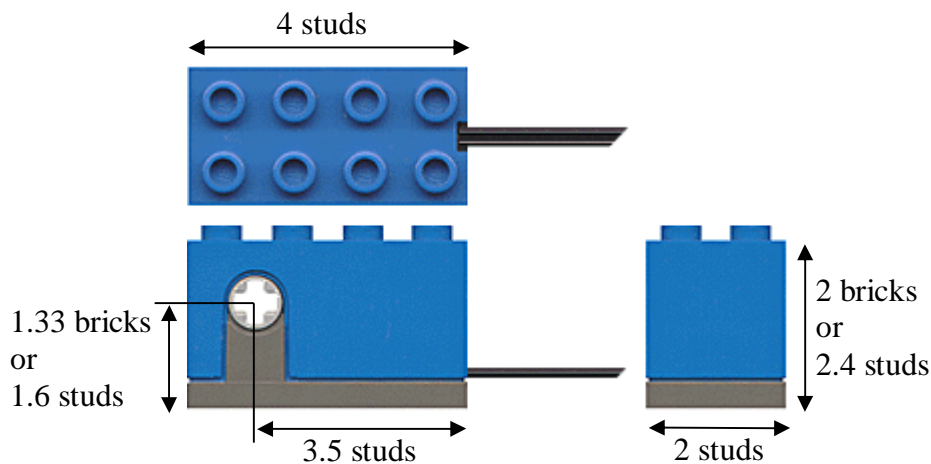
Figure 4-25. Rotation Sensor
