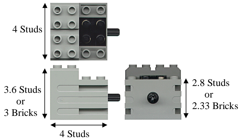
Figure 4-4. 9 Volt Geared Motor
