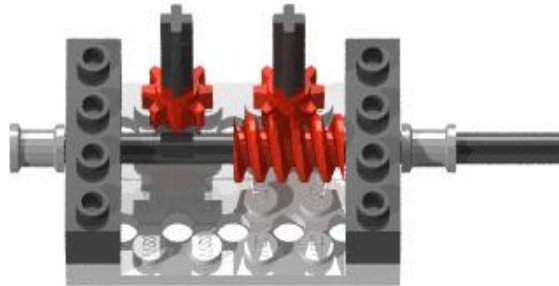
Figure 2-21. Directional Transmission
