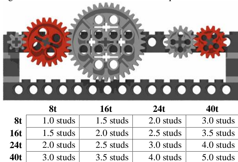
Figure 2-2. Stud Gear Spacing
