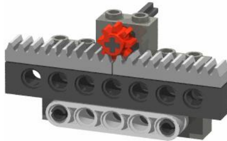
Figure 2-27. LEGO Gear Rack and Pinion
