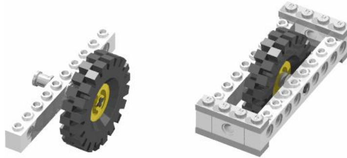
Figure 3-12. Cantilevered and Fully Supported Wheels
