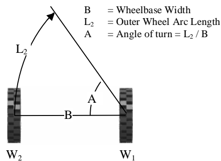
Figure 5-8. Pivoting About a Wheel
