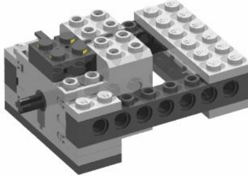
Figure 4-9. Motor Mount Using Rails
