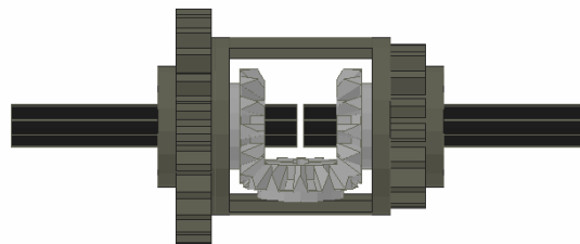
Figure 2-22. LEGO Differential
