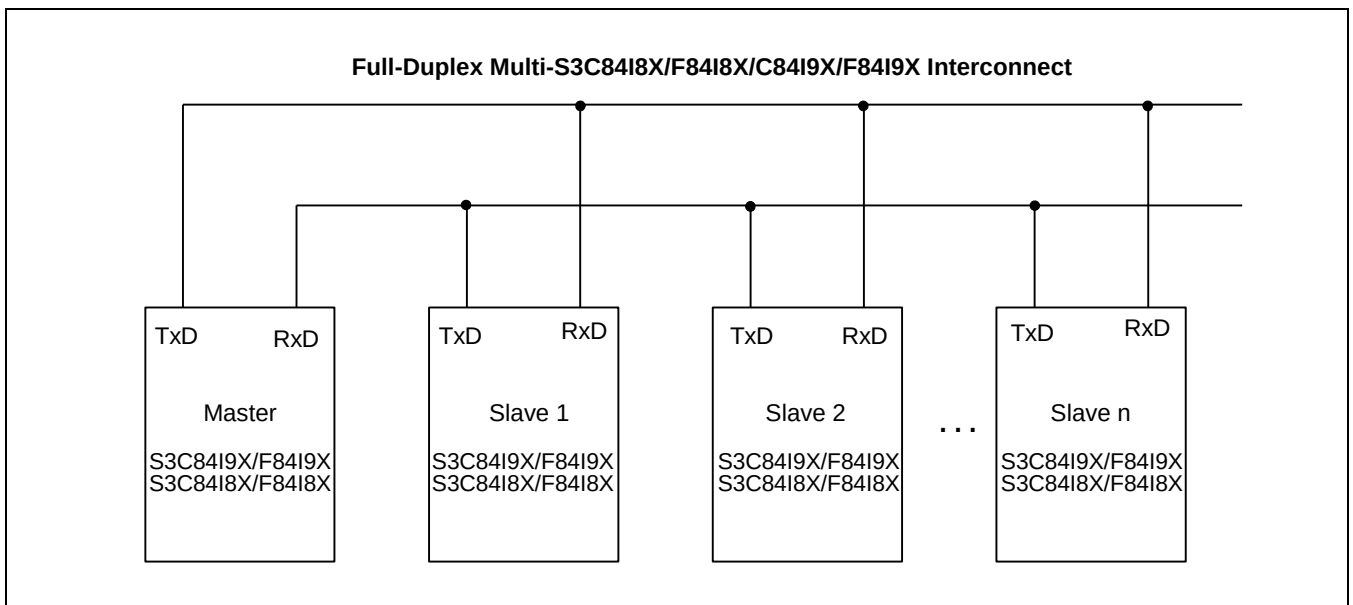
Figure 15-9 Connection Example for Multiprocessor Serial Data Communications
