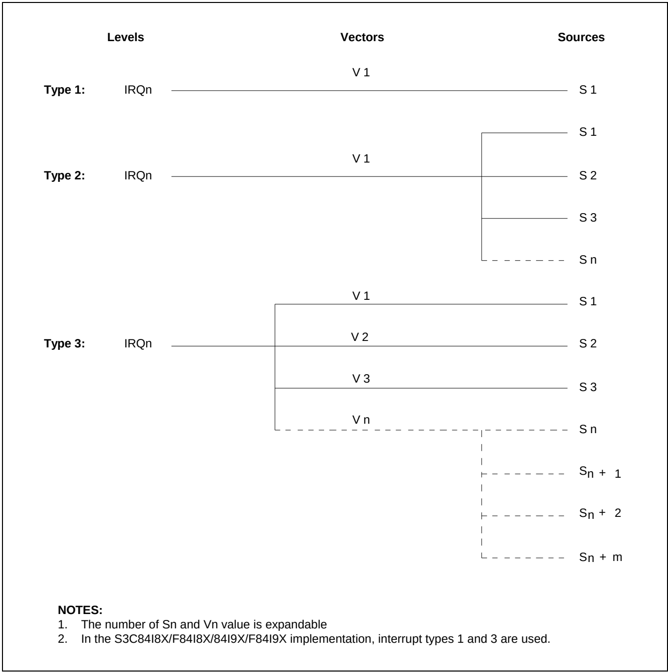
Figure 5-1 S3C8-Series Interrupt Types
