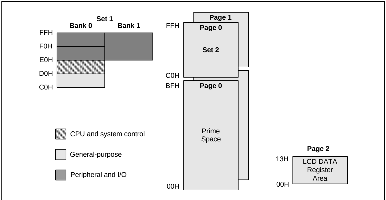
Figure 2-6 Set 1, Set 2, Prime Area Register (S3C84I9X/F84I9X)
