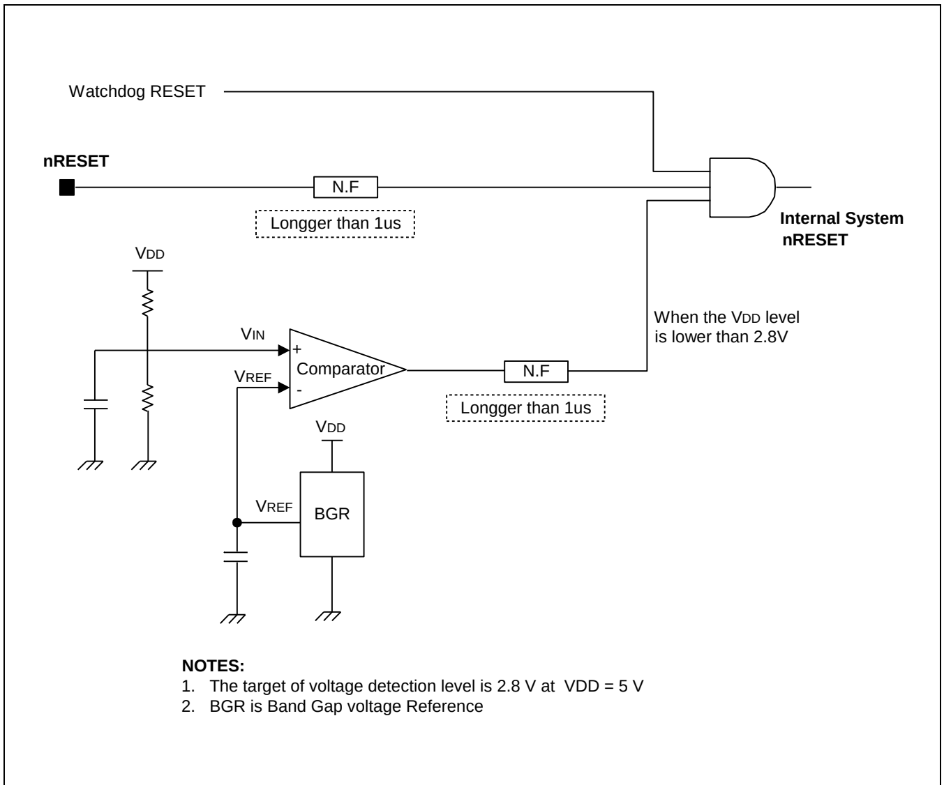
Figure 19-1 Low Voltage Reset Circuit
