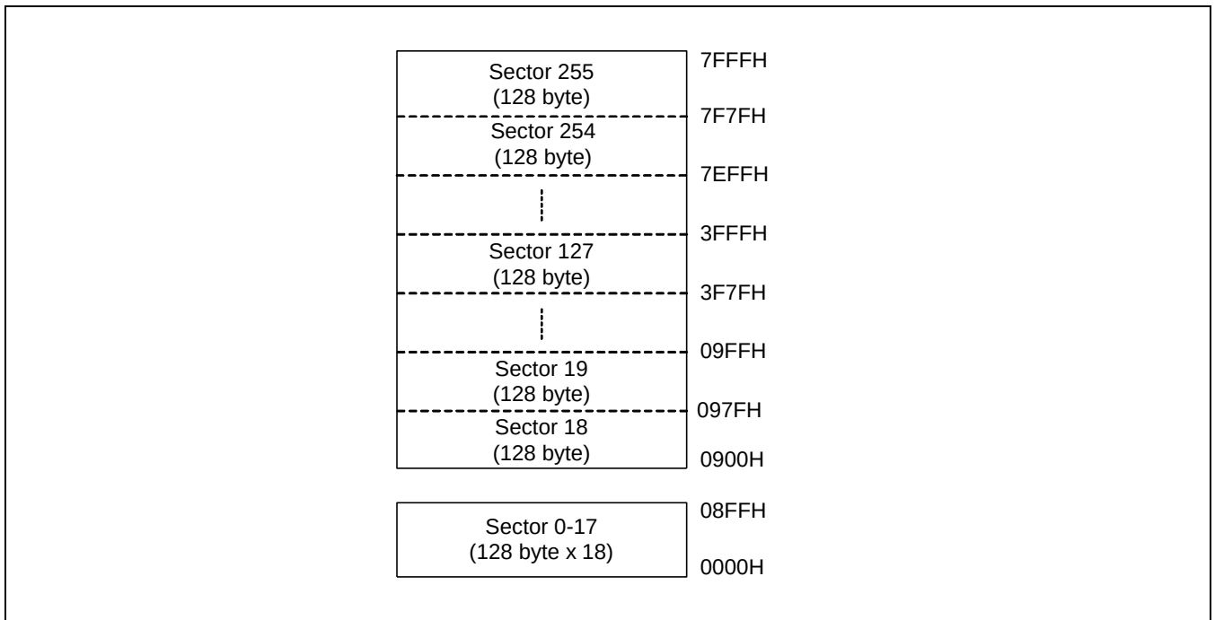
Figure 20-3 Sectors in User Program Mode
