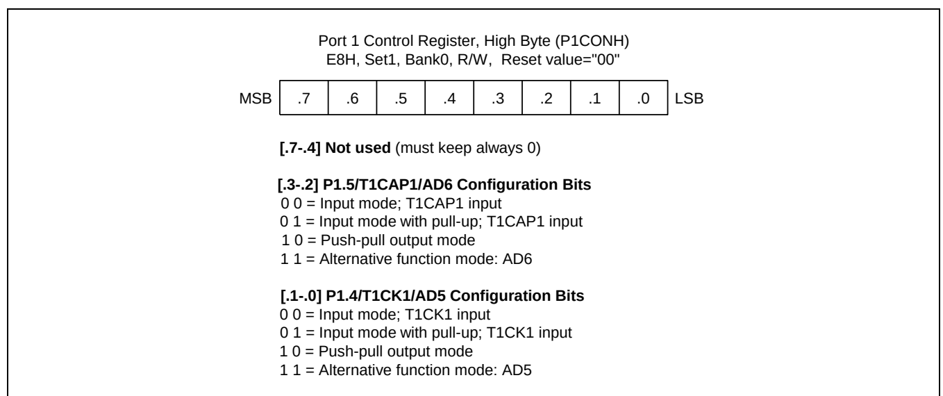
Figure 9-2 Port 1 High-Byte Control Register (P1CONH)
