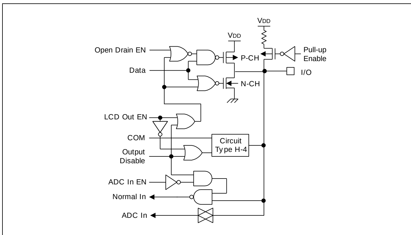
Figure 1-11 Pin Circuit Type H-16 (P0.0–P0.3)
