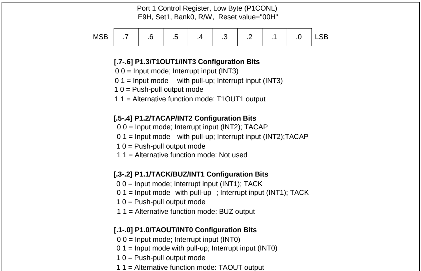
Figure 9-3. Port 1 Low-Byte Control Register (P1CONL)
