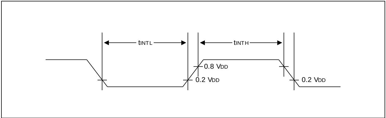
Figure 21-1 Input Timing for External Interrupts (Ports 2)
