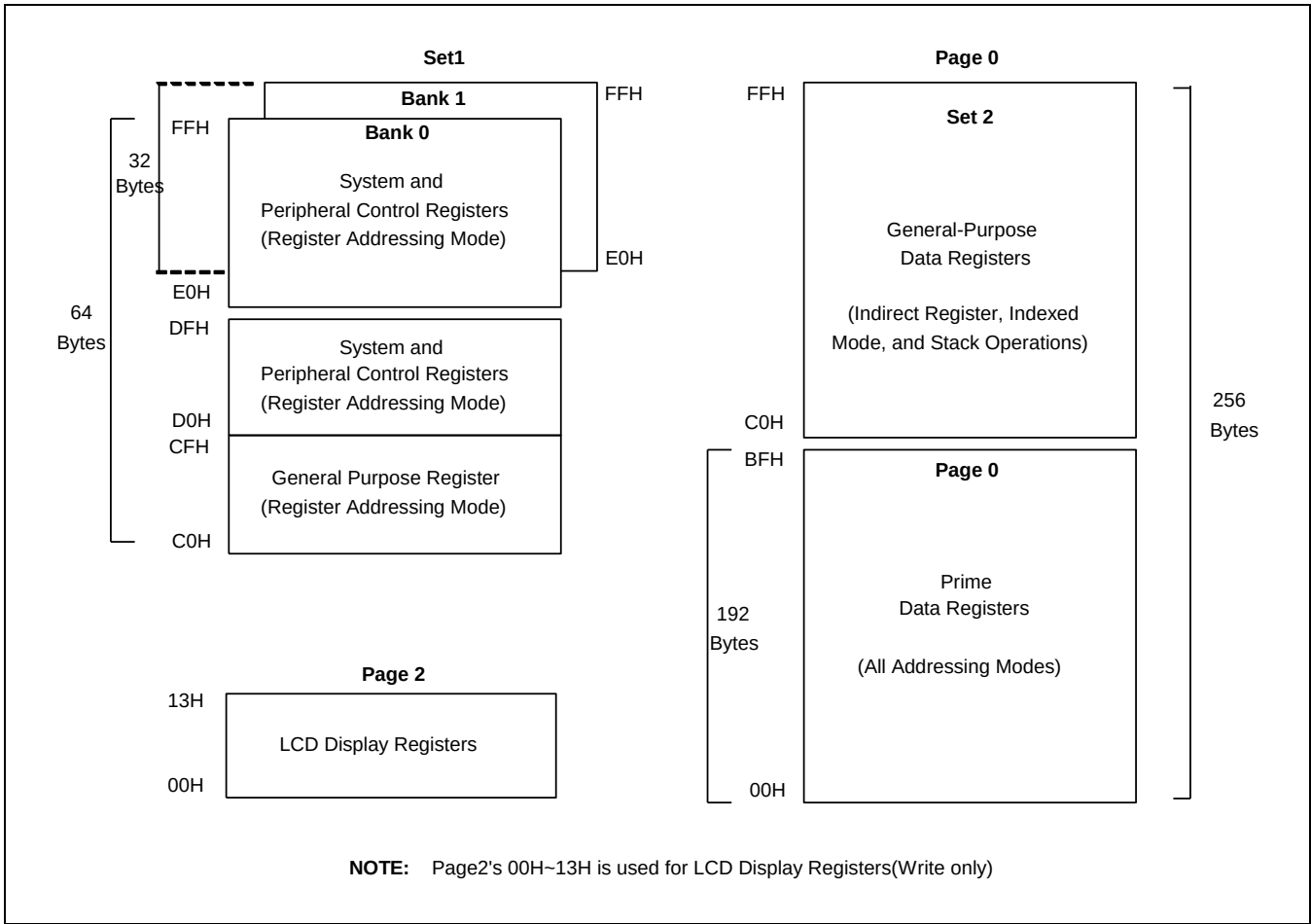
Figure 2-4 Internal Register File Organization of S3F84I8X/C84I8X
