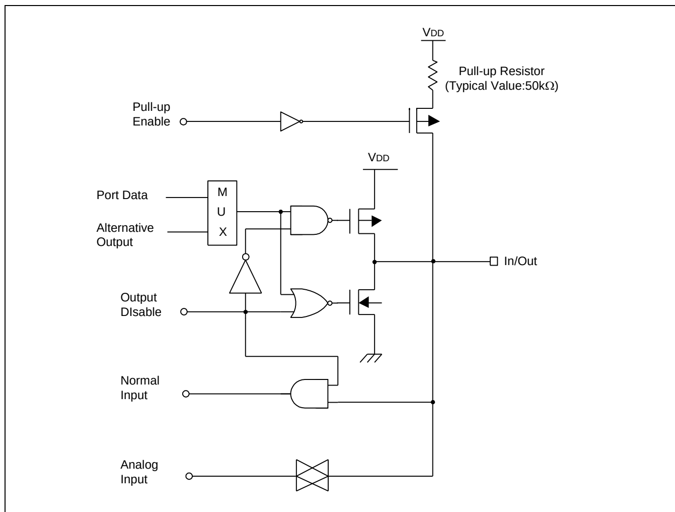
Figure 1-8 Pin Circuit Type E (P2.2-P2.3)
