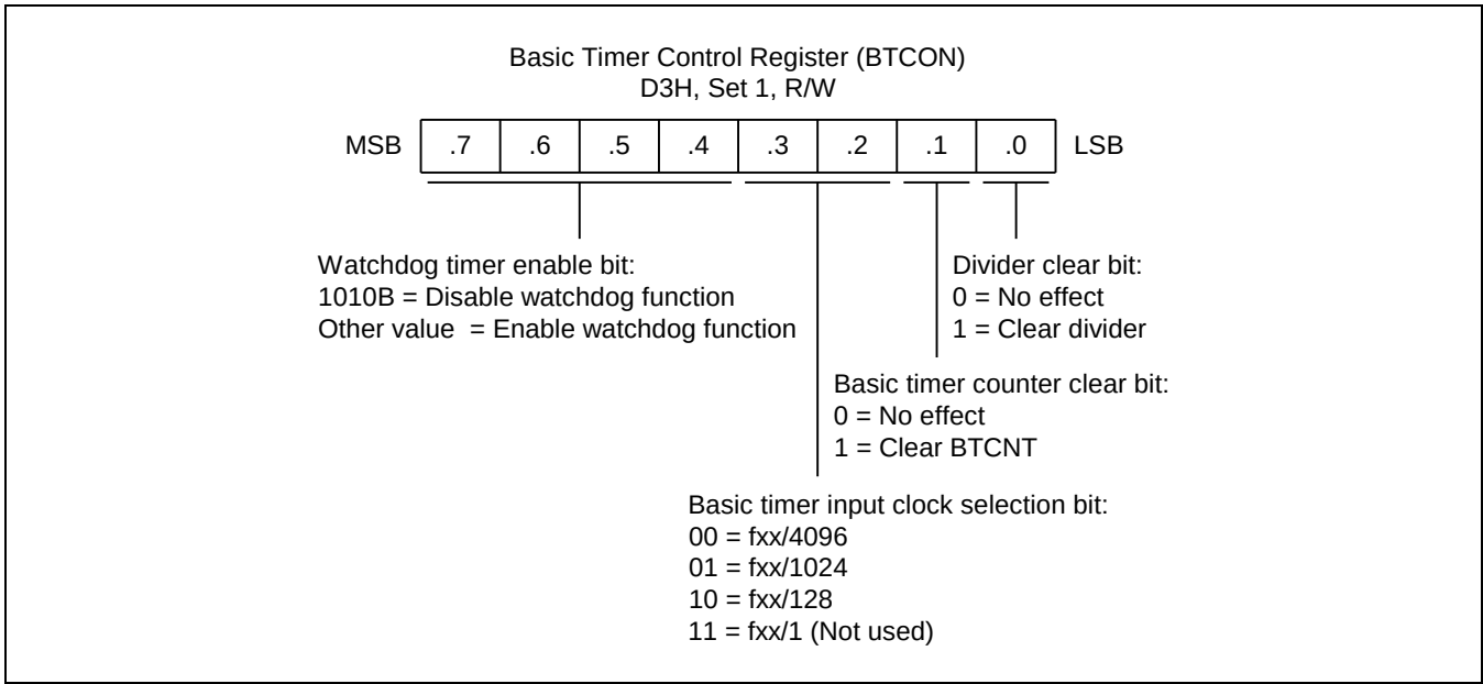
Figure 10-1 Basic Timer Control Register (BTCN)
