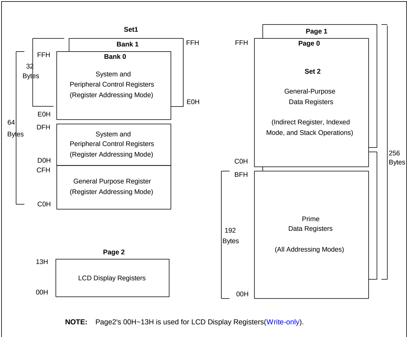
Figure 2-3. Internal Register File Organization of S3F84I9X/C84I9X
