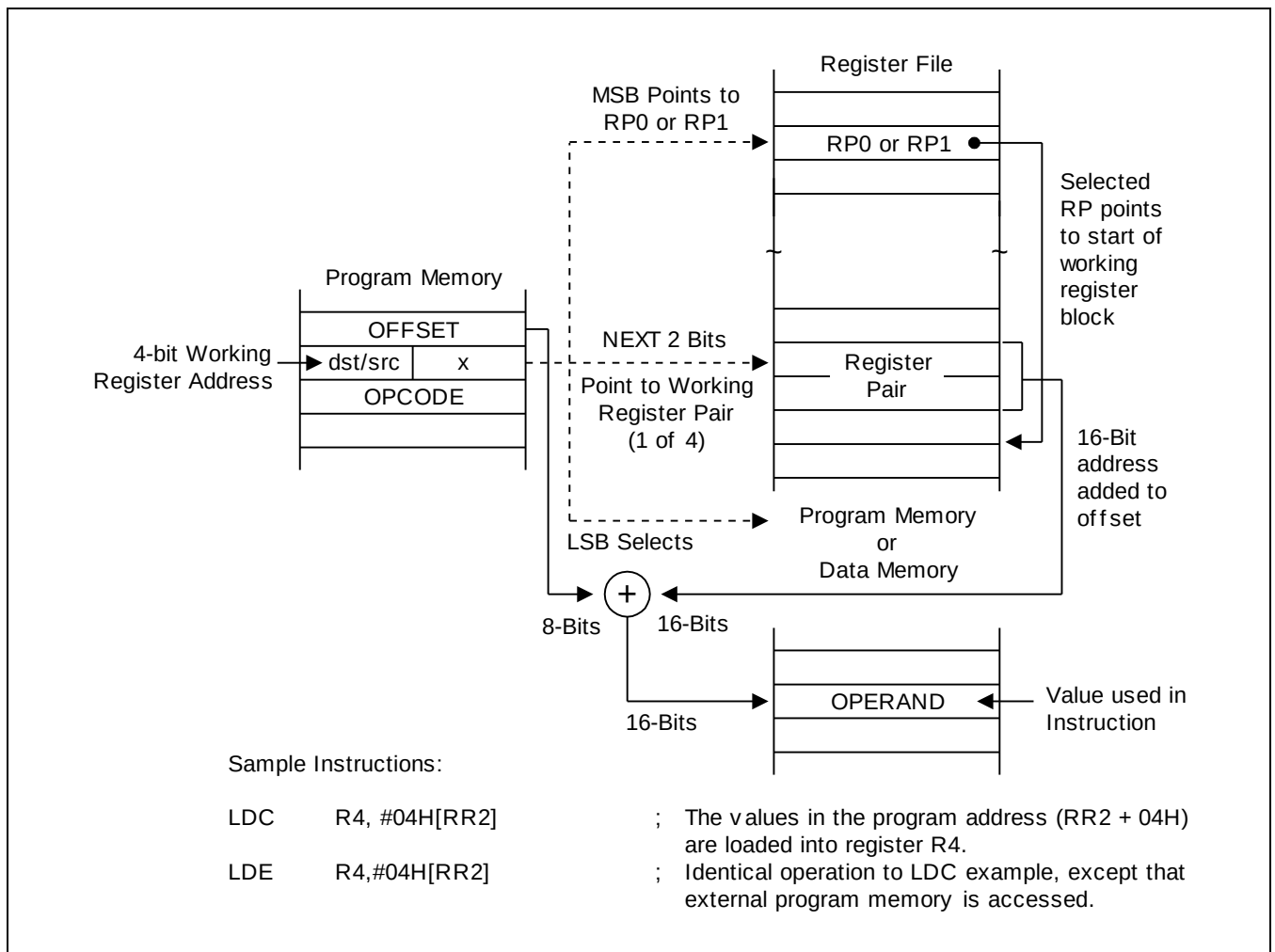
Figure 3-8 Indexed Addressing to Program or Data Memory with Short Offset
