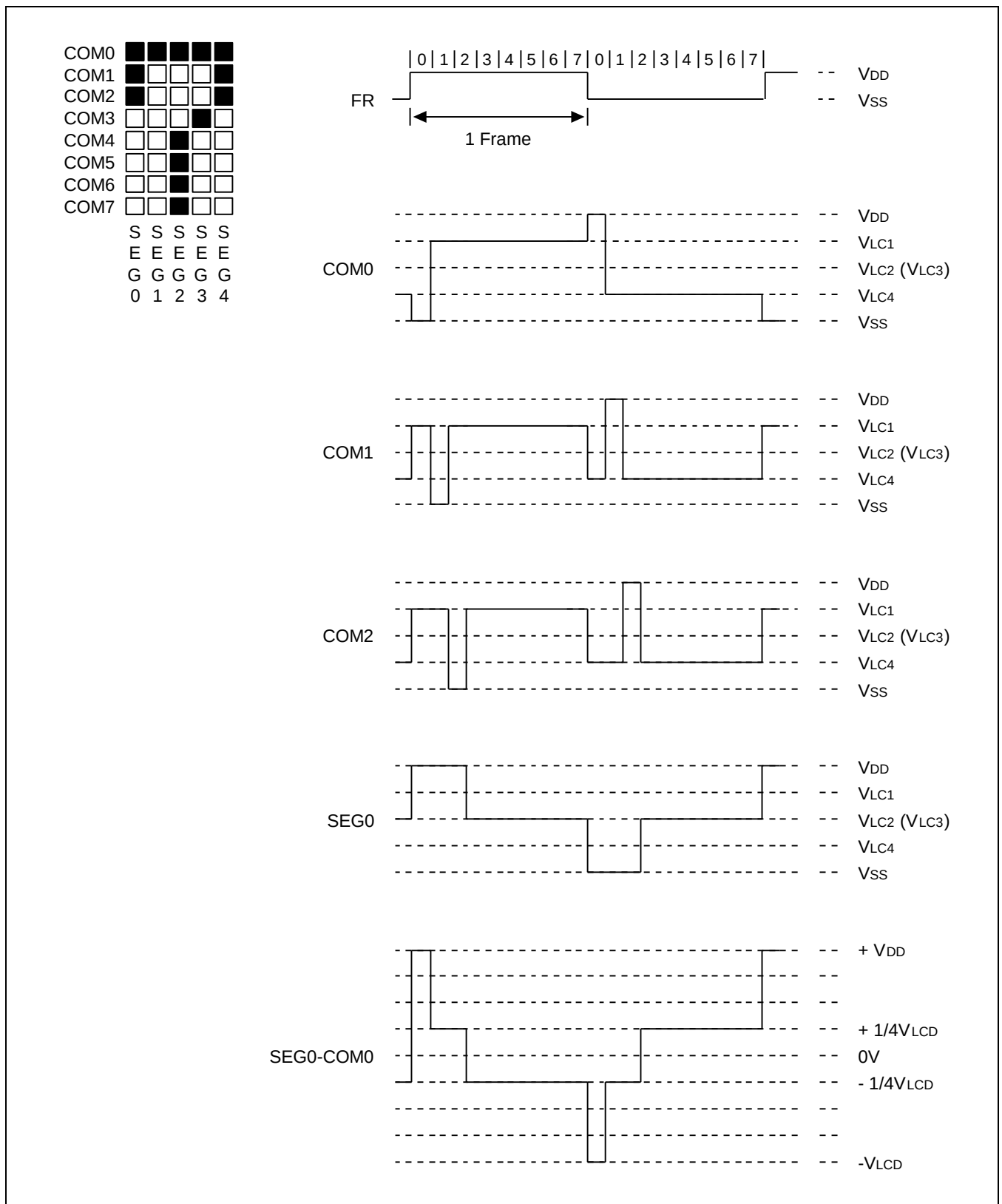
Figure 18-7 LCD Signal Waveforms (1/8 Duty, 1/4 Bias)
