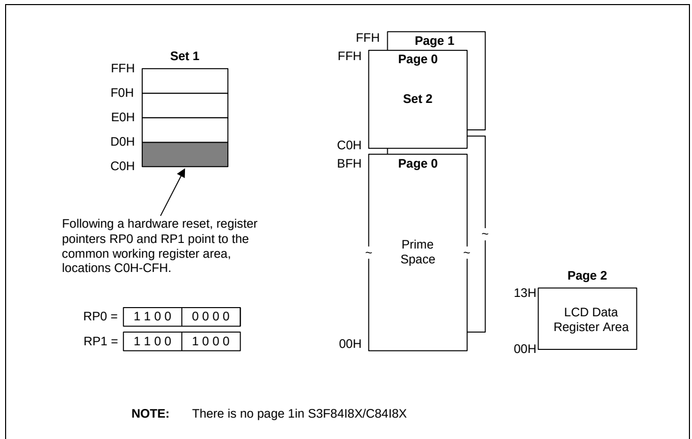
Figure 2-13 Common Working Register Area
