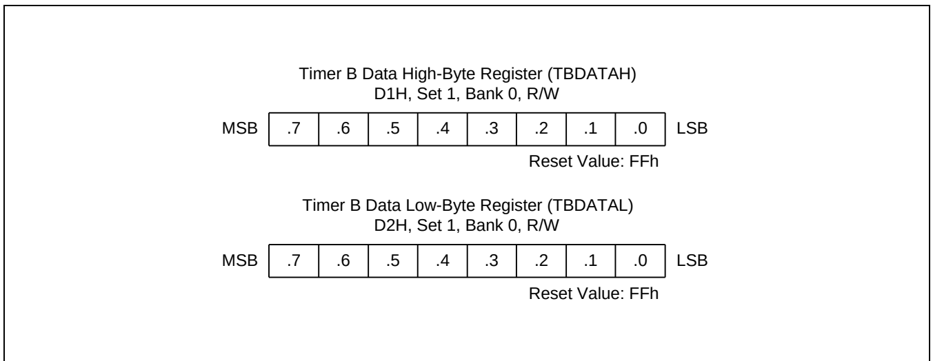
Figure 11-5 Timer B Data Registers (TBDATAH, TBDATAL)
