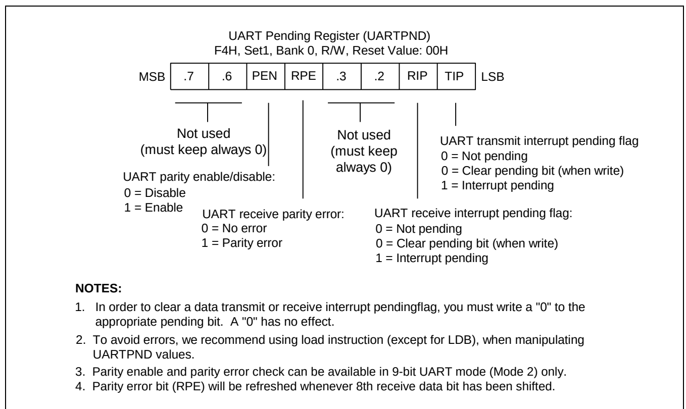
Figure 15-2 UART Interrupt Pending Register (UARTPND)
