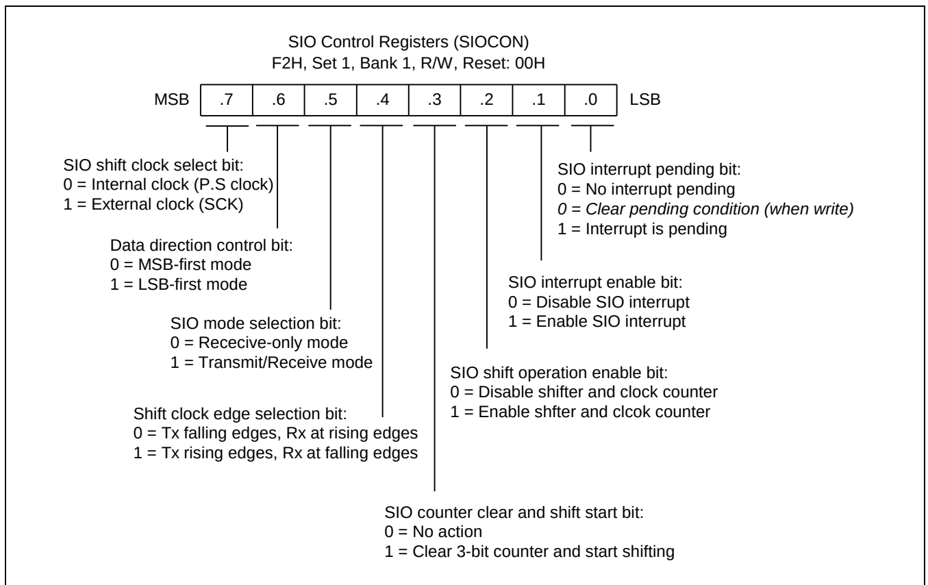
Figure 14-1 Serial I/O Interface Control Register (SIOCON)
