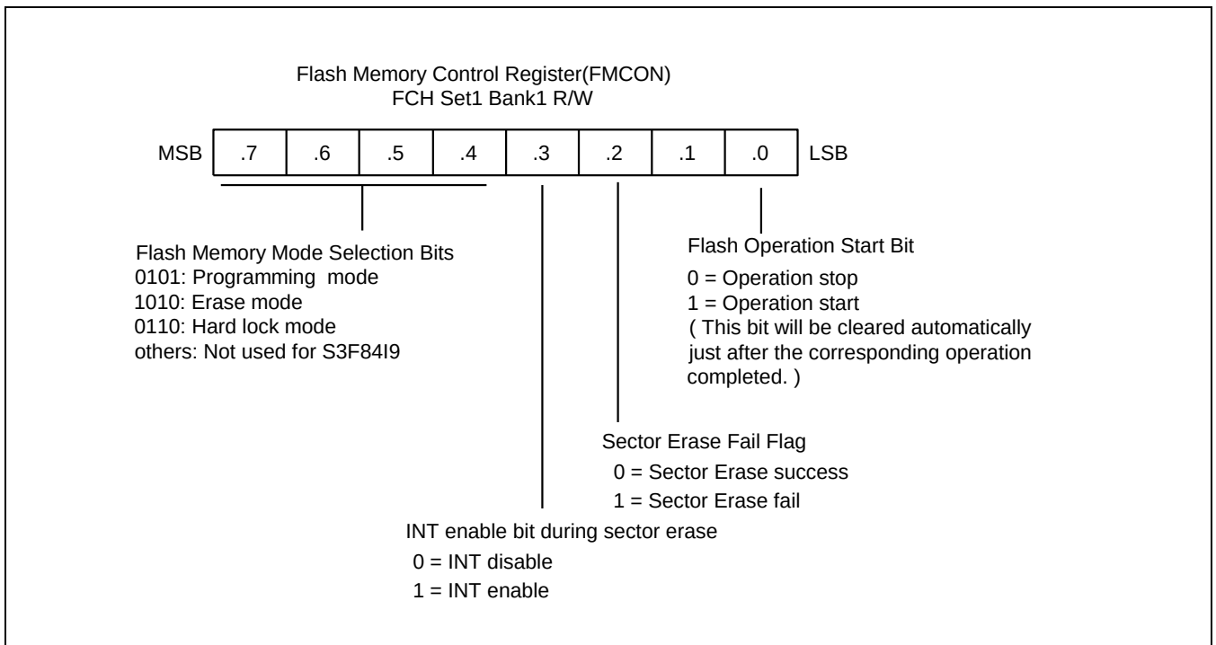
Figure 20-1 Flash Memory Control Register (FMCON)
