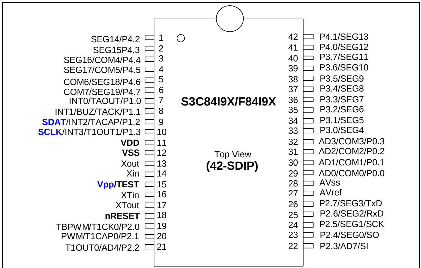
Figure 1-3. S3C84I9X/F84I9X Pin Assignment (42-pin SDIP)
