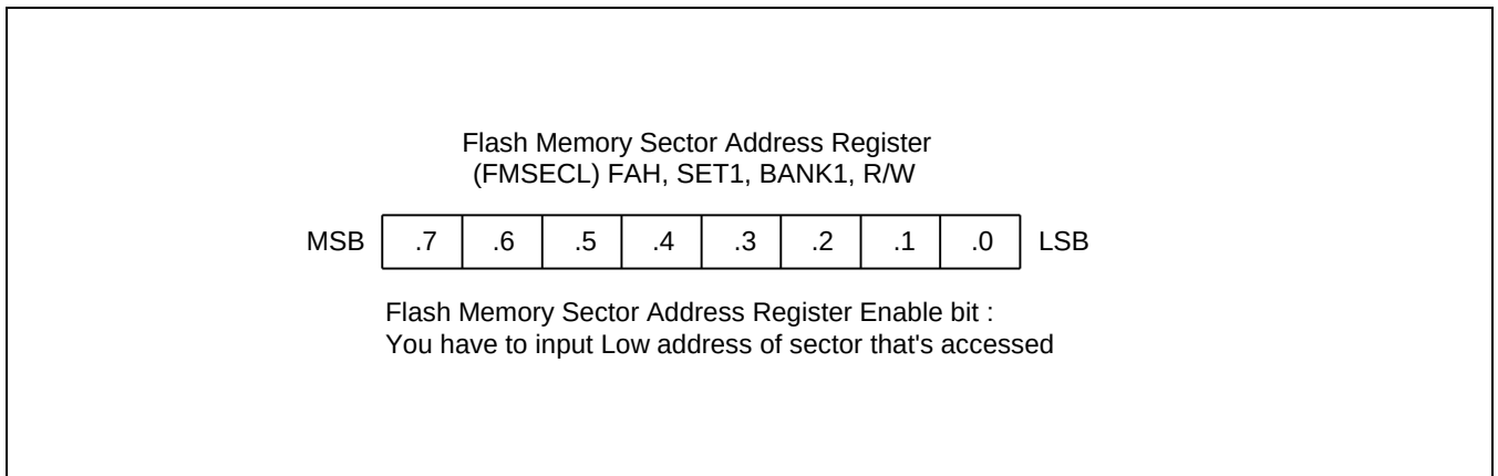
Figure 20-5 Flash Memory Sector Address Register (FMSECL)
