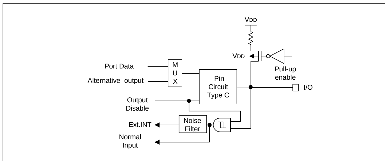
Figure 1-7 Pin Circuit Type D-5 (P1.0–P1.3)
