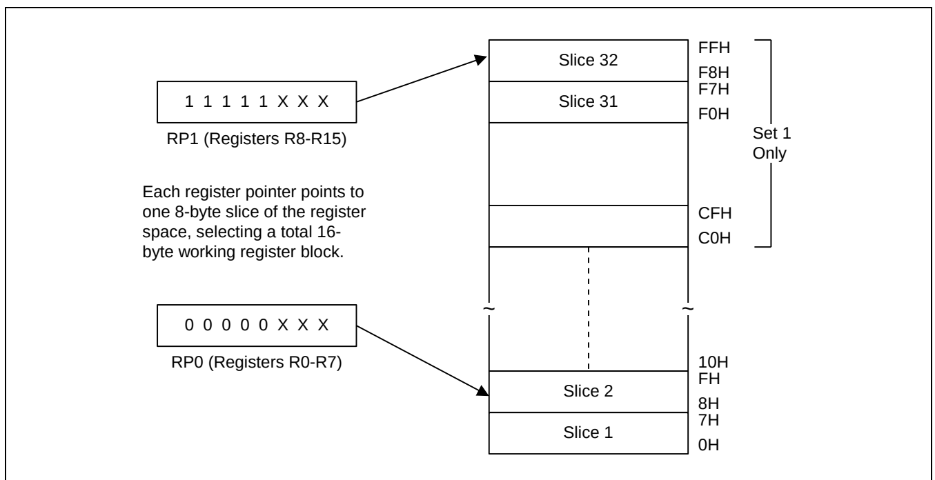
Figure 2-8 8 byte Working Register Areas (Slices)
