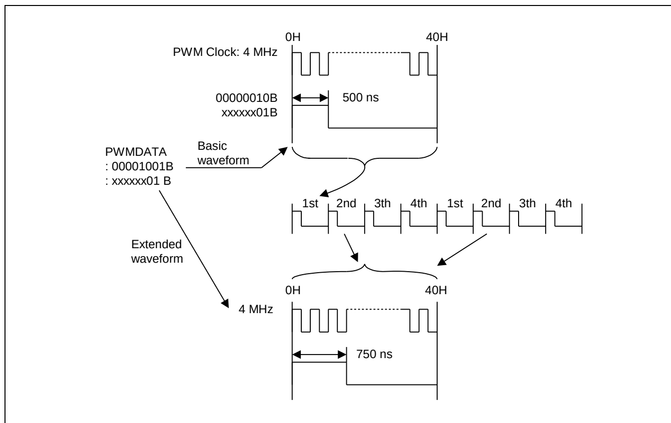
Figure 13-2 10-Bit Extended PWM Waveform
