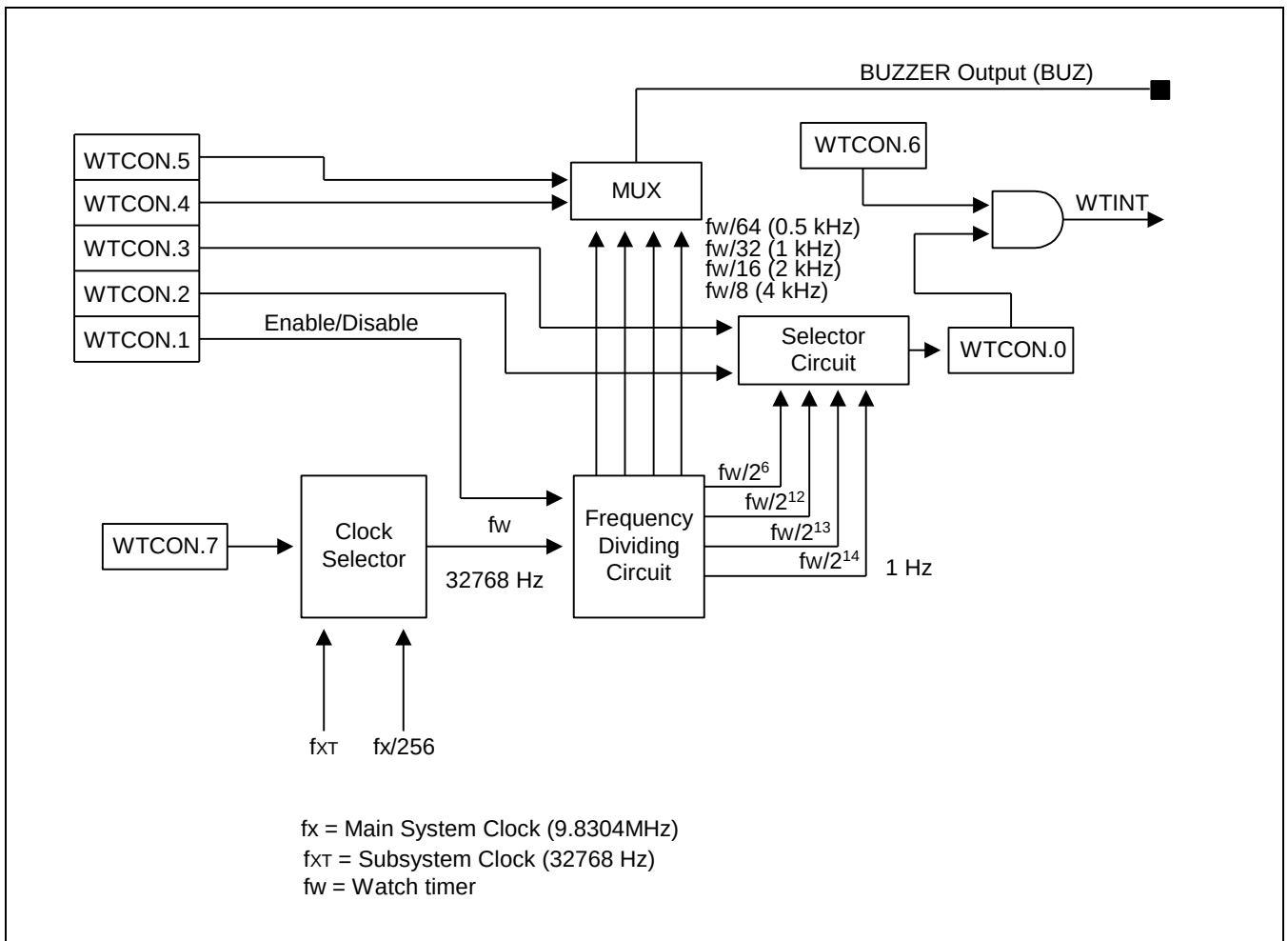
Figure 17-1 Watch Timer Circuit Diagram
