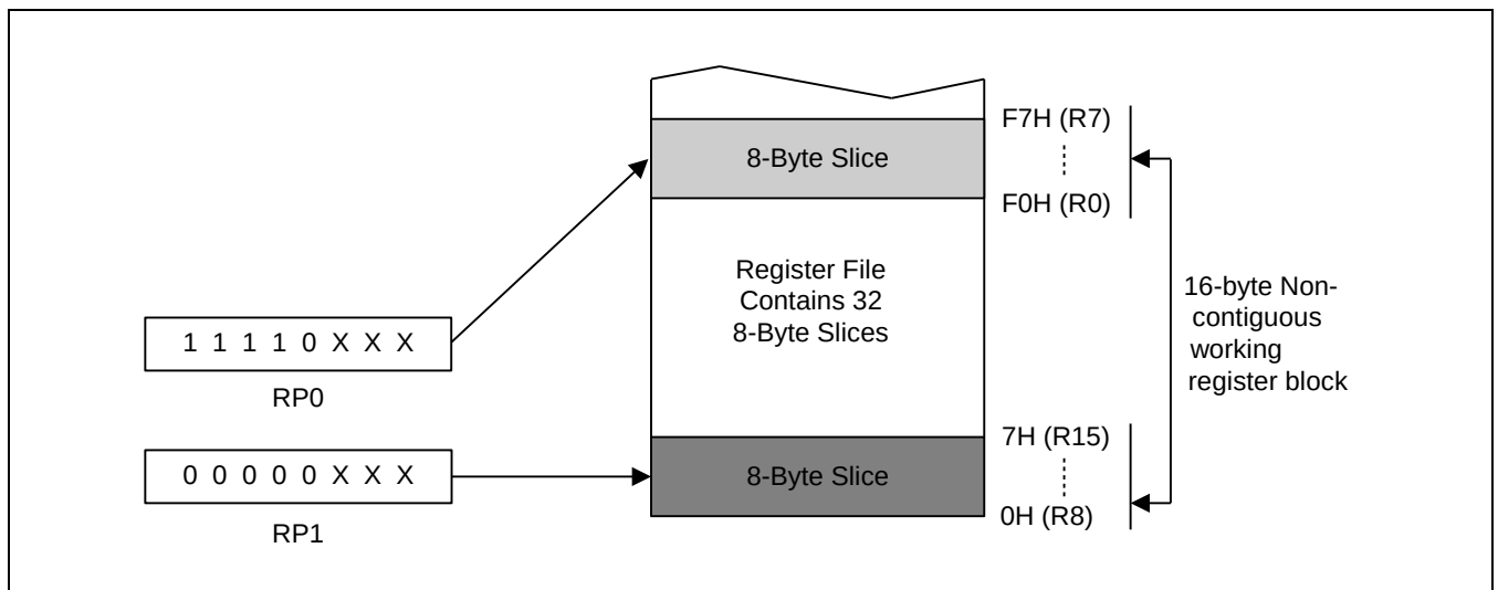
Figure 2-10 Non-Contiguous 16 byte Working Register Block
