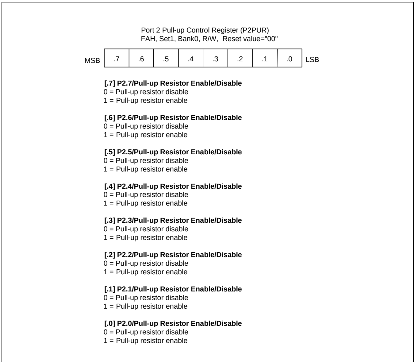
Figure 9-8 Port 2 Pull-up Control Register (P2PUR)
