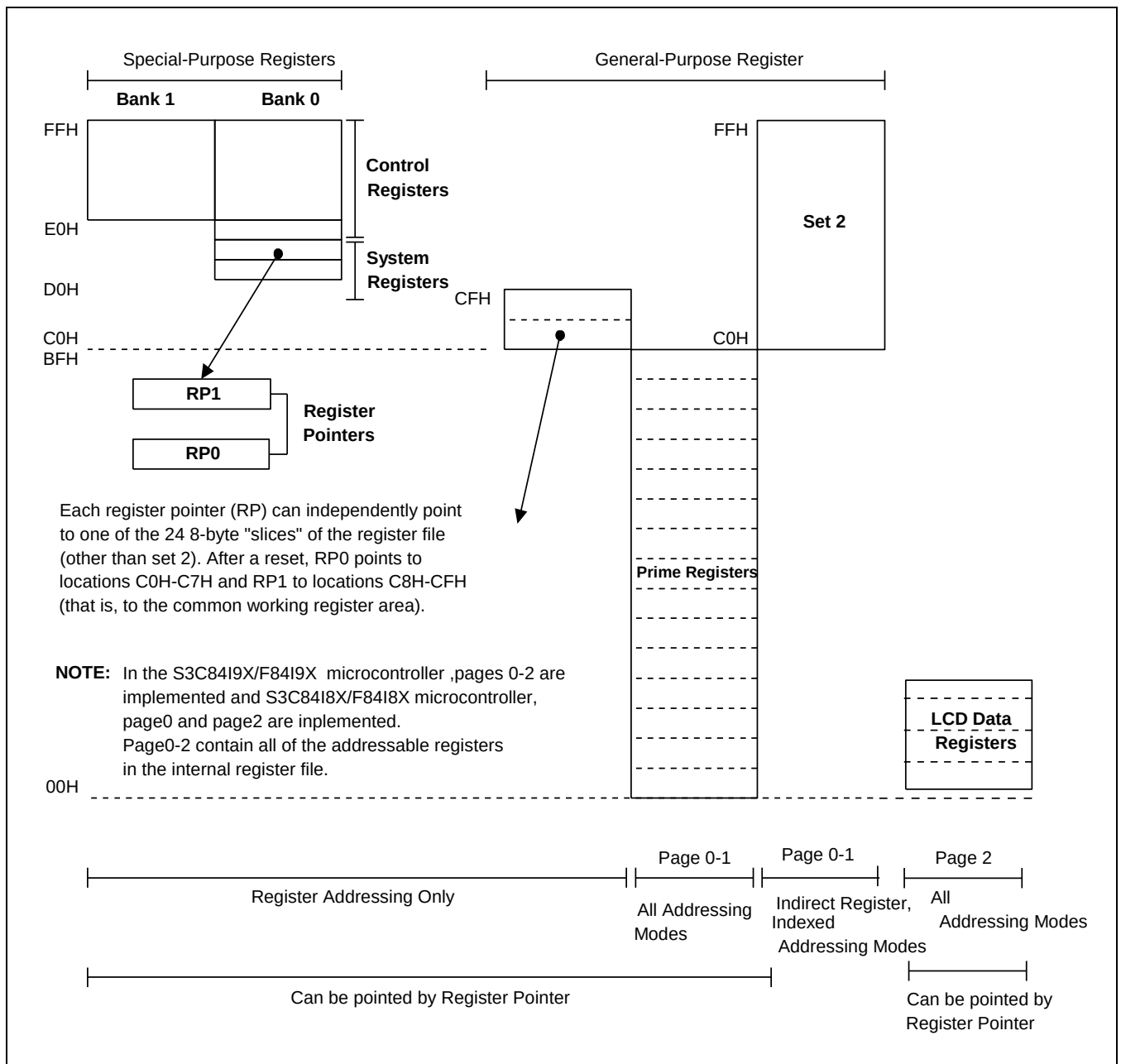
Figure 2-12 Register File Addressing
