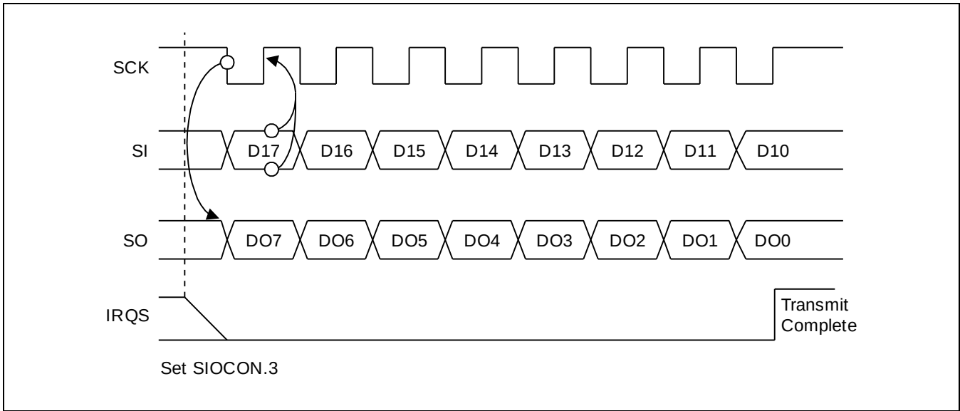
Figure 14-4 Serial I/O Timing in Transmit-Receive Mode (Tx at falling, SIOCON.4 = 0)
