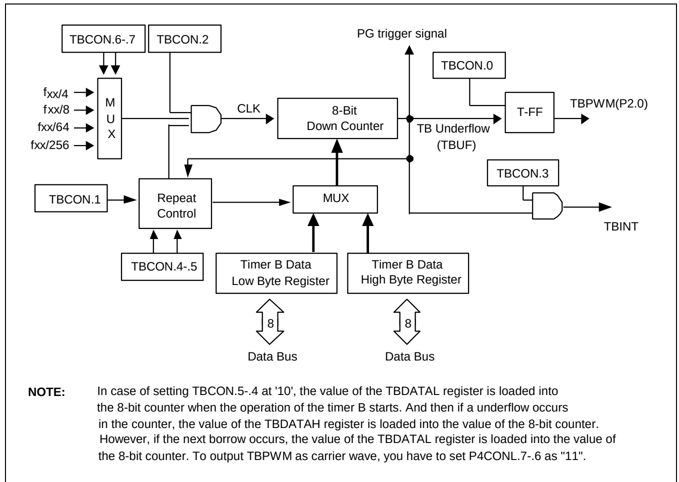
Figure 11-3 Timer B Functional Block Diagram
