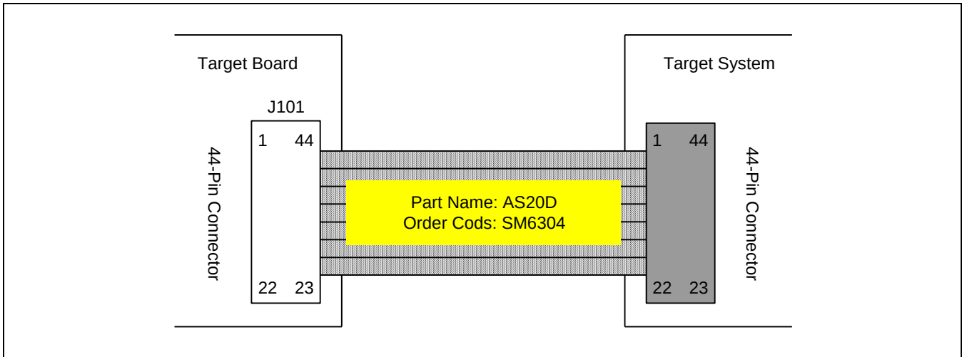
Figure 23-6 TB84I9 Adapter Cable for 44pin Connector Package
