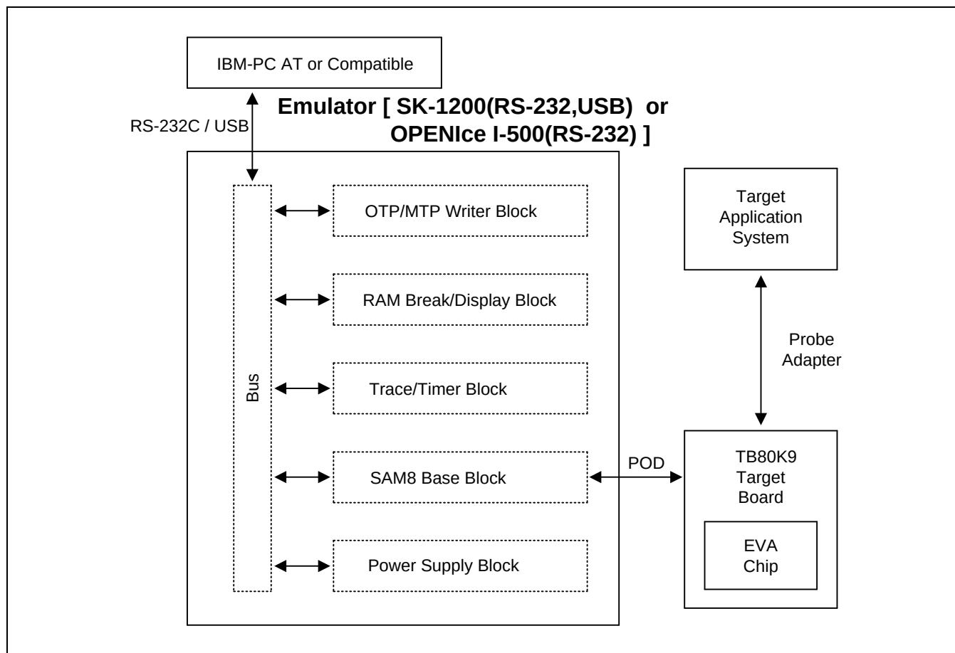
Figure 23-1 Development System Configuration
