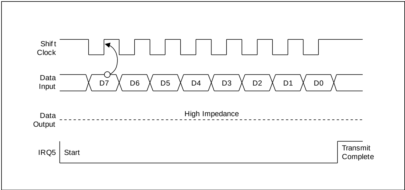
Figure 14-6 Serial I/O Timing in Receive-Only Mode
