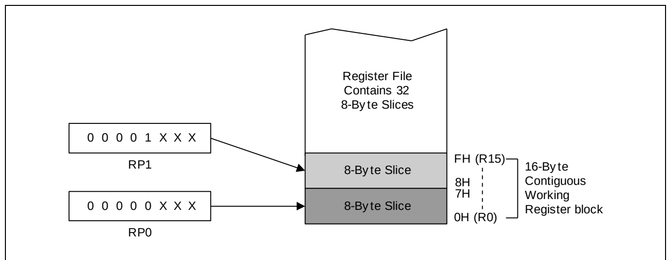
Figure 2-9 Contiguous 16 byte Working Register Block
