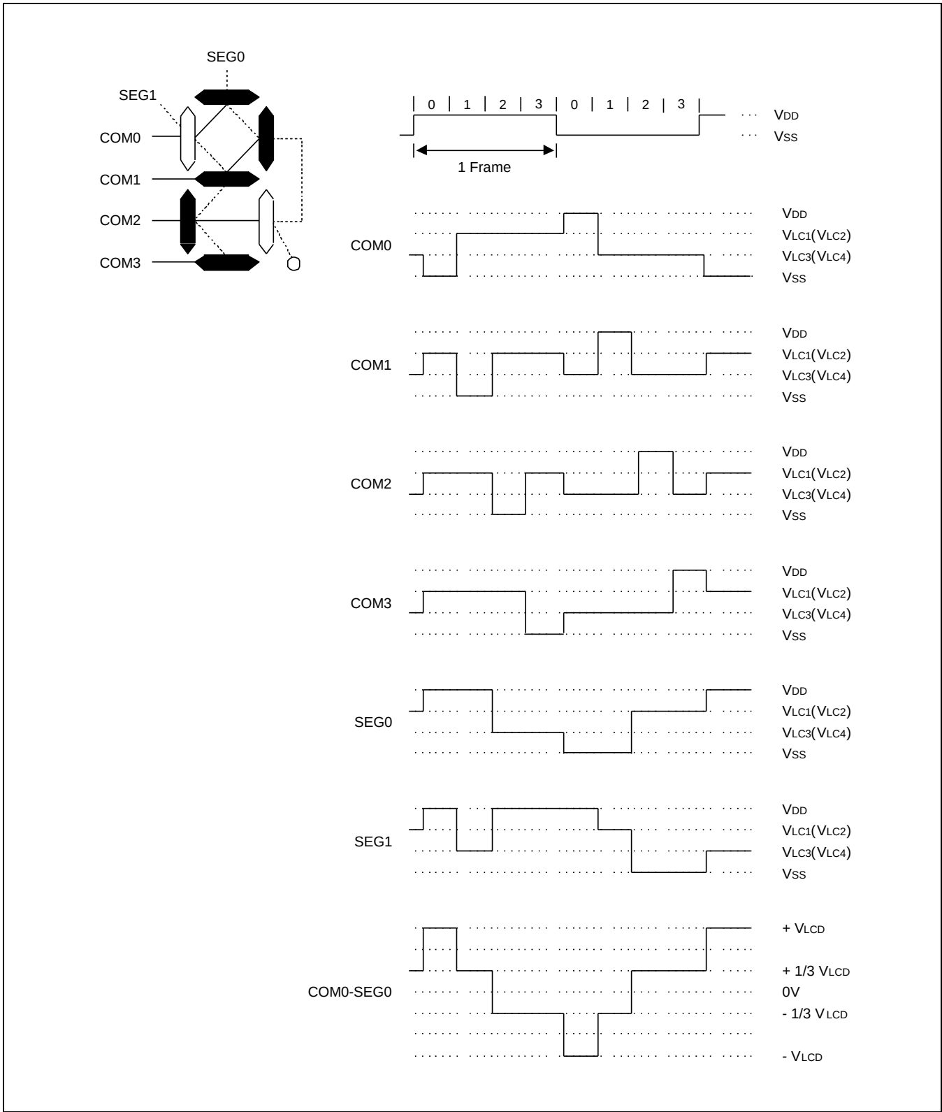
Figure 18-8 LCD Signal Waveforms (1/4 Duty, 1/3 Bias)
