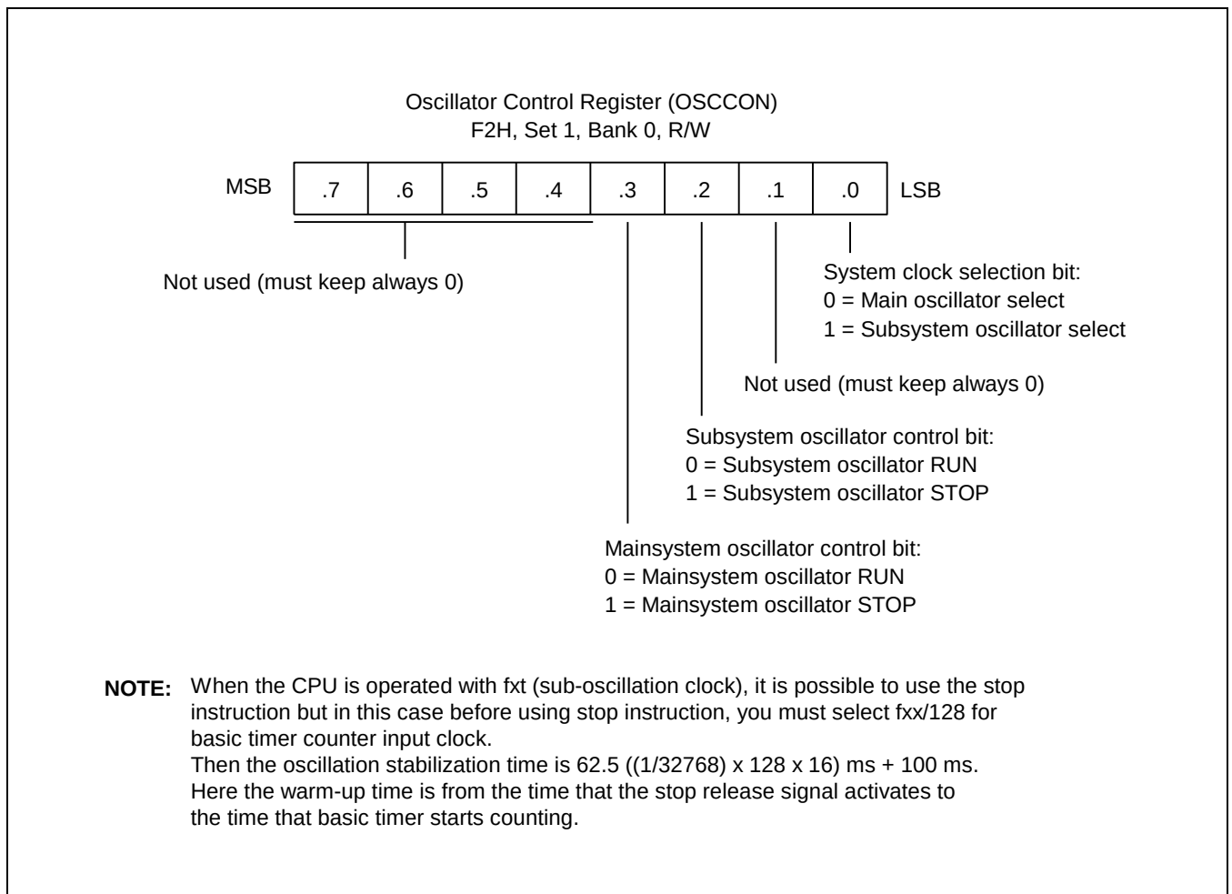
Figure 7-5 Oscillator Control Register (OSCCON)
