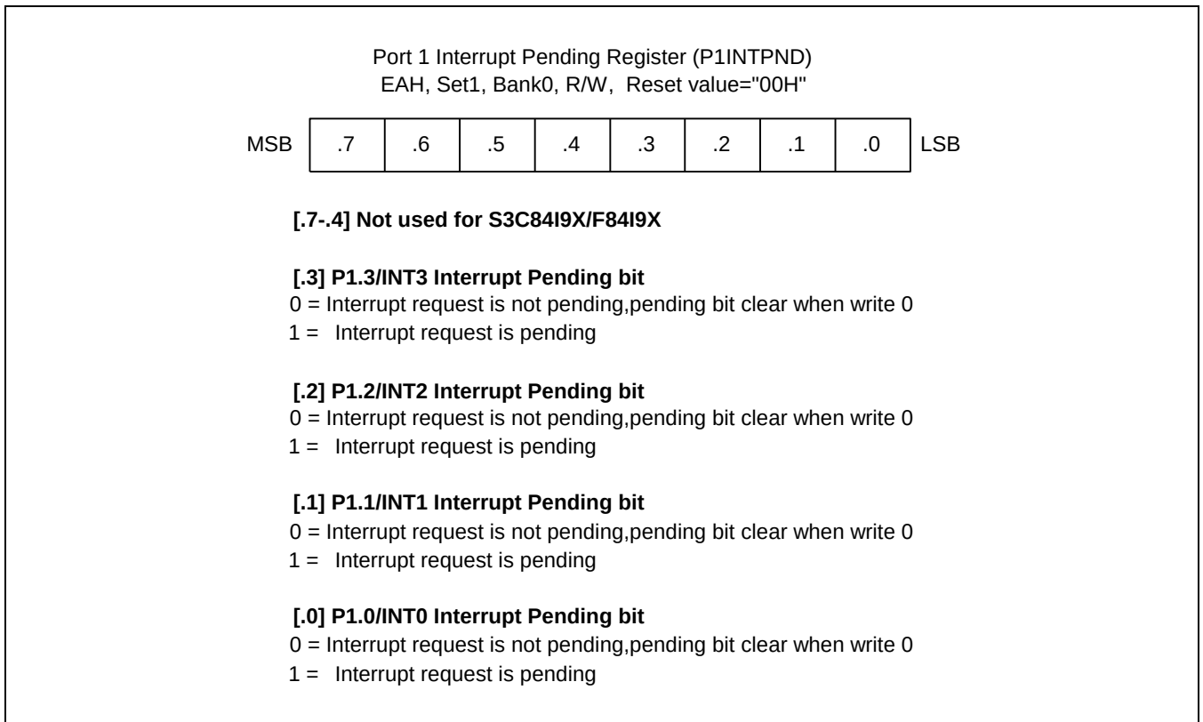
Figure 9-4 Port 1 Interrupt Pending Register (P1INTPND)
