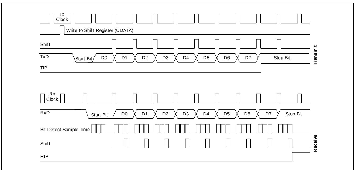
Figure 15-7 Timing Diagram for UART Mode 1 Operation
