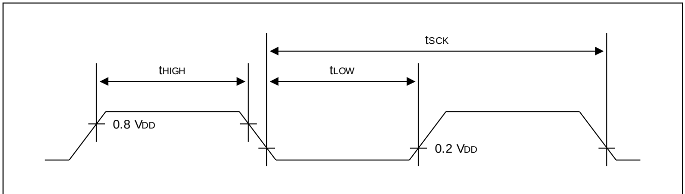
Figure 21-7 Waveform for UART Timing Characteristics
