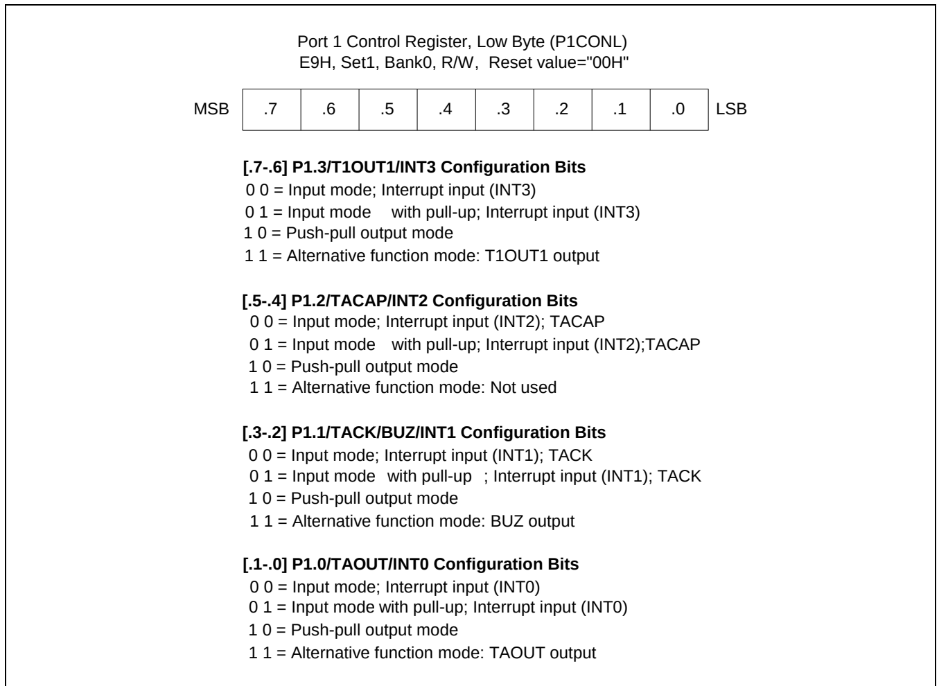
Figure 9-3 Port 1 Low-Byte Control Register (P1CONL)
