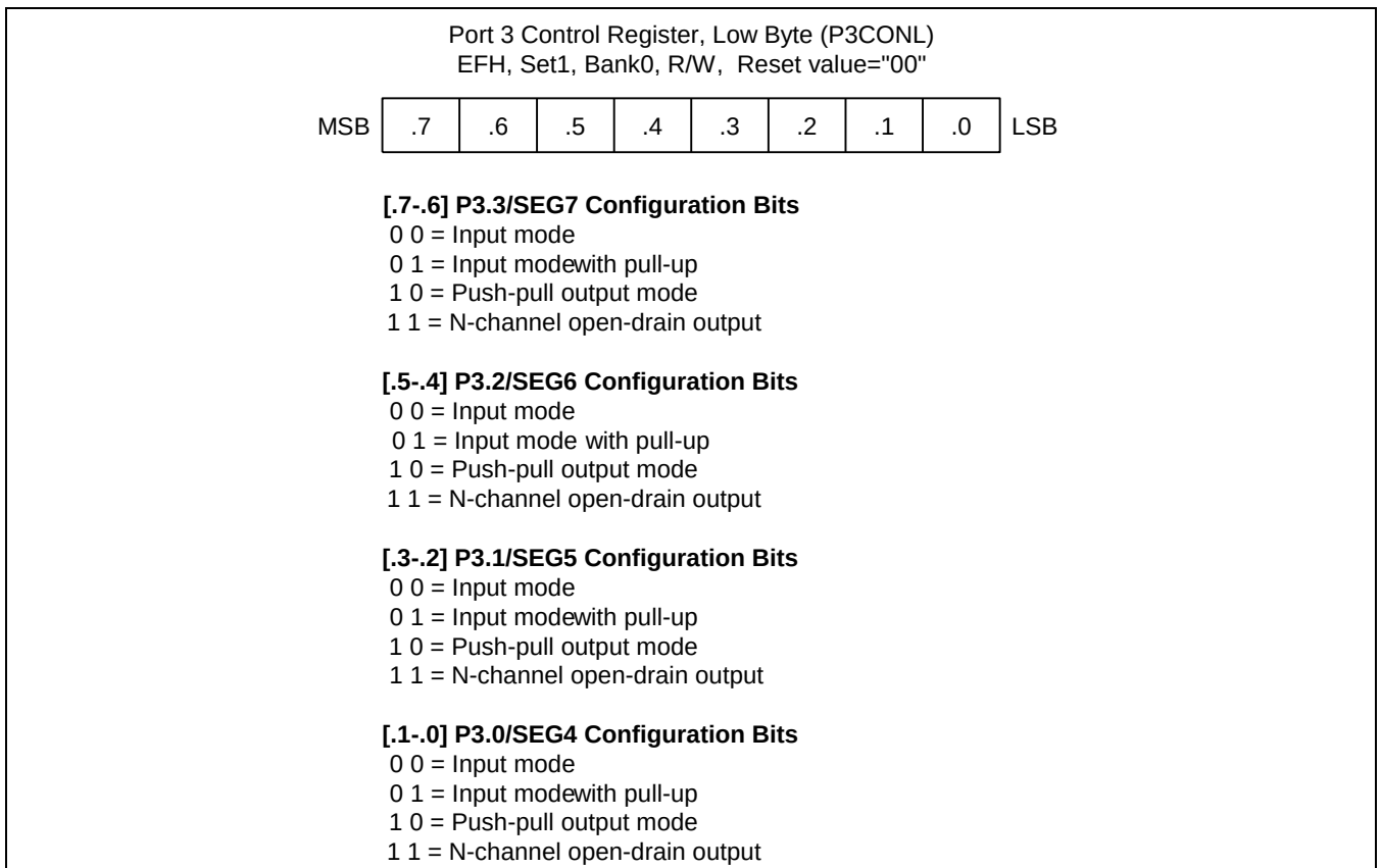
Figure 9-10. Port 3 Low-Byte Control Register (P3CONL)
