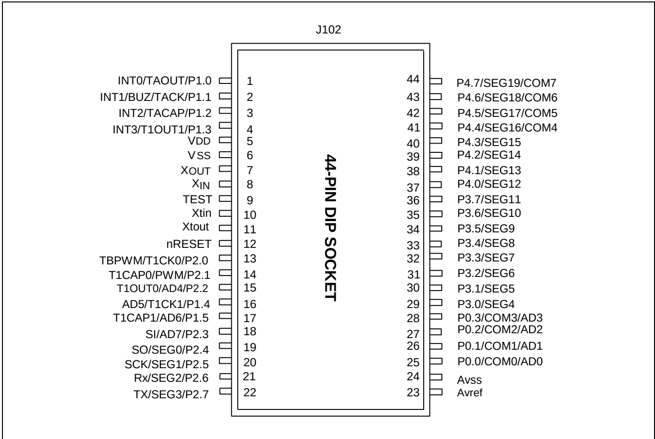
Figure 23-4 44-Pin Connector Pin Assignment for TB84I9
