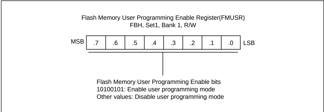
Figure 20-2 Flash Memory User Programming Enable Register (FMUSR)
