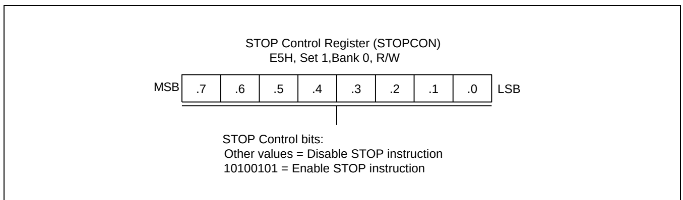
Figure 7-6 STOP Control Register (STOPCON)
