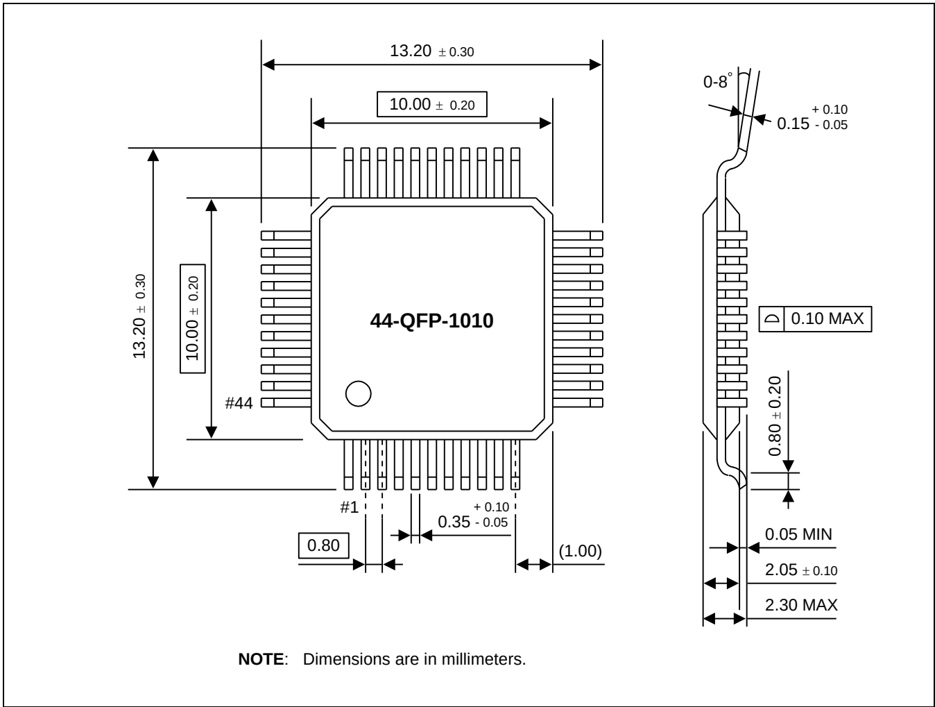
Figure 22-2 44-QFP-1010 Package Dimensions
