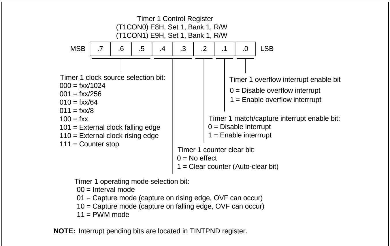
Figure 12-1 Timer 1 (0, 1) Control Register (T1CON0, T1CON1)
