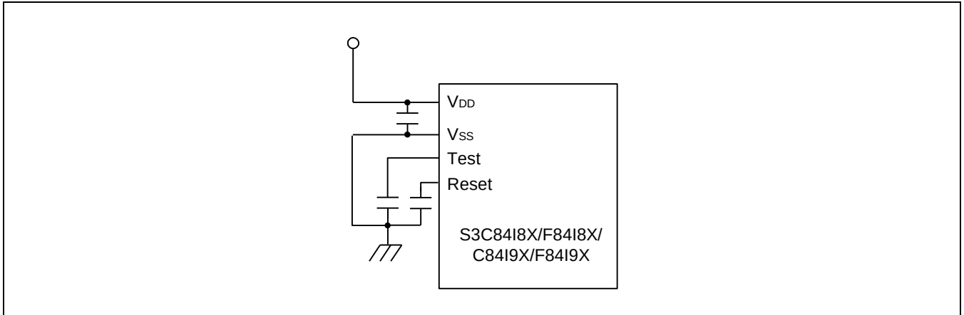
Figure 21-9 The Circuit Diagram to Improve EFT Characteristics
