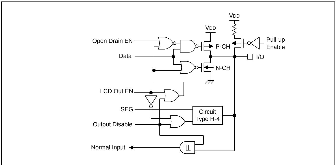
Figure 1-12 Pin Circuit Type H-17 (P3.0–P3.7, P4.0–P4.)
