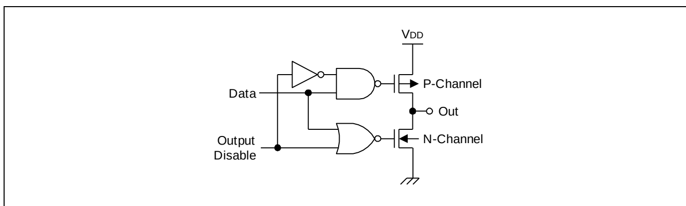
Figure 1-5 Pin Circuit Type C
