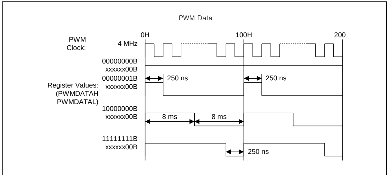
Figure 13-1 10-Bit PWM Basic Waveform
