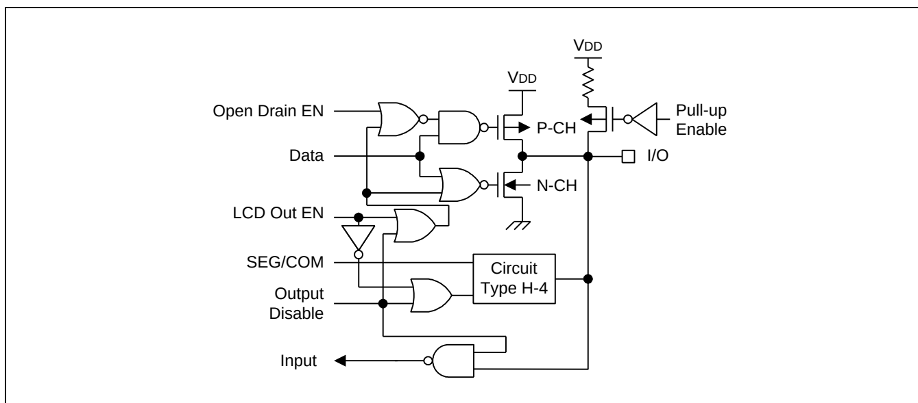
Figure 1-10 Pin Circuit Type H-14 (P4.4–P4.7)
