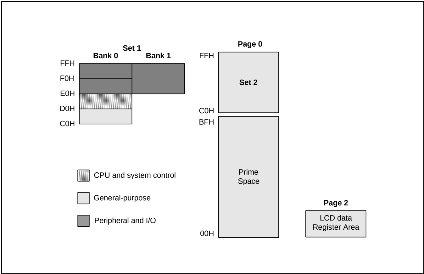
Figure 2-7 Set 1, Set 2, Prime Area Register (S3C84I8X/F84I8X)
