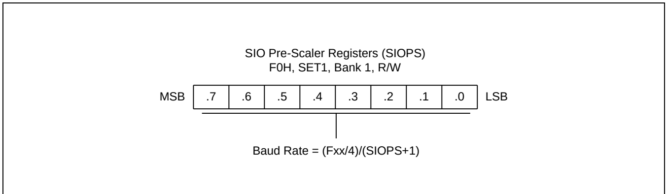
Figure 14-2 SIO Pre-Scaler Register (SIOPS)
