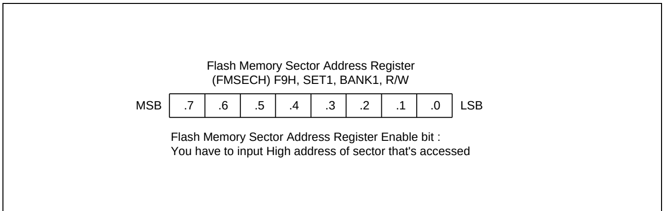
Figure 20-4 Flash Memory Sector Address Register (FMSECH)
