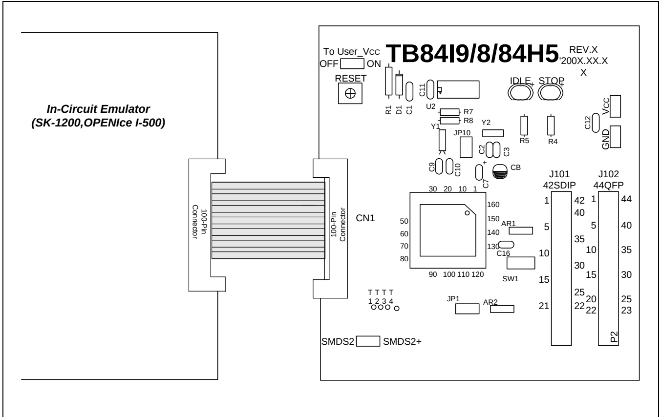
Figure 23-2 S3F84I9X/S3F84I8X Target Board Configuration
