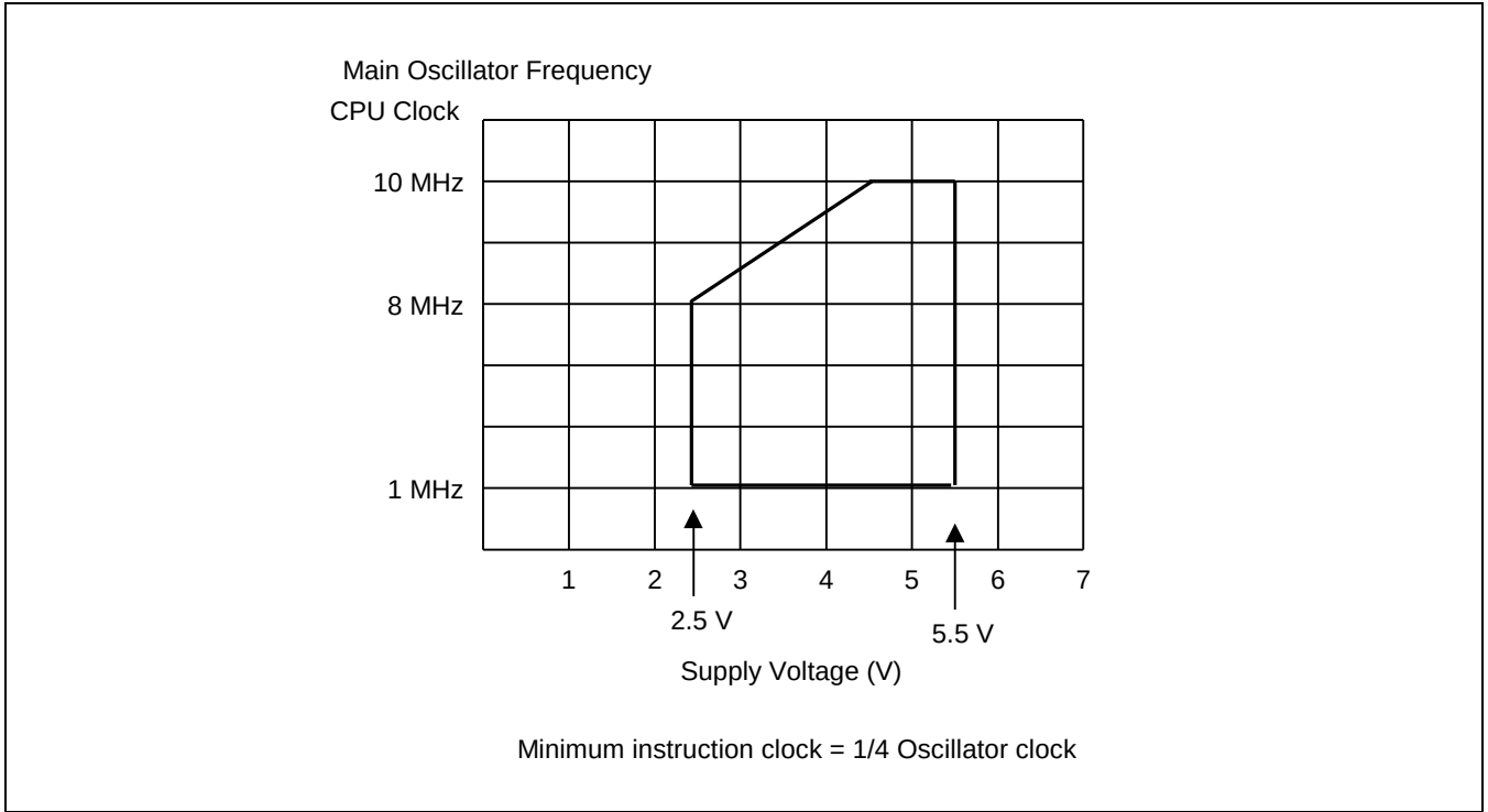
Figure 21-8 Operating Voltage Range
