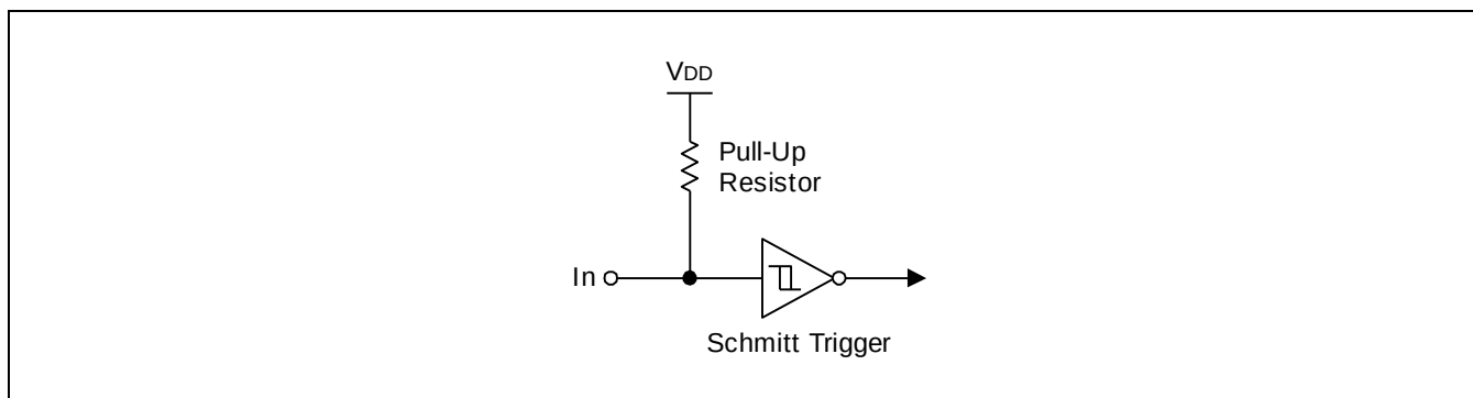
Figure 1-4 Pin Circuit Type B (nRESET)
