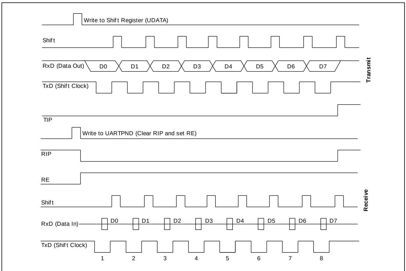
Figure 15-6 Timing Diagram for UART Mode 0 Operation
