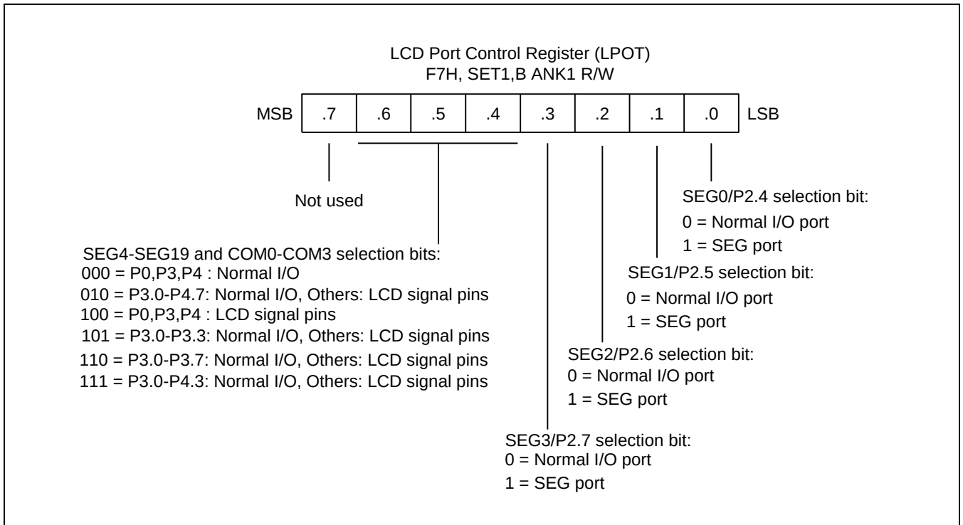
Figure 18-5 LCD Port Control Register
