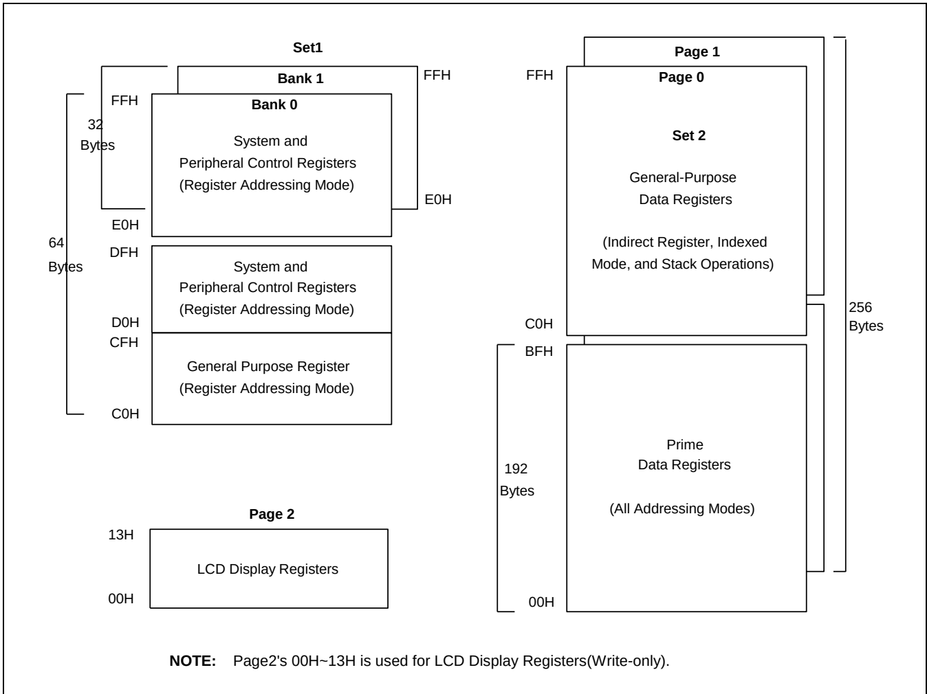
Figure 2-3 Internal Register File Organization of S3F84I9X/C84I9X
