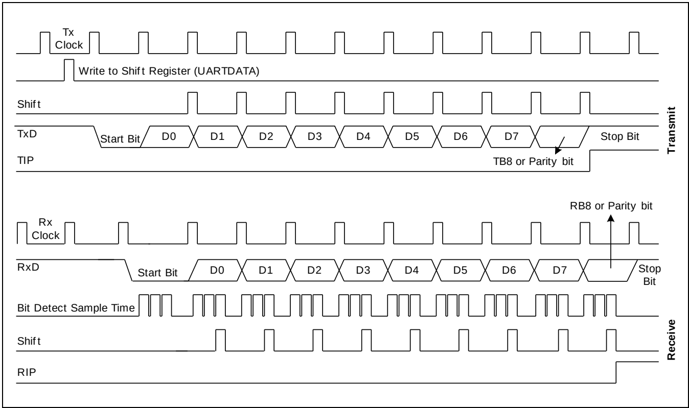
Figure 15-8 Timing Diagram for UART Mode 2 Operation
