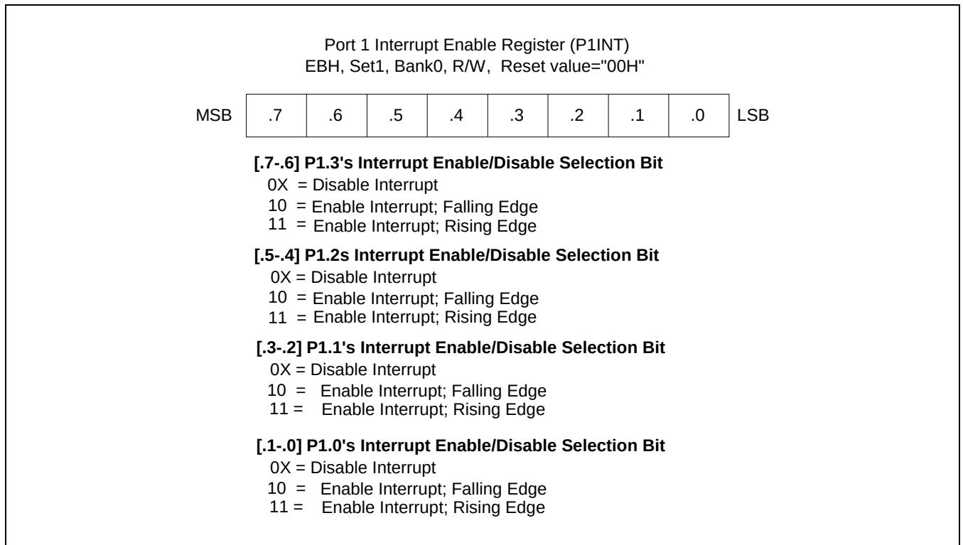
Figure 9-5 Port 1 Interrupt Enable Register (P1INT)
