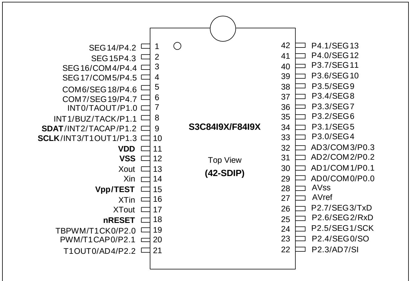
Figure 1-3 S3C84I9X/F84I9X Pin Assignment (42-pin SDIP)
