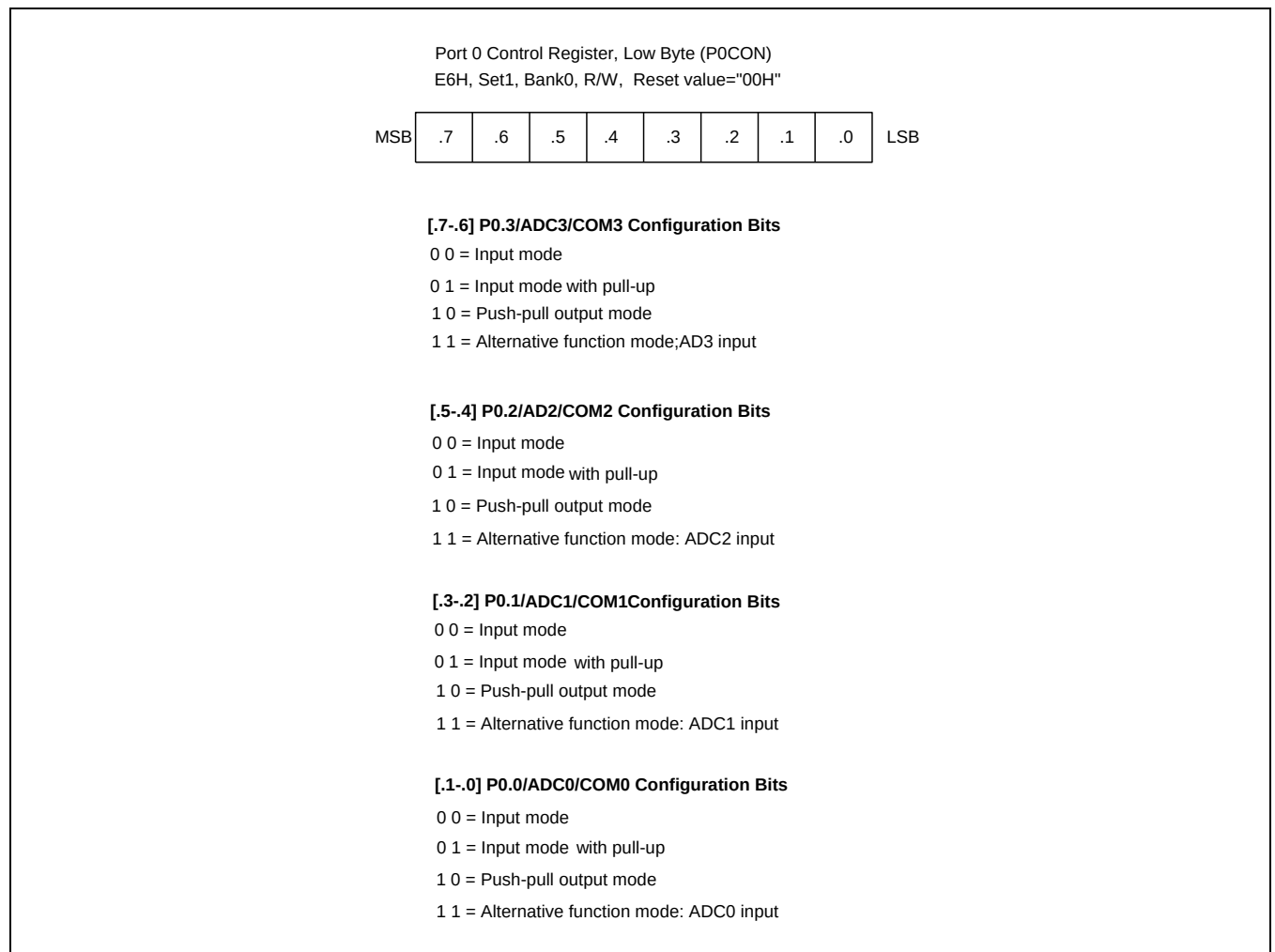
Figure 9-1 Port 0 Low Byte Control Register (P0CON)
