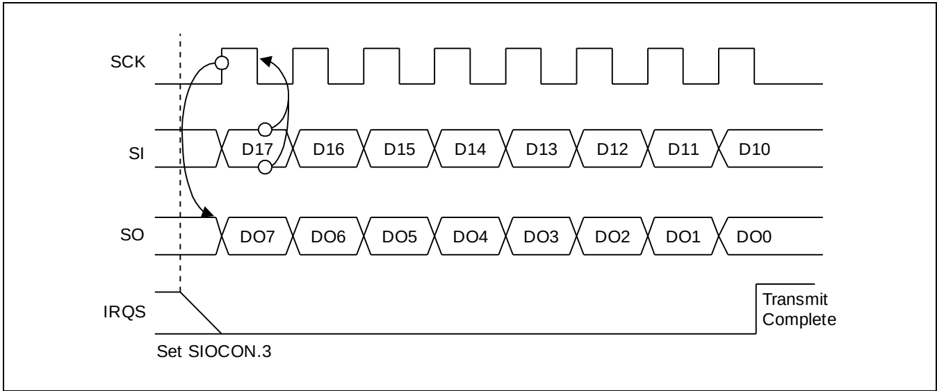
Figure 14-5 Serial I/O Timing in Transmit-Receive Mode (Tx at rising, SIOCON.4 = 1)
