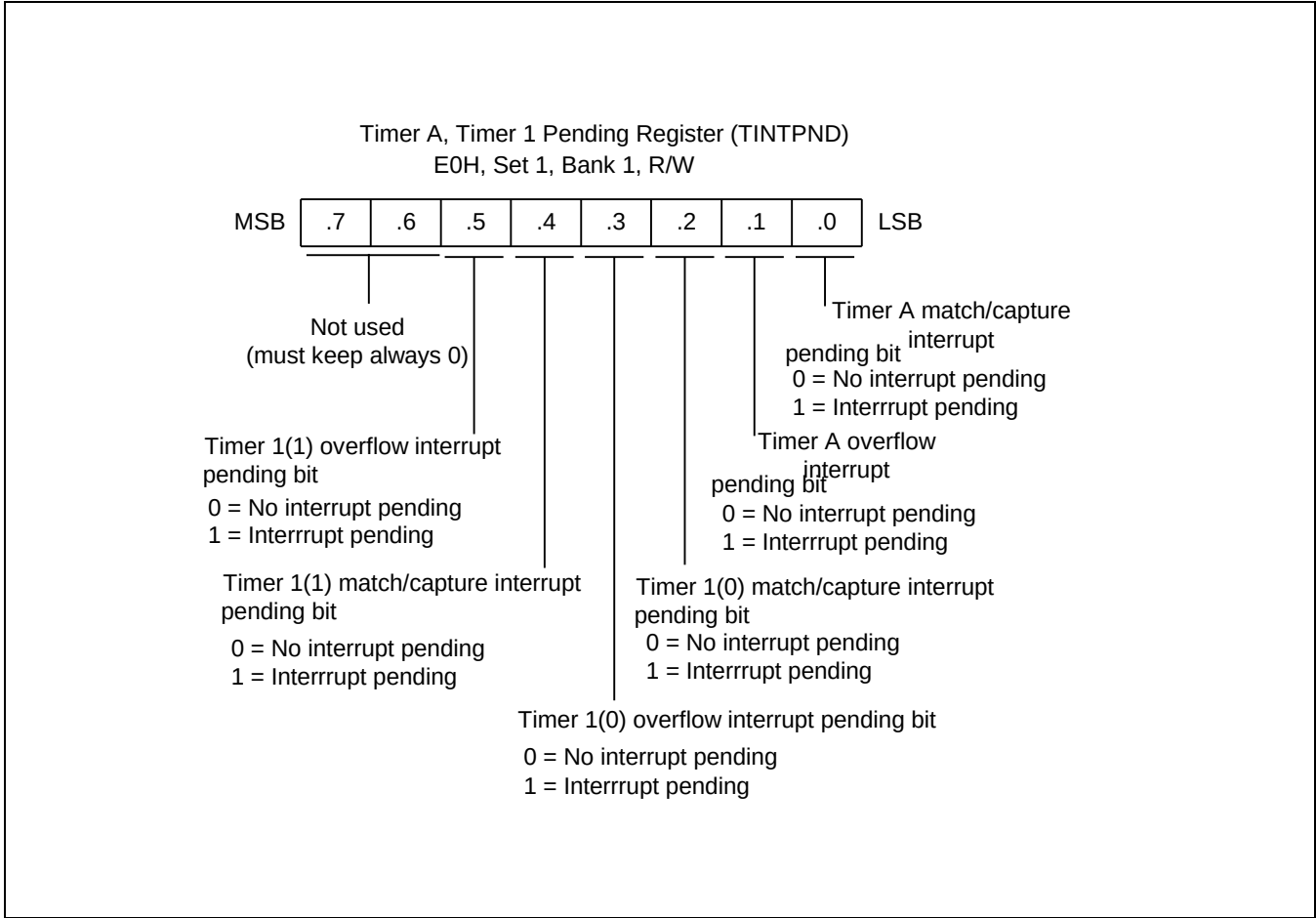
Figure 12-2 Timer A, Timer 1 (0, 1) Pending Register (TINTPND)
