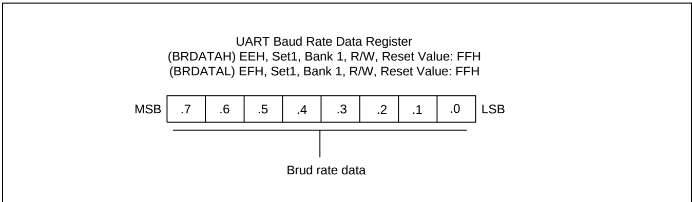
Figure 15-4 UART Baud Rate Data Register (BRDATAH, BRDATAL)
