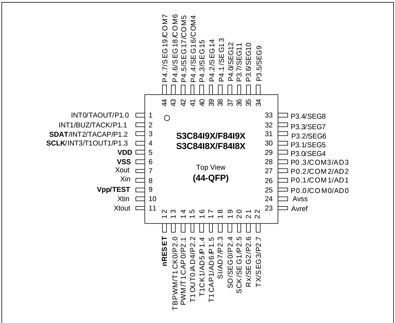
Figure 1-2 S3C84I8X/F84I8X/C84I9X/F84I9X Pin Assignment (44-pin QFP)
