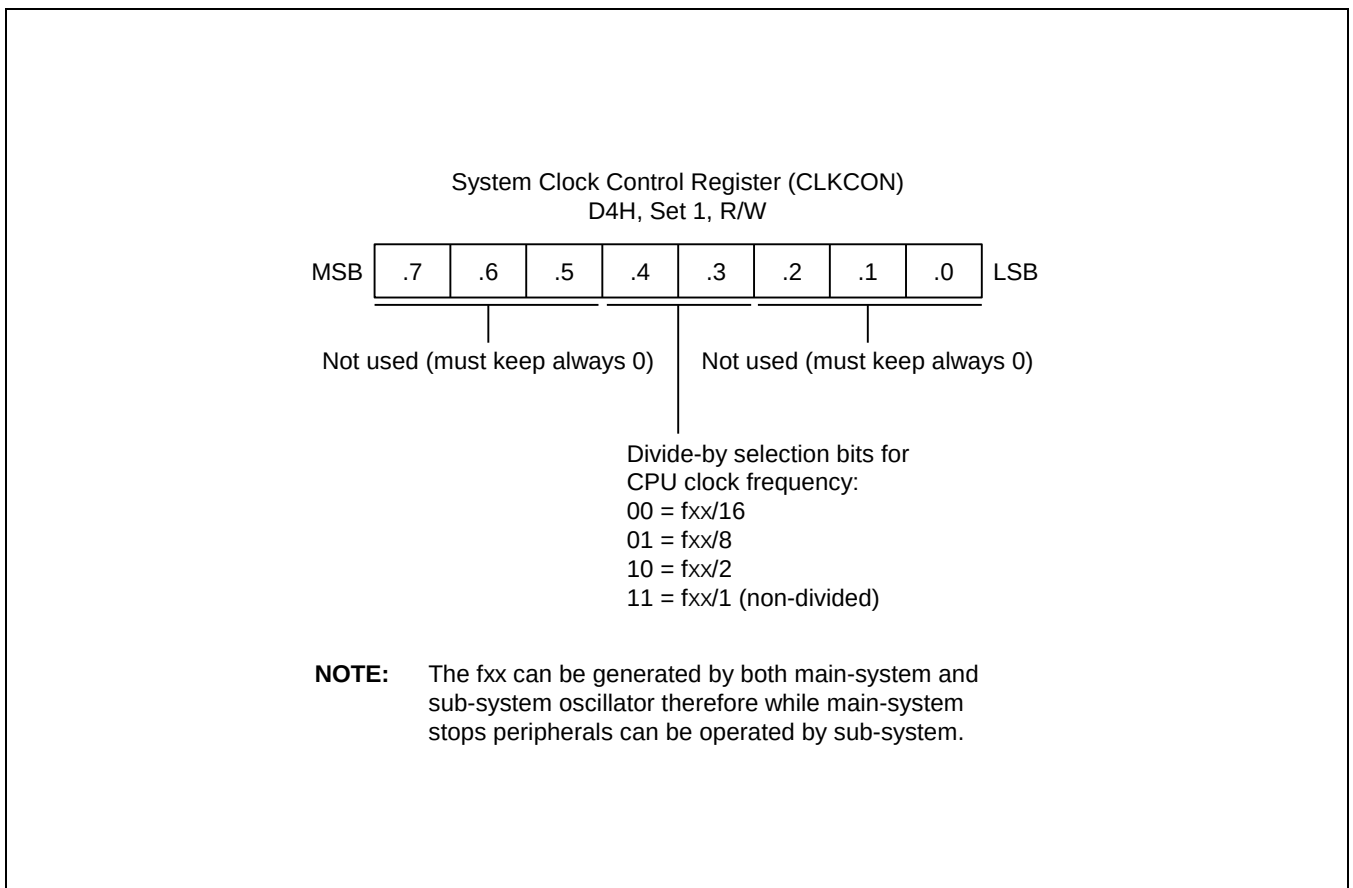
Figure 7-4 System Clock Control Register (CLKCON)
