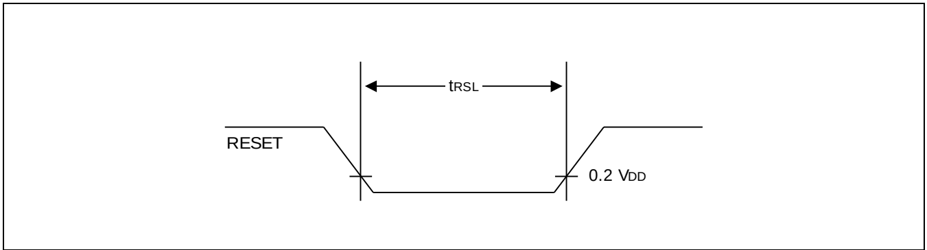
Figure 21-2 Input Timing for nRESET
