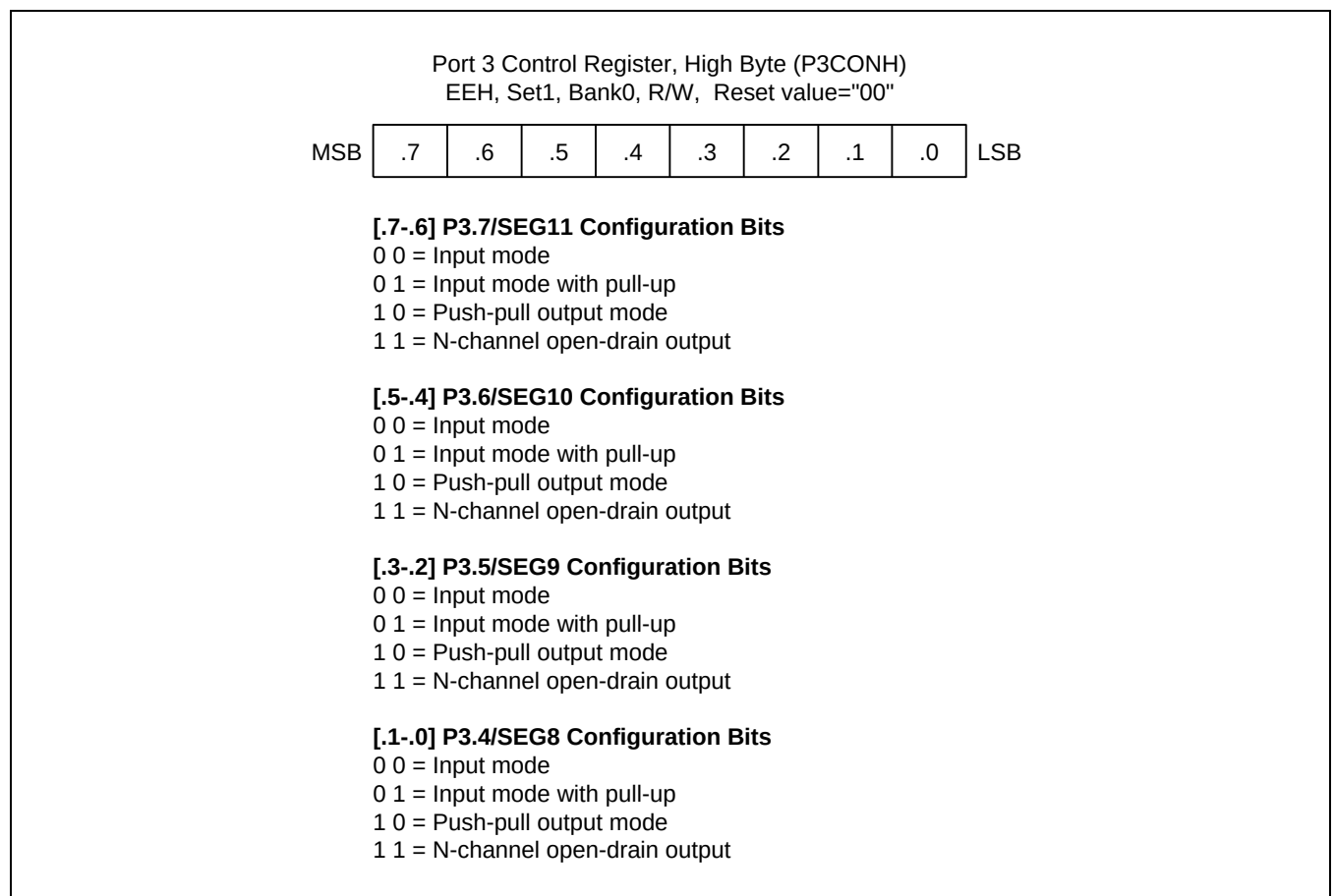
Figure 9-9 Port 3 High-Byte Control Register (P3CONH)
