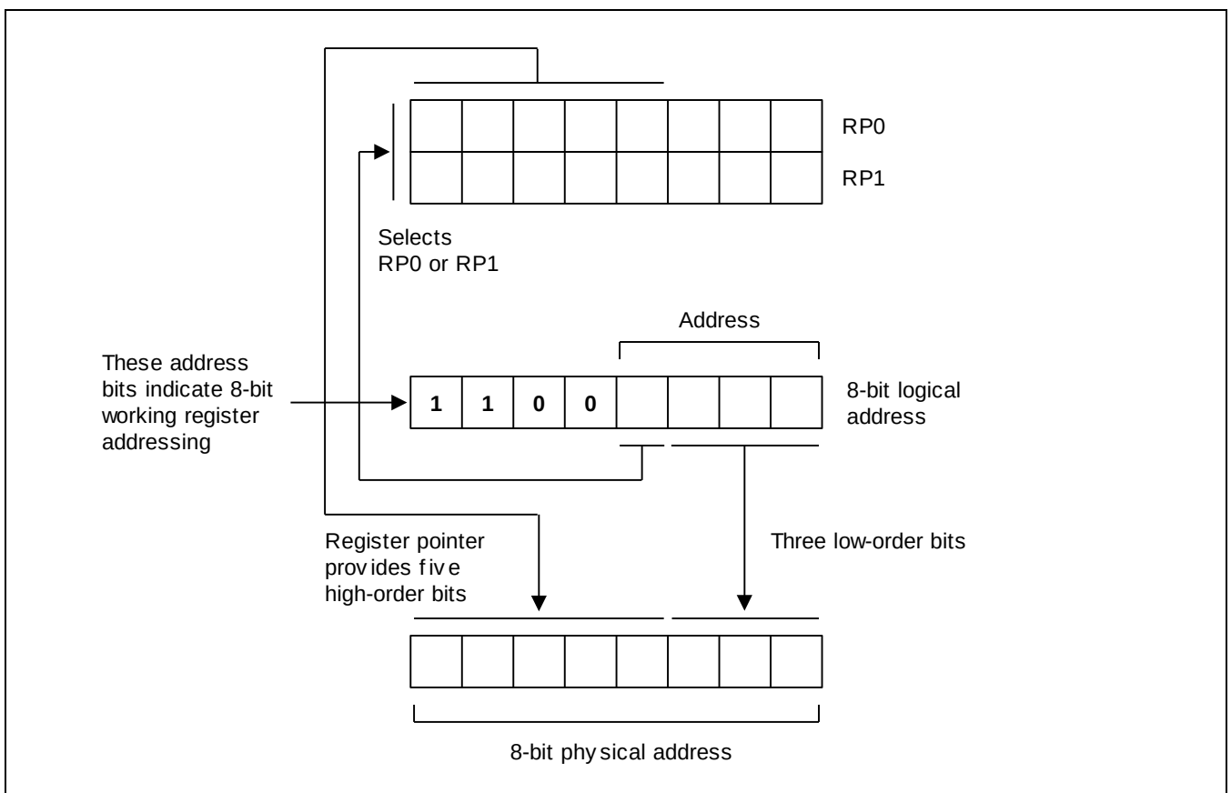
Figure 2-16 8-bit Working Register Addressing
