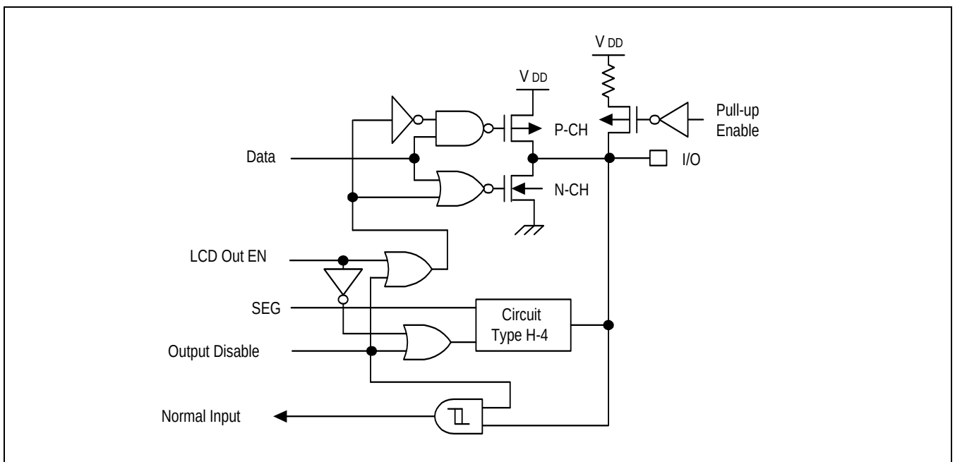
Figure 1-13 Pin Circuit Type H-18 (2.4–P2.7)
