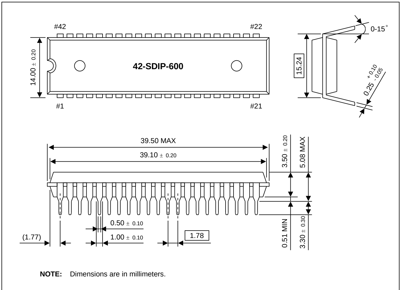
Figure 22-1 42-SDIP-600 Package Dimensions
