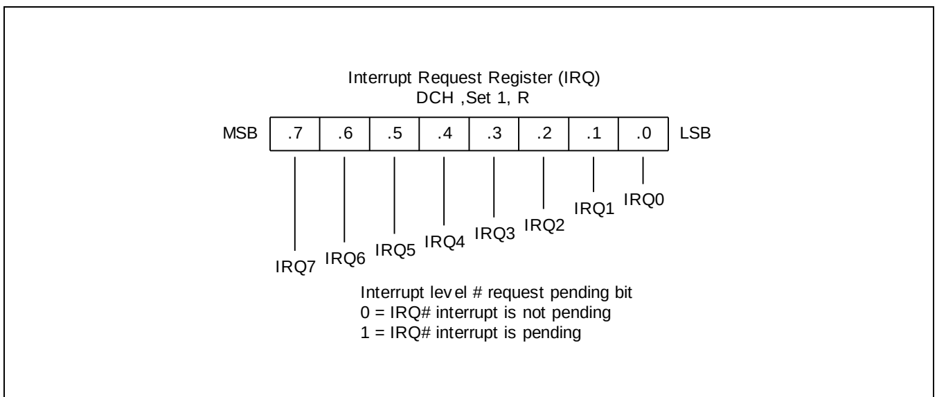
Figure 5-9 Interrupt Request Register (IRQ)
