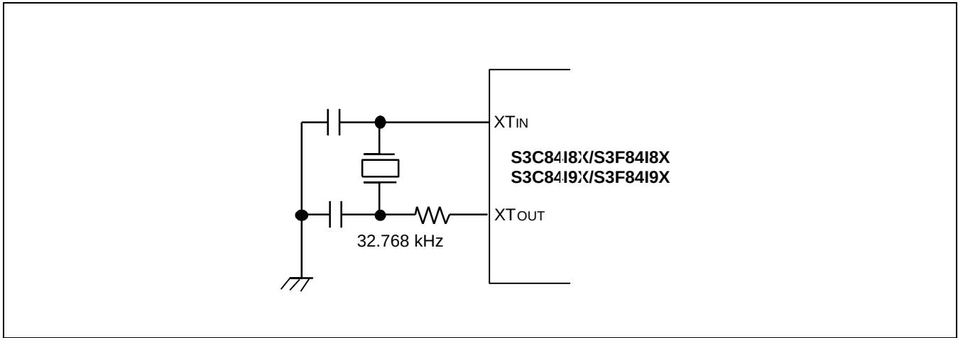
Figure 7-2 Sub-System Oscillator Circuit (Crystal Oscillator)
