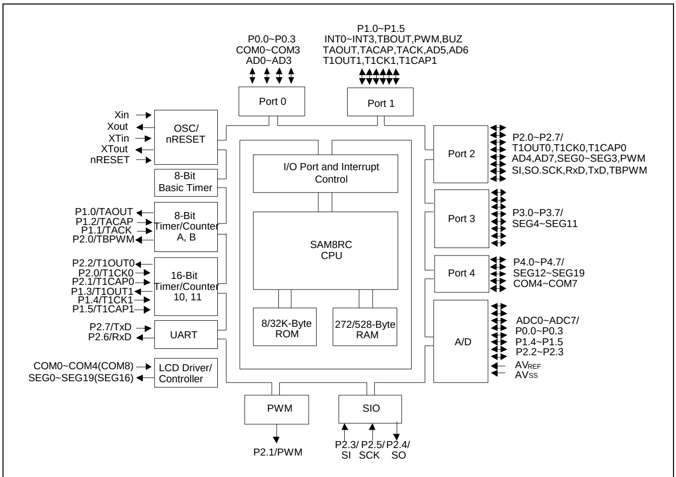
Figure 1-1 S3C84I8/F84I8/C84I9/F84I9 Block Diagram
