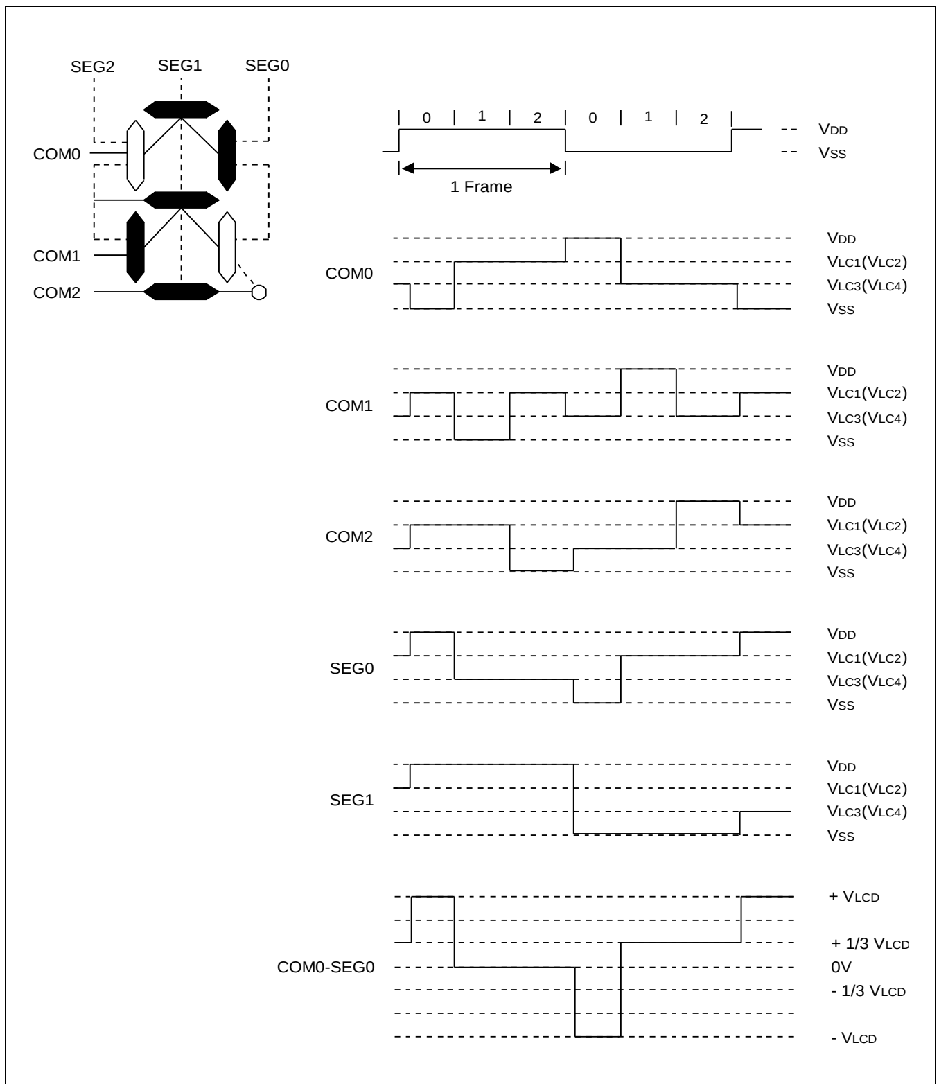
Figure 18-9 LCD Signal Waveforms (1/3 Duty, 1/3 Bias)
