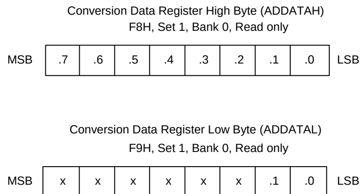
Figure 16-2 A/D Converter Data Register (ADDATAH, ADDATAL)
