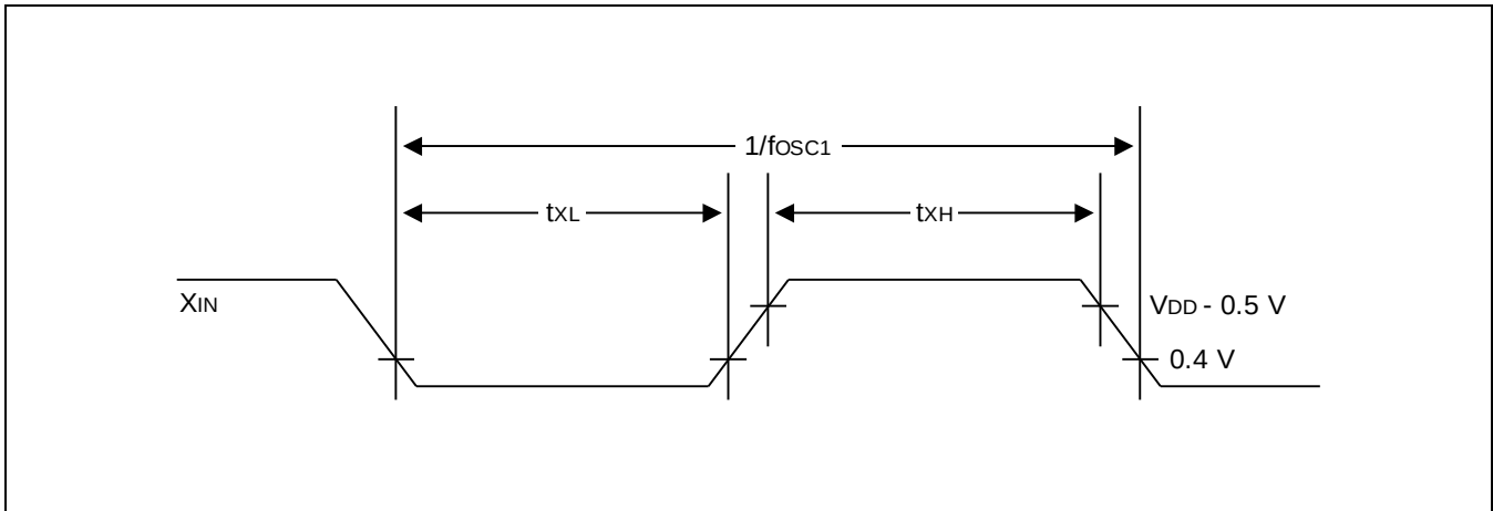
Figure 21-3 Clock Timing Measurement at XIN
