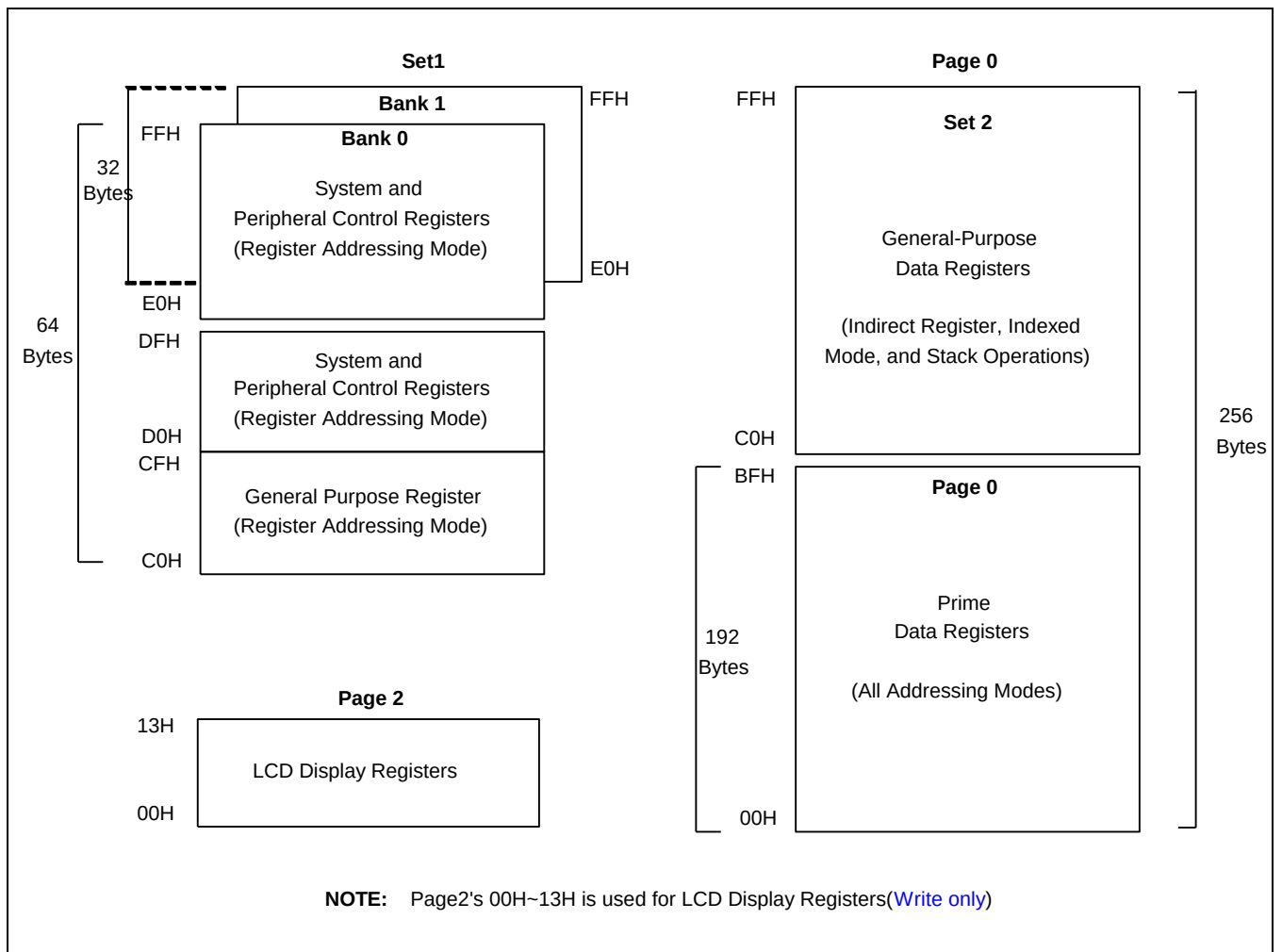
Figure 2-4. Internal Register File Organization of S3F84I8X/C84I8X
