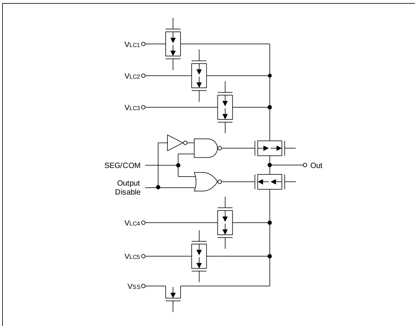
Figure 1-9 Pin Circuit Type H-4
