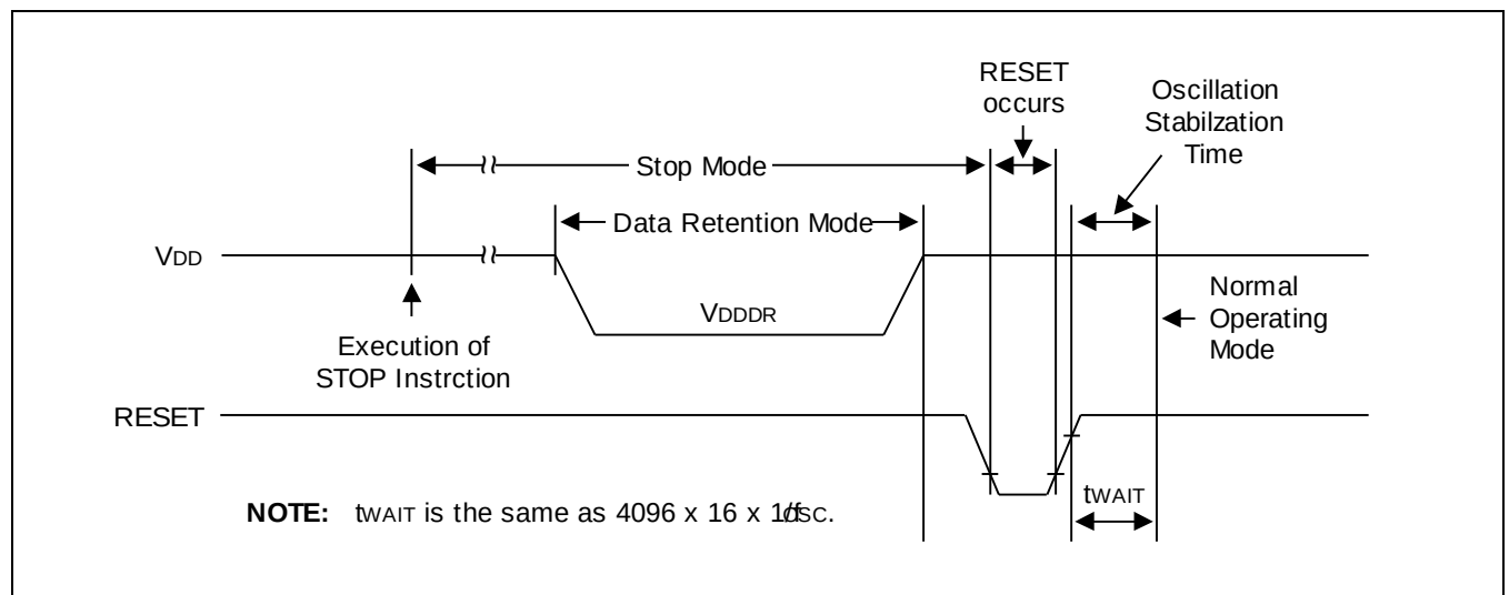
Figure 21-4 Stop Mode Release Timing initiated by RESET
