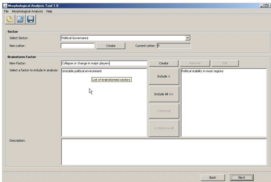
Figure 5: Assigning Symbolic Name & Selecting Factors
