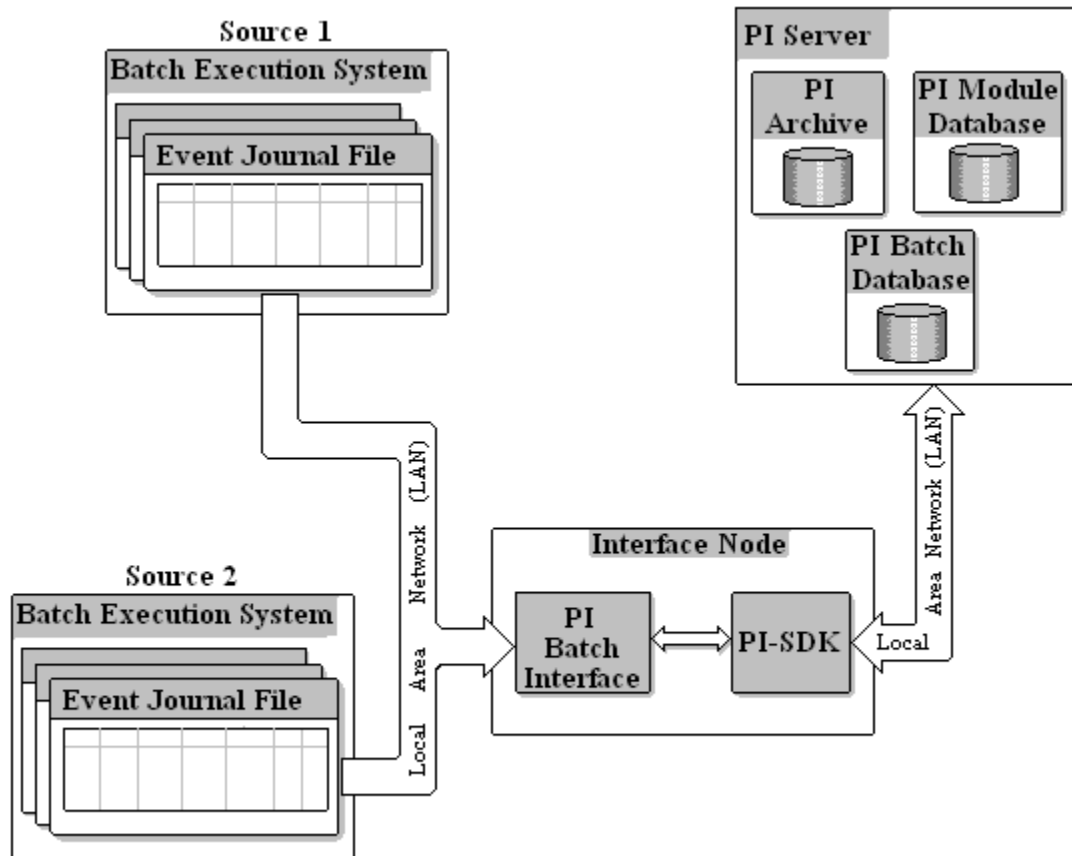
Figure 1. Schematic of Recommended Hardware and Software Configuration for Batch interface with Event Files as sources.
