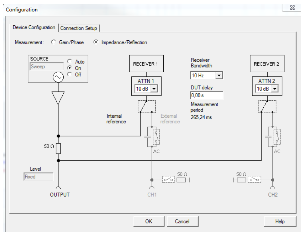
Figure 12: Standard input impedance measurement - configuration window
