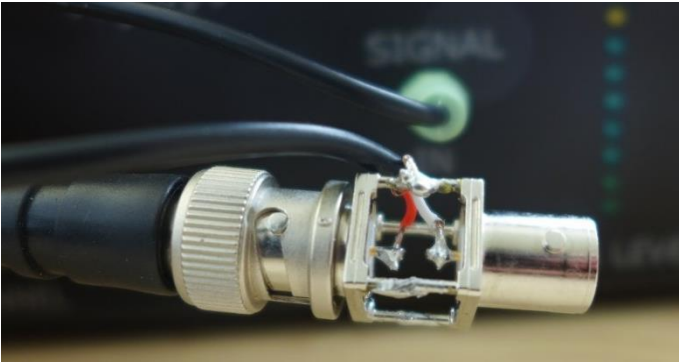
Figure 7: Audio connector to BNC connector
