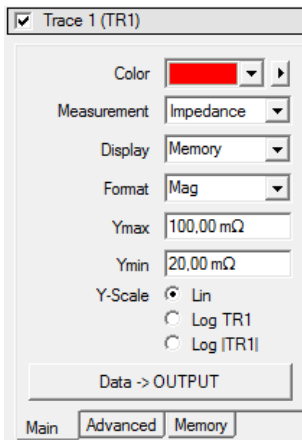
Figure 20: Output impedance measurement - trace 1 settings
