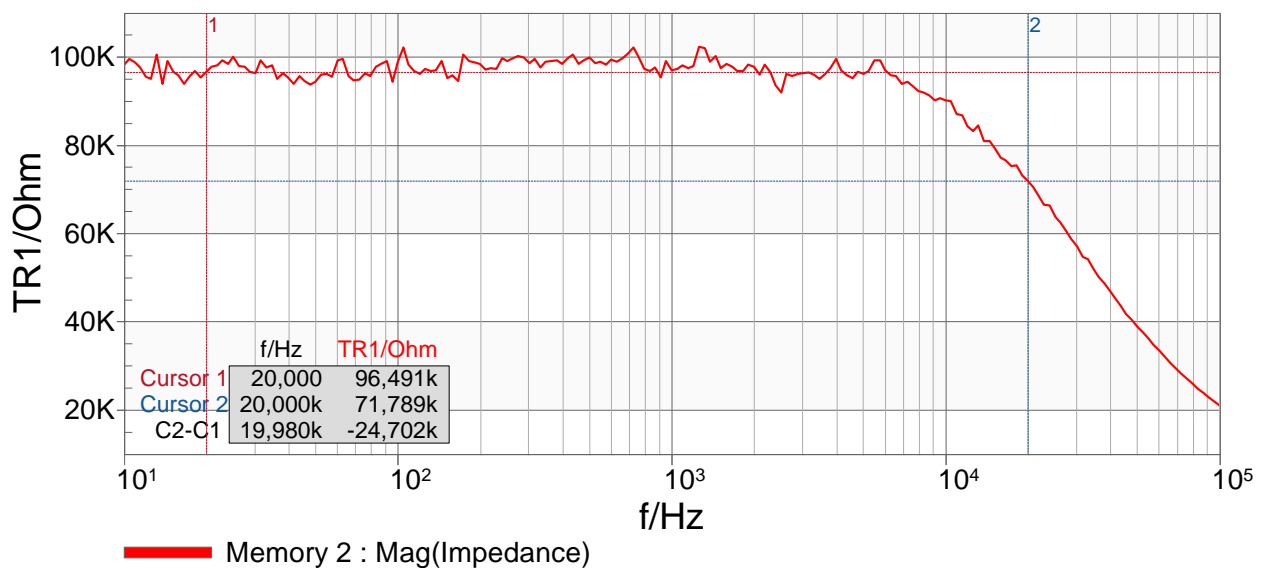
Figure 15: Standard input impedance measurement - frequency sweep
