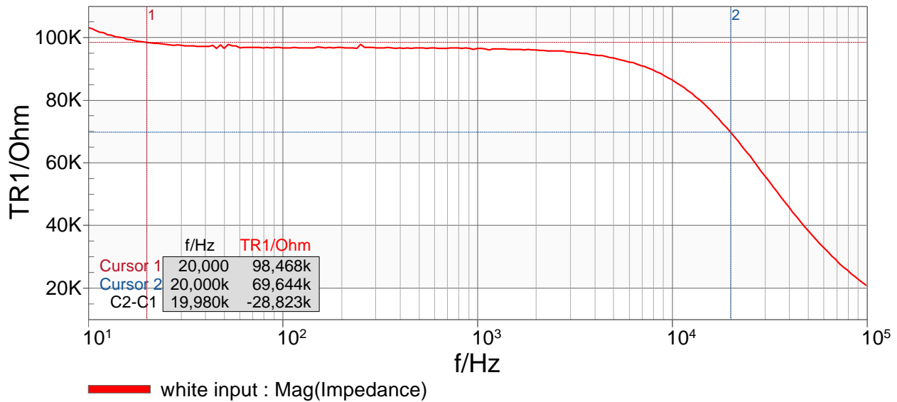
Figure 19: Input impedance with high impedance bridge - frequency sweep
