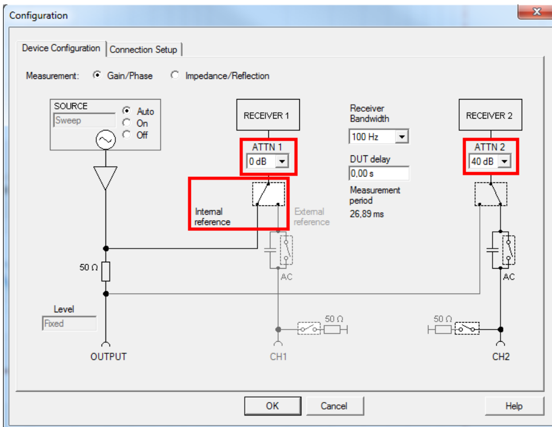
Figure 4: Gain measurement configuration window
