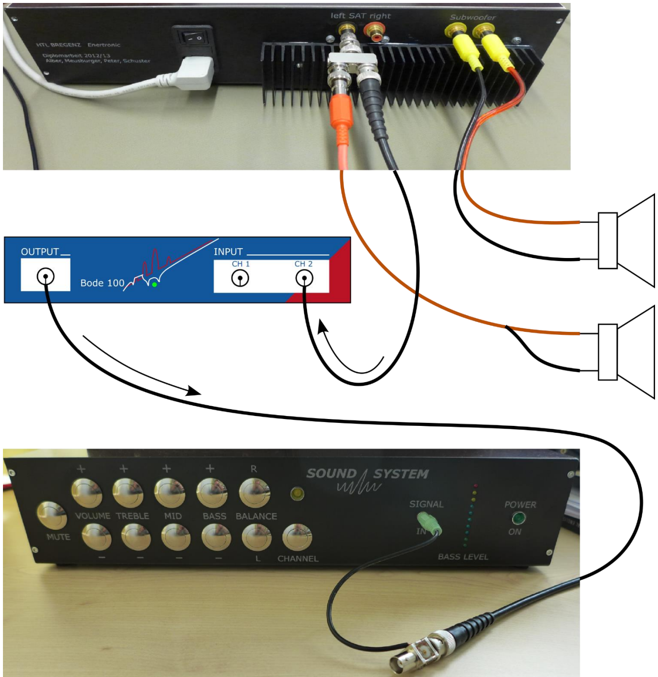
Figure 6: Gain measurement - connection setup
