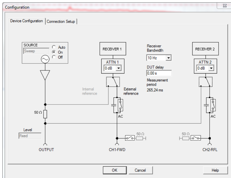
Figure 16: Input impedance with high impedance bridge – configuration window
