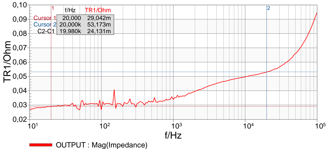
Figure 23: sound system output impedance measurement
