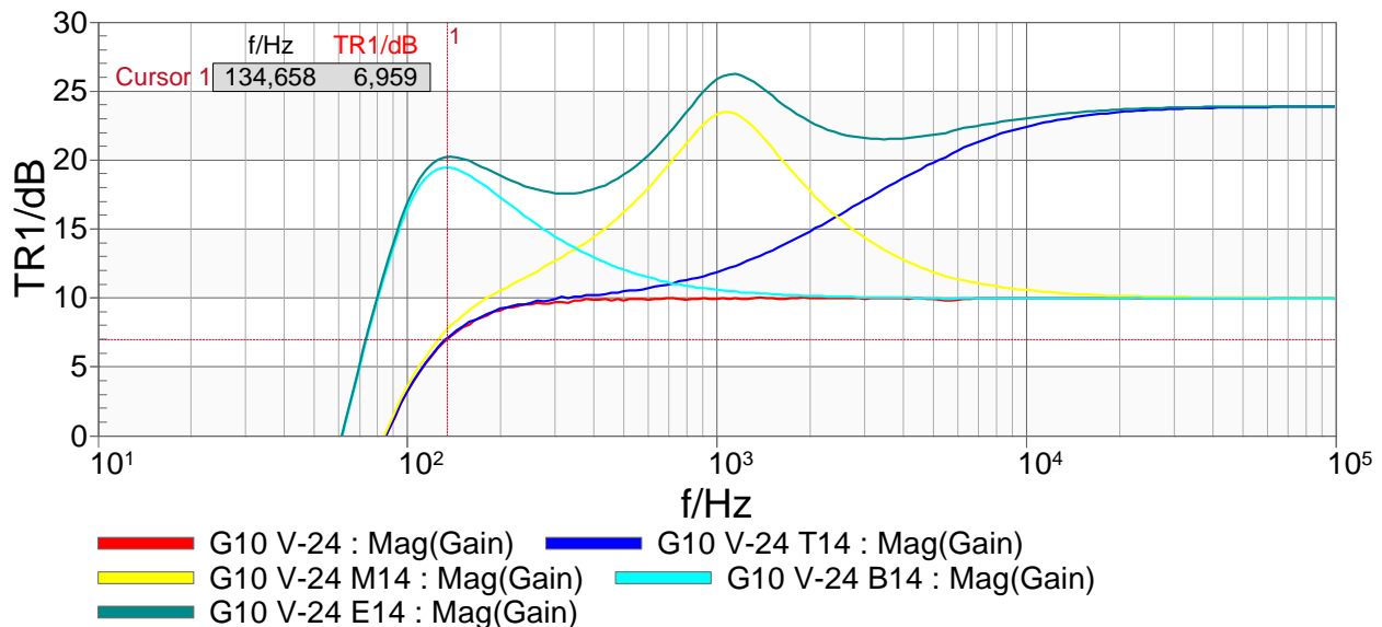
Figure 11: Gain measurement - equalizer maximum
