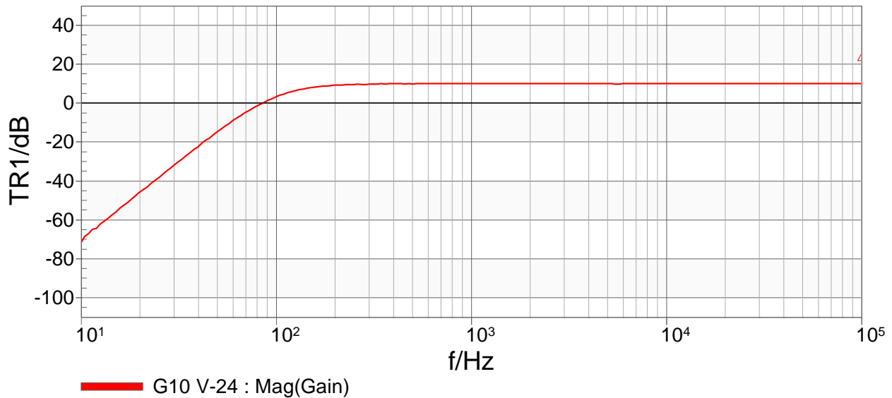
Figure 9: Gain measurement - equalizer neutral
