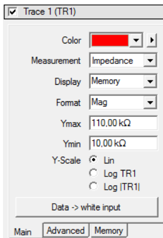
Figure 17: Input impedance with high impedance bridge - trace 1 settings
