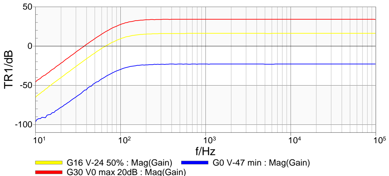
Figure 8: Gain measurement - minimum, maximum and 50 %
