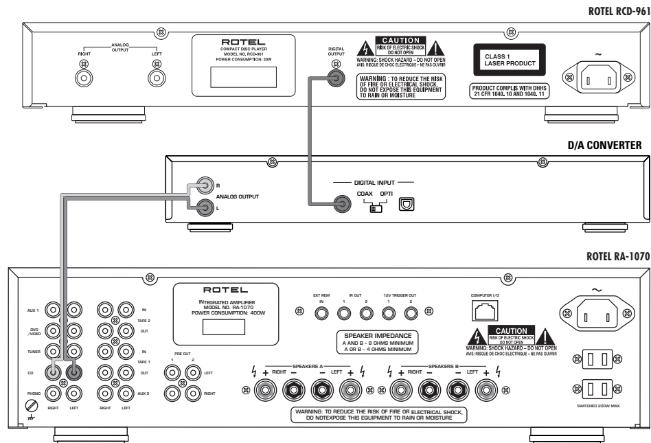
Figure 4: Digital Outputs
