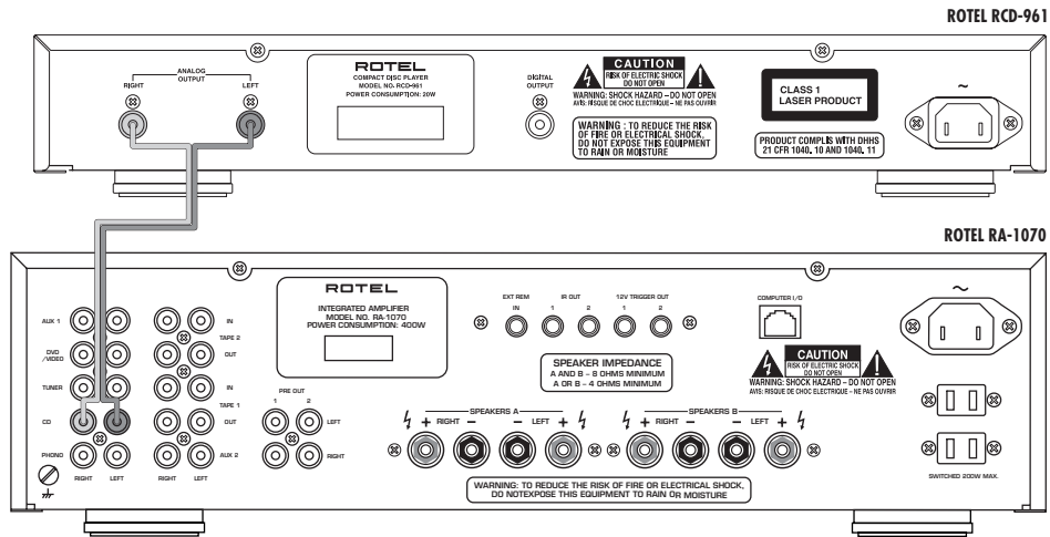
Figure 3: Analog Outputs
