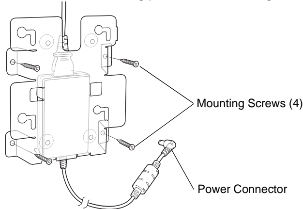
Figure 2-5 Inserting Mounting Screws
