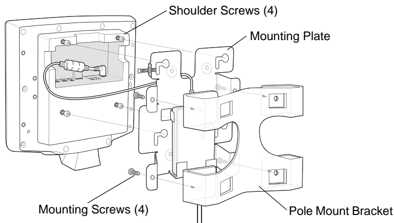
Figure 2-8 Securing Pole Mount Bracket
