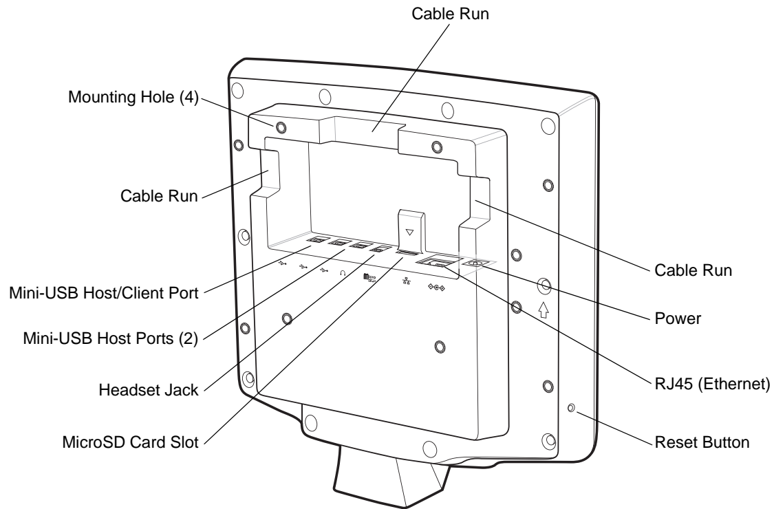
Figure 1-2 MK3100 Rear View
