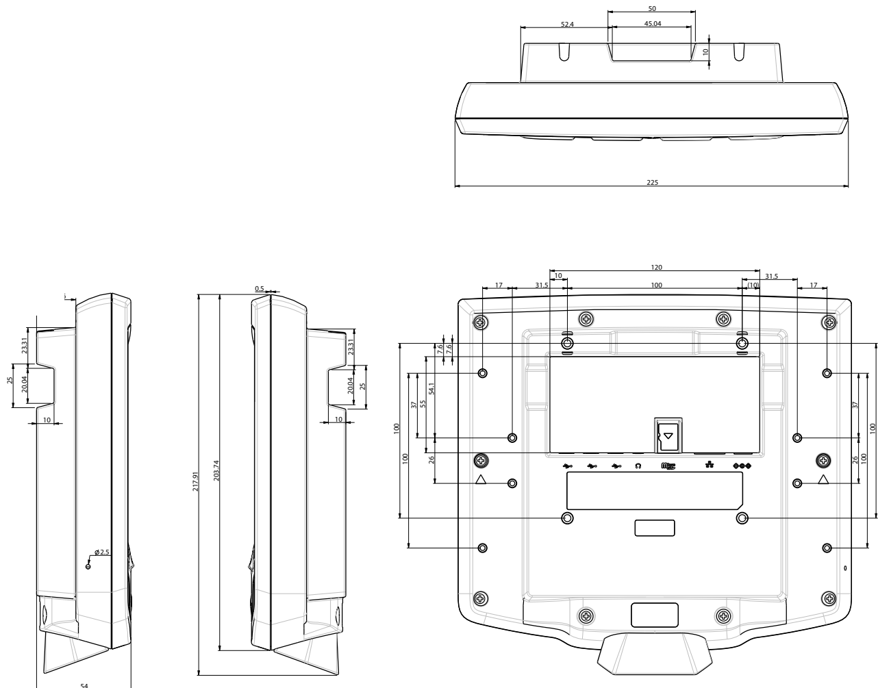
Figure 2-2 MK3100 Mounting Dimensions
