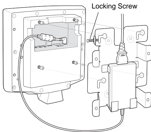
Figure 2-7 Mounting MK3100 on Mounting Plate
