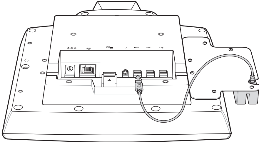
Figure 2-12 Connecting the USB Cable
