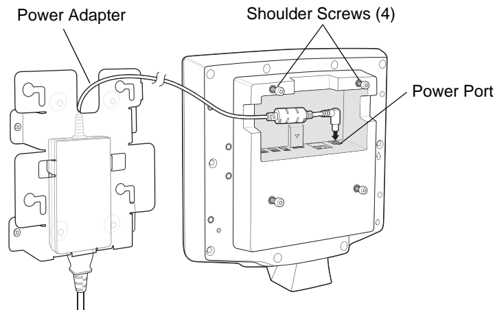
Figure 2-6 Inserting Shoulder Screws
