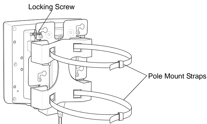
Figure 2-9 Inserting Locking Screw
