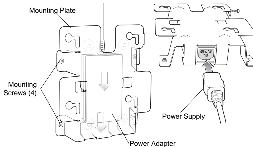
Figure 2-3 Securing the Mounting Plate - Configuration 1
