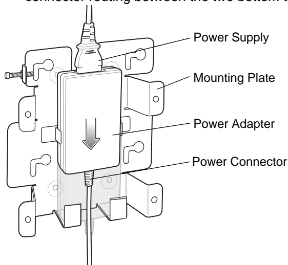
Figure 2-4 Securing the Mounting Plate - Configuration 2
