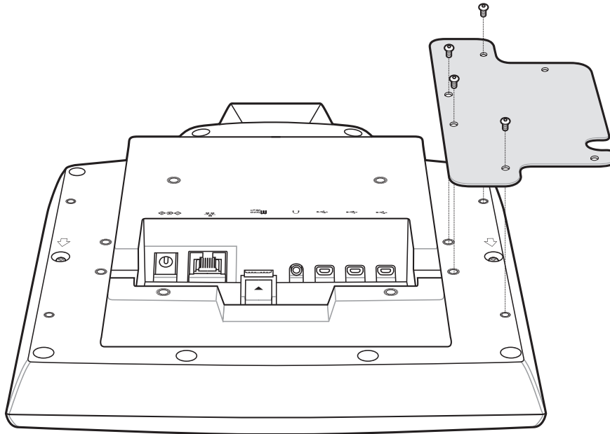
Figure 2-10 Securing the MSR Mounting Plate
