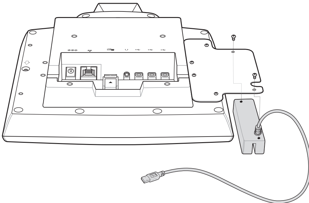
Figure 2-11 Securing the MSR to the Mounting Plate
