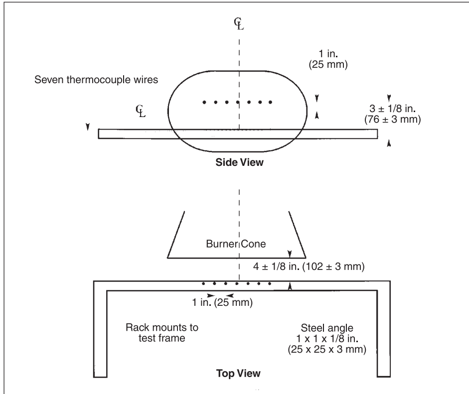
FIGURE 5 Thermocouple Rake Position Relative to Burner Cone
