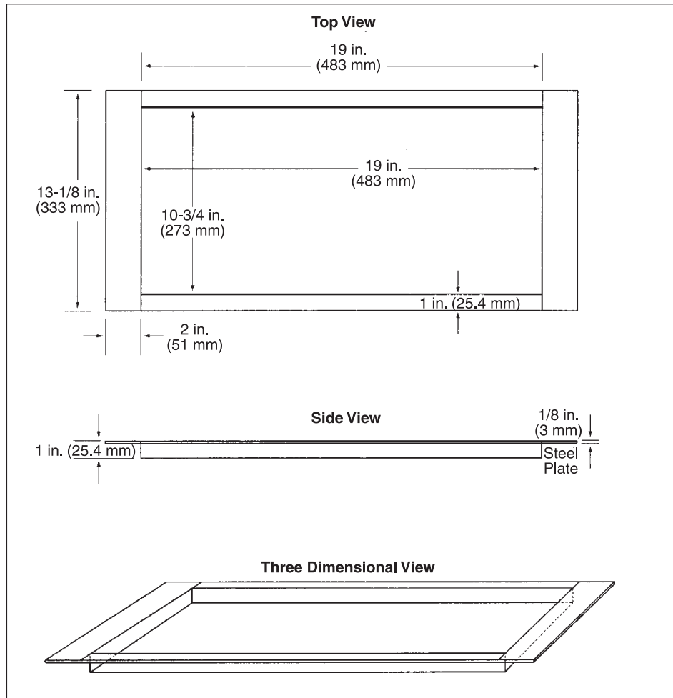
FIGURE 5 3 Views
