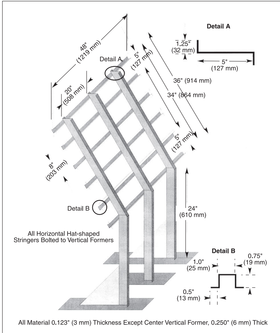
FIGURE 1 Burnthrough Test Apparatus Specimen Holder
