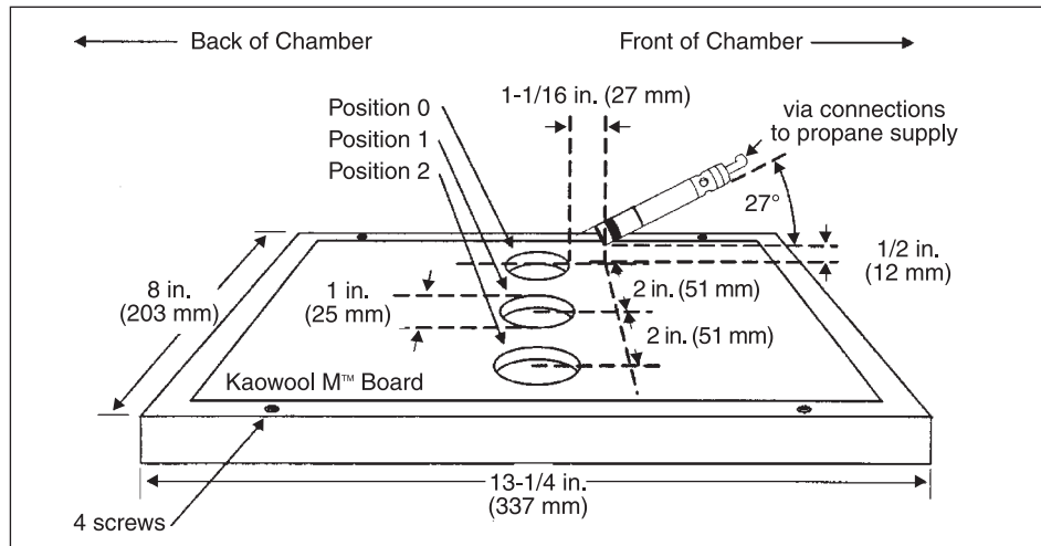
FIGURE 7 Calorimeter Holding Frame
