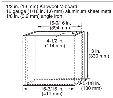
FIGURE 2 Internal Chimney
