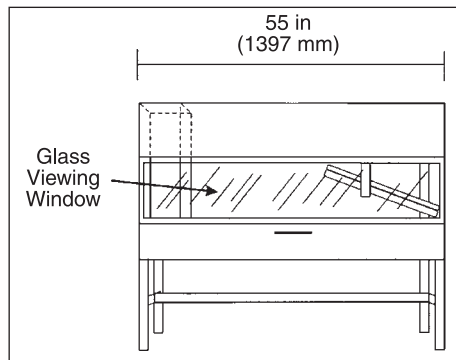
FIGURE 1 Radiant Panel Test Chamber
