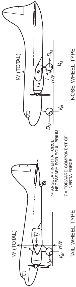
FIGURE 2—Level landing.
