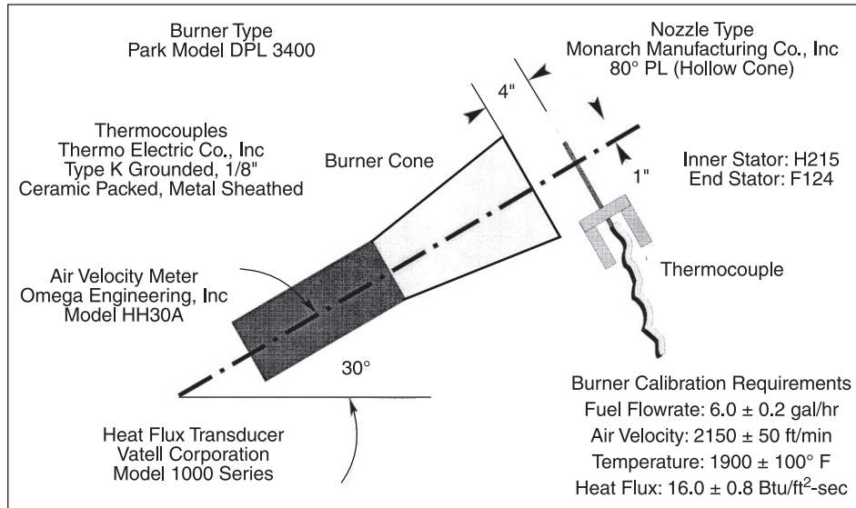
FIGURE 8 Burner Information and Calibration Settings
