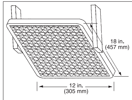
FIGURE 3b Air Propane Radiant Panel
