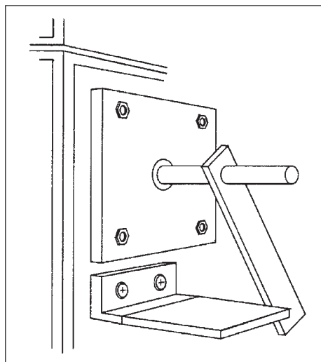
FIGURE 8 Propane Burner Stop
