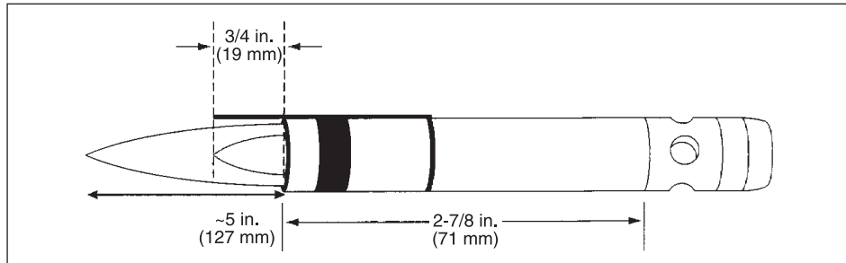
FIGURE 6 Propane Pilot Burner
