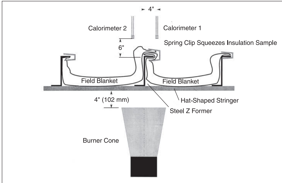
FIGURE 7 Test Specimen Installation on Test Frame
