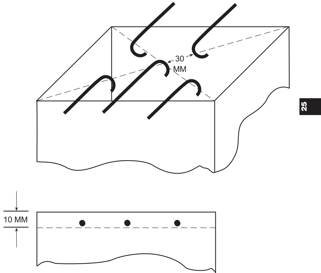
Figure 5. Thermocouple Position
