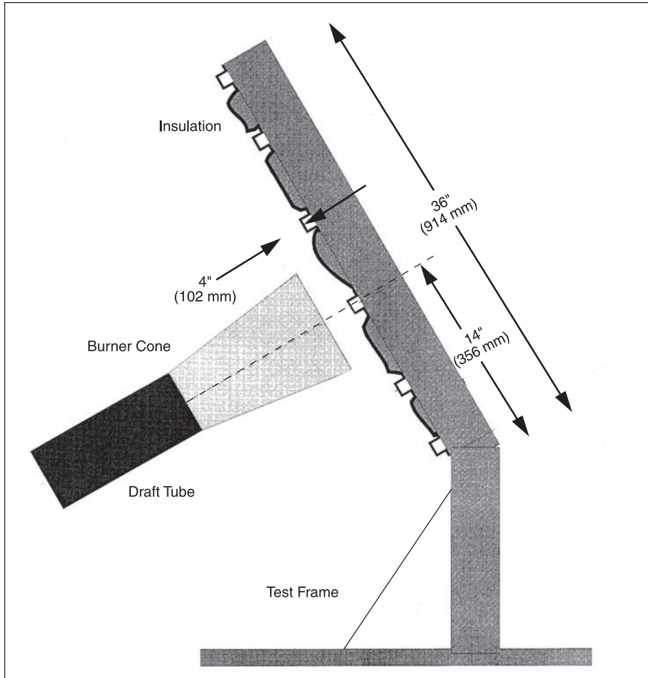
FIGURE 2 Burnthrough Test Apparatus
