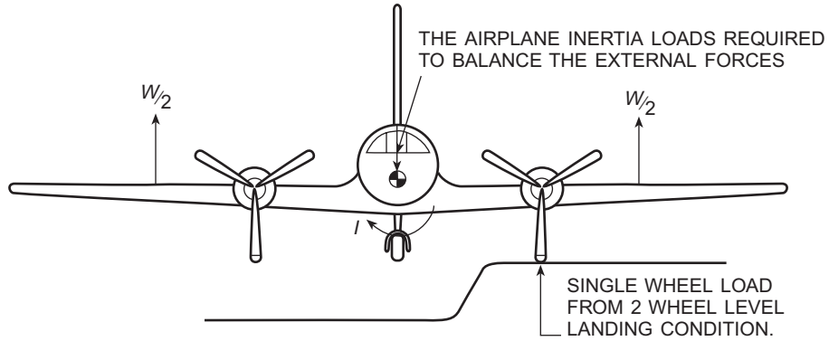
NOSE OR TAIL WHEEL TYPE
