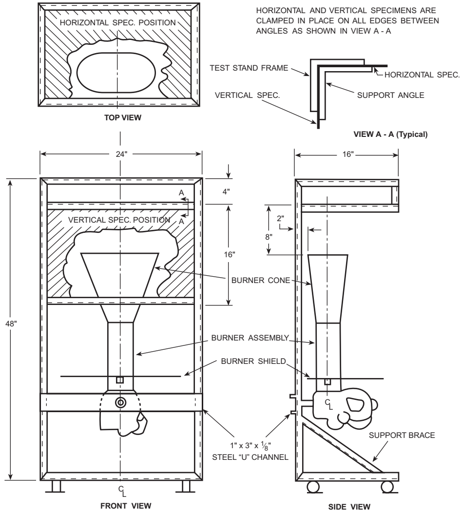
FIGURE 1. Test apparatus for horizontal and vertical mounting.
