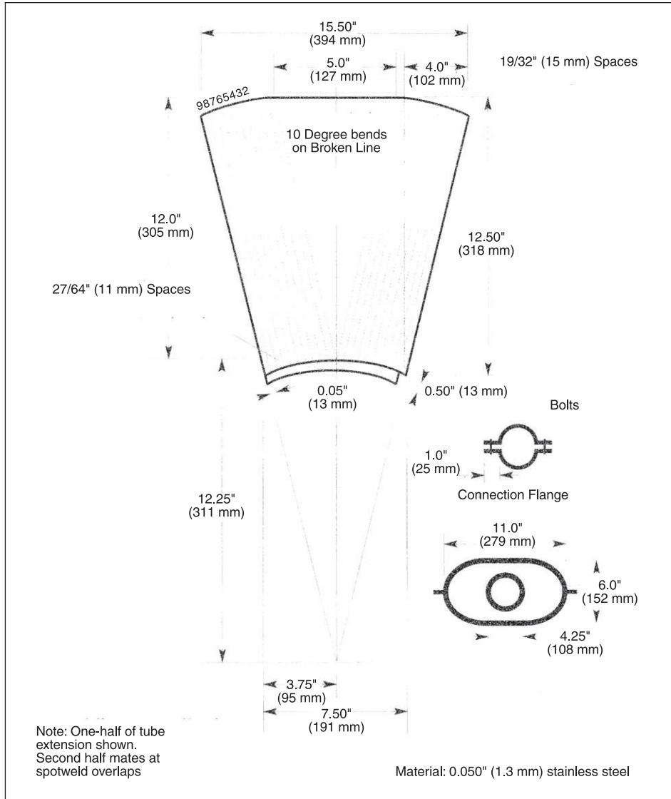
FIGURE 3 Burner Draft Tube Extension Cone Diagram
