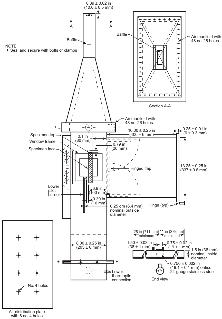
Figure 1B Rate of Heat Release Apparatus
