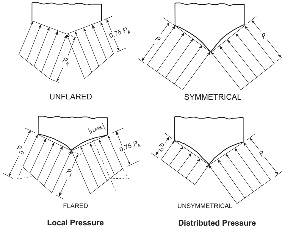
FIGURE 3 — Transverse pressure distributions.
