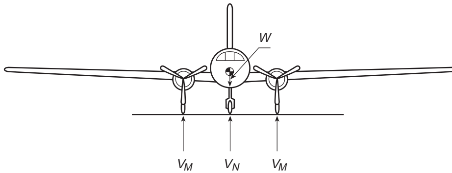
FIGURE 8—Pivoting, nose or tail wheel type.
