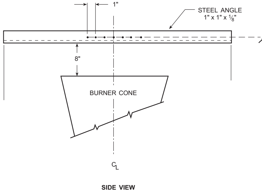
FIGURE 3. Thermocouple rake bracket
