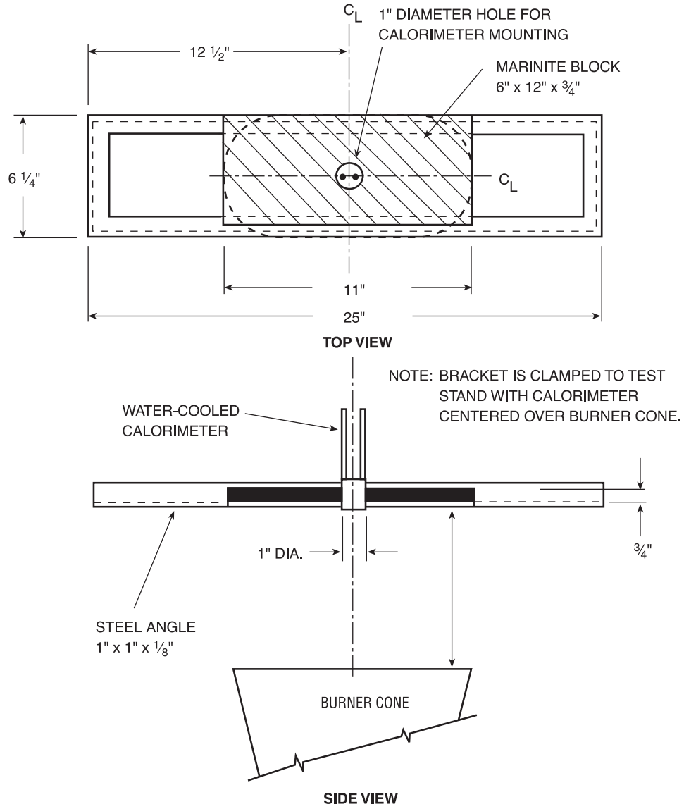
FIGURE 2. Calorimeter bracket
