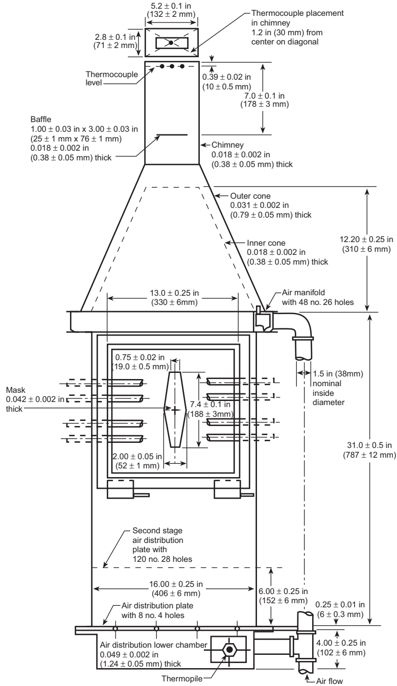
Figure 1A Rate of Heat Release Apparatus
