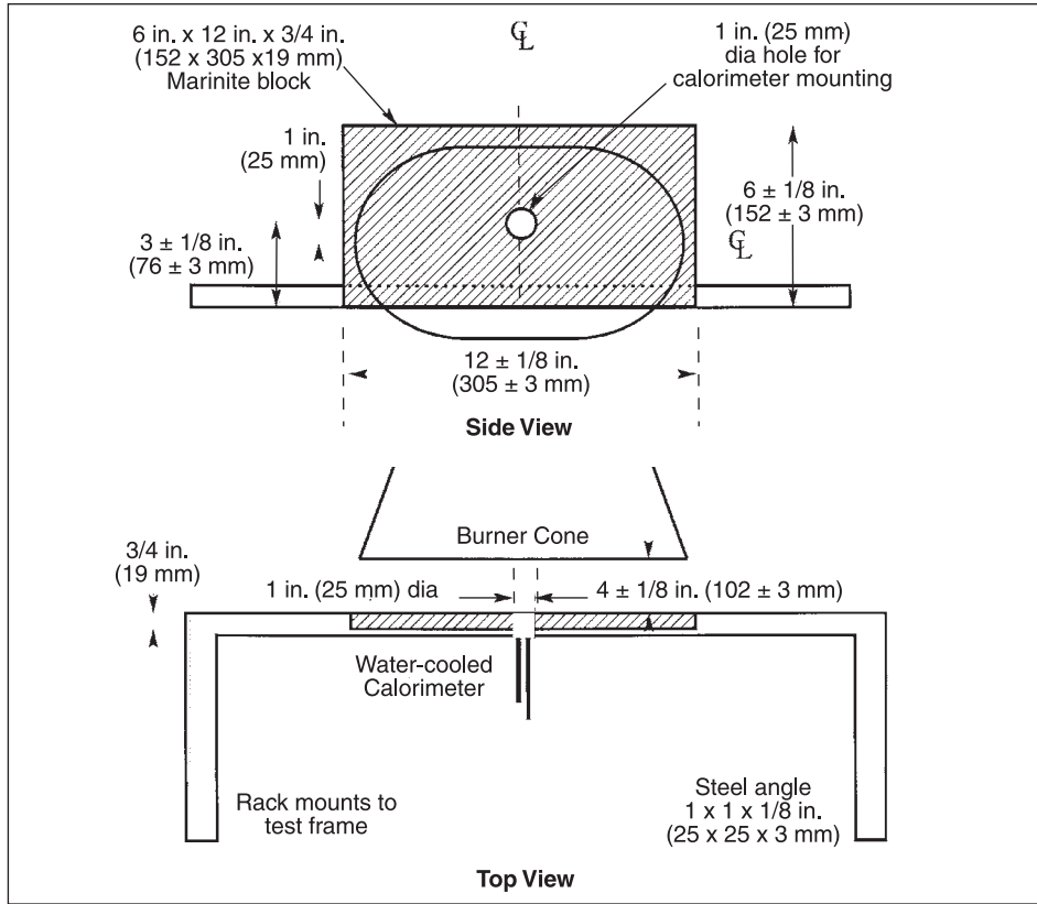
FIGURE 4 Calorimeter Position Relative to Burner Cone
