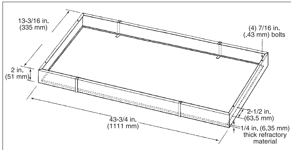
FIGURE 4 Sliding Platform
