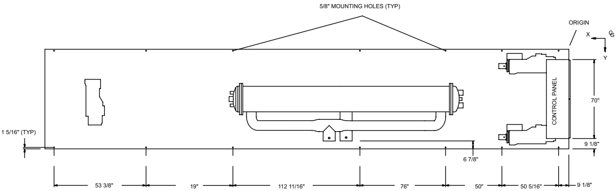
VIEW D-D
