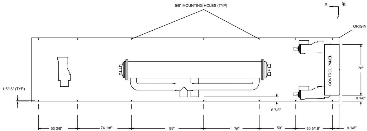
VIEW D-D
