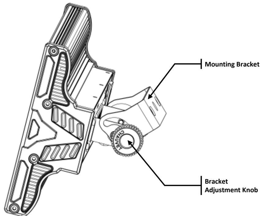
Mounting Diagram
