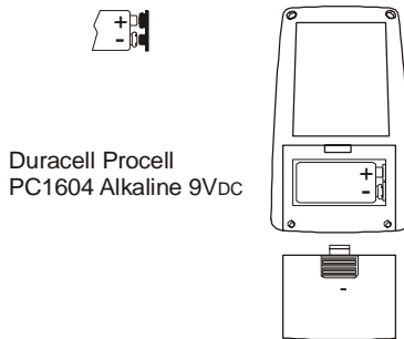
Figure 1 - Battery Replacement
